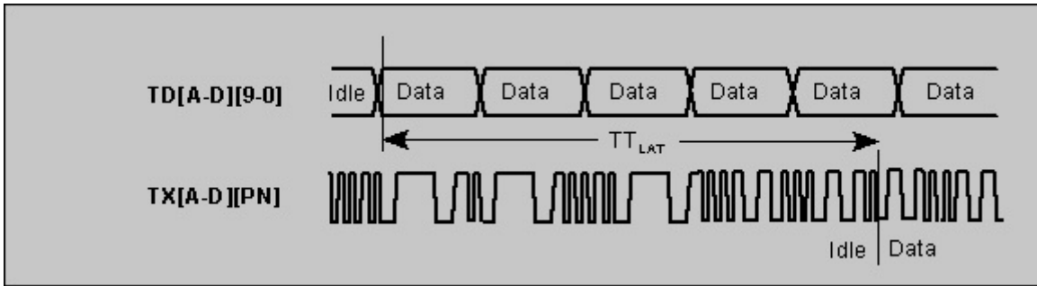
FIGURE 6-2. TRANSMITTER LATENCY
