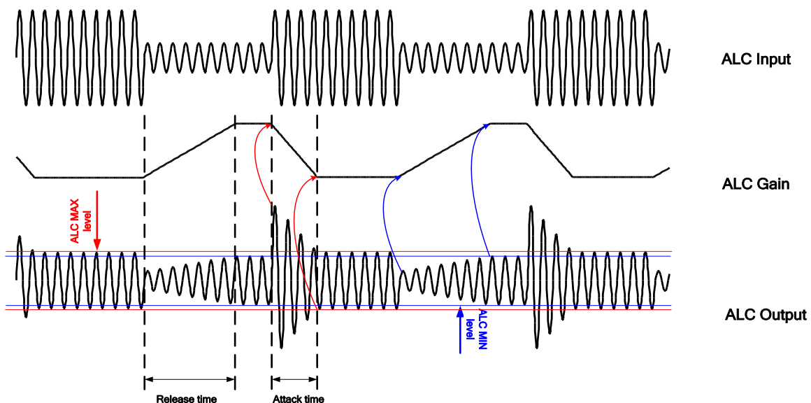
Figure 11. Principle of operation of the ALC
