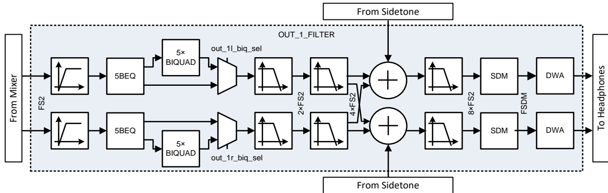
Figure 15. Output filters block diagram
