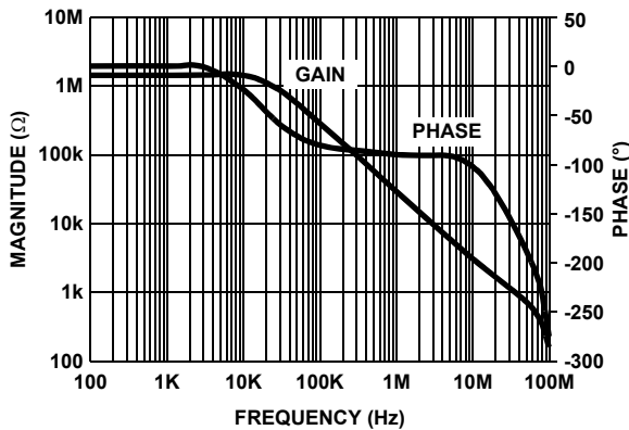
FIGURE 51. TRANSIMPEDANCE (ROL) vs FREQUENCY
