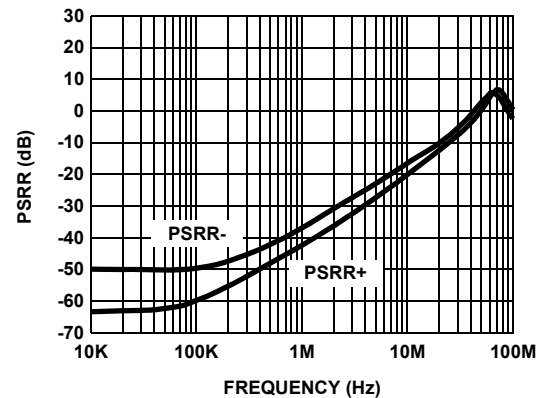
FIGURE 48. POWER SUPPLY REJECTION vs FREQUENCY
