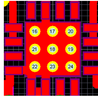
TOP (16 Ld QFN)
