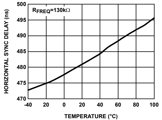
FIGURE 28. HORIZONTAL DELAY vs TEMPERATURE
