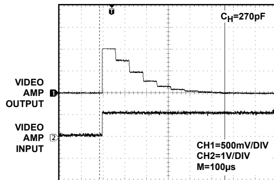
Auto-zero mechanism restores amplifier output to 1.3V after +1V step at input
