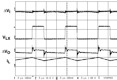
Steady State Operation (inductor continuous conduction) VIN=5V, VO=12V, IO=300mA
