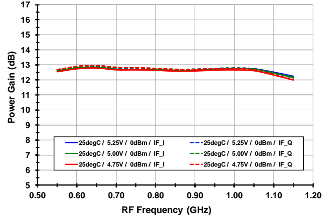
GAIN vs. V_{CC} [ High Side Injection ]
