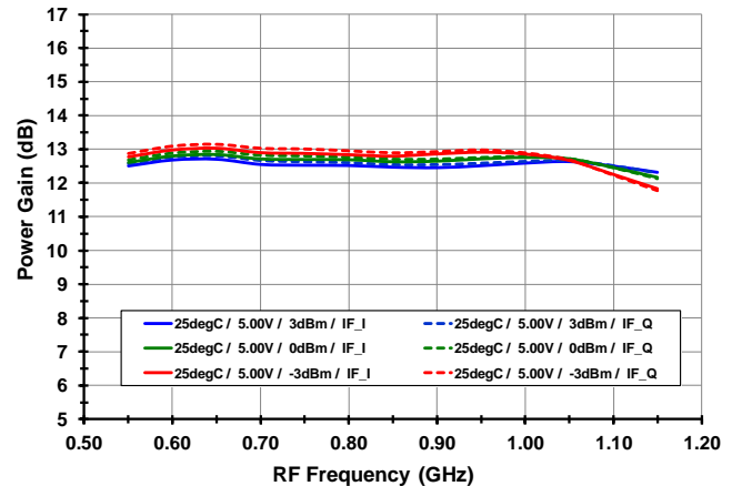
GAIN vs. LO level [ High Side Injection ]
