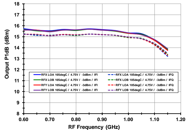
OP1dB [High Side Injection]
