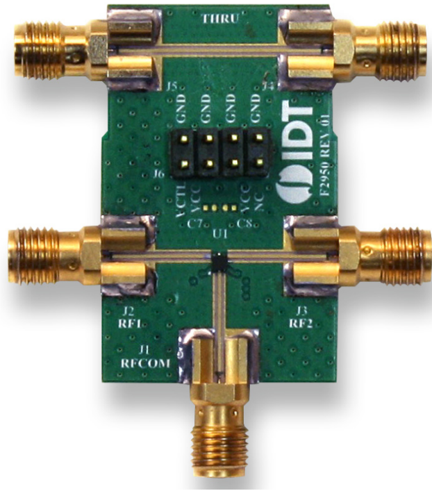
Figure 18. Top View
