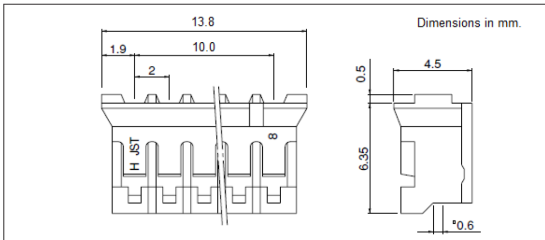
Figure 7. Receptacle Drawing
