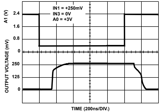
FIGURE 4. CHANNEL-TO-CROSSING RESPONSE
