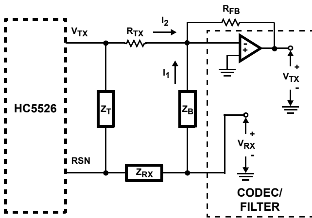
FIGURE 17. TRANSHYBRID CIRCUIT
