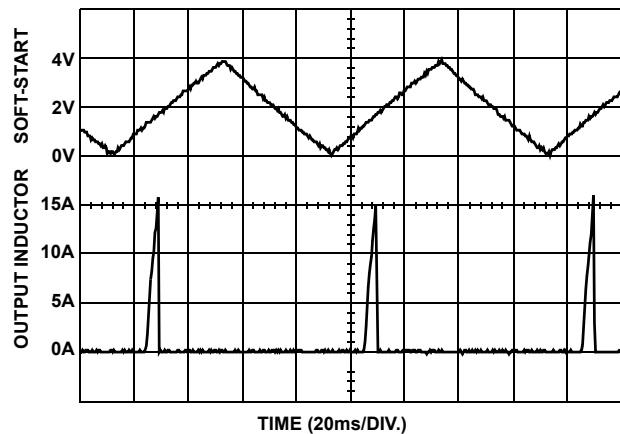
FIGURE 4. OVER-CURRENT OPERATION
