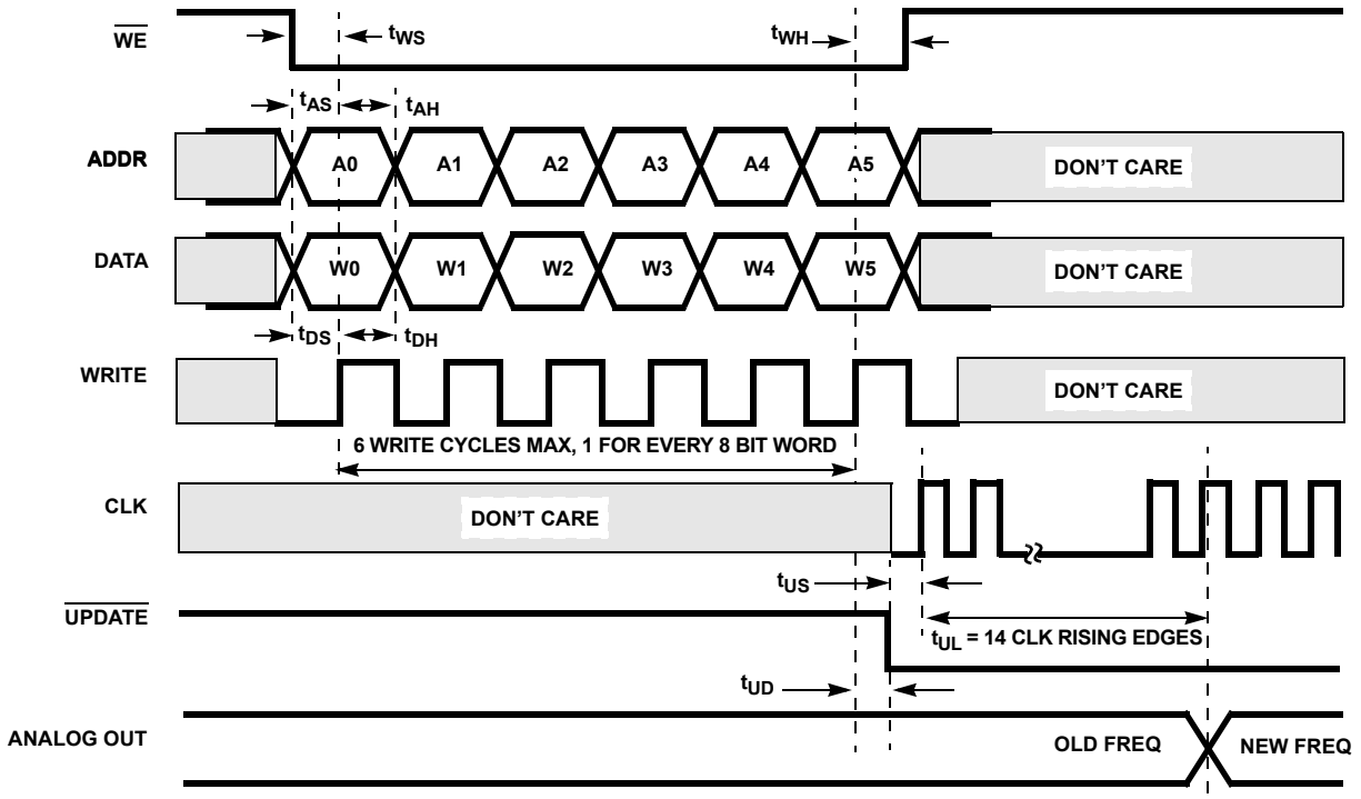
FIGURE 2. PARALLEL-LOAD METHOD 1, UPDATE ACTIVE AFTER LOADING REGISTERS ( \overline{RESET} = \text{HIGH} )
