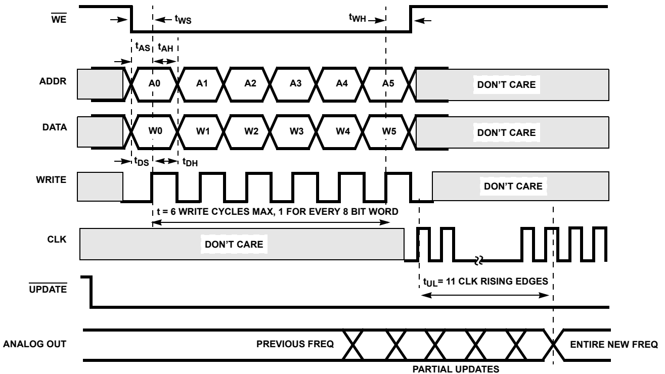
FIGURE 3. PARALLEL-LOAD METHOD 2, UPDATE ACTIVE WHILE LOADING REGISTERS ( \overline{RESET} = \text{HIGH} )
