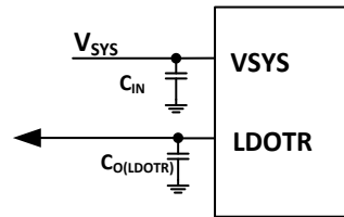
Figure 30. LDO3, 4 External component connections
