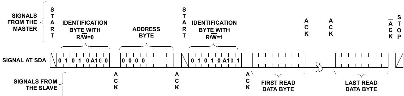
FIGURE 24. READ SEQUENCE
