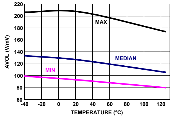
FIGURE 30. AVOL vs TEMPERATURE, V_+, V_- = \pm 2.5V, V_O = -2V \text{ TO } +2V, R_L = 1k
