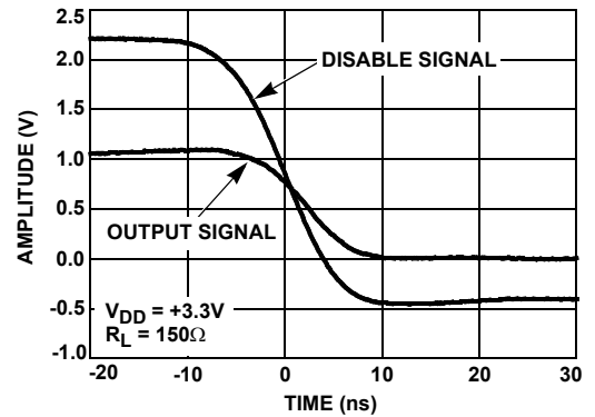
FIGURE 14. DISABLE TIME
