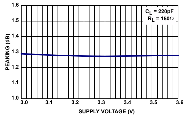
FIGURE 5. PEAKING vs SUPPLY VOLTAGE ( C_L = 220pF )
