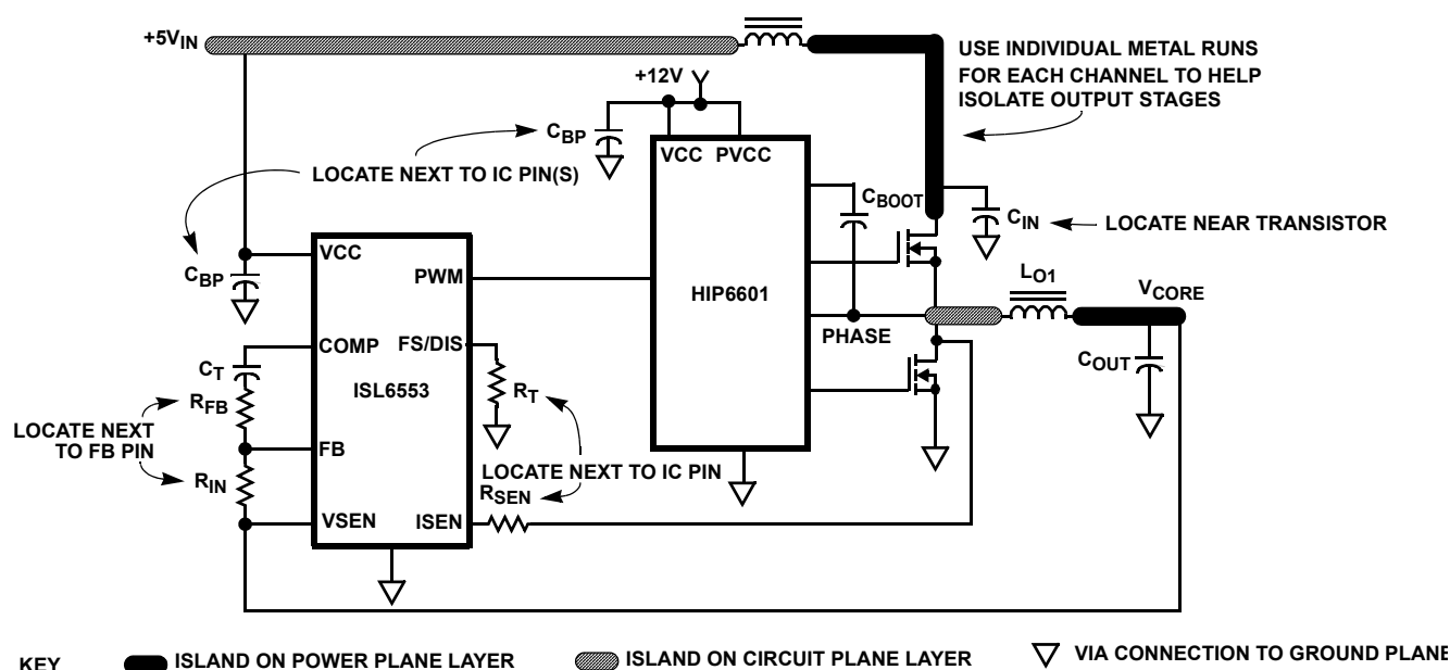
FIGURE 11. PRINTED CIRCUIT BOARD POWER PLANES AND ISLANDS
