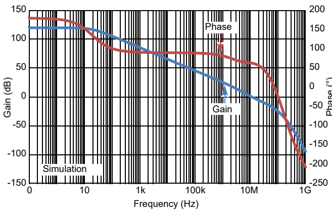
Figure 30. Open-Loop Frequency Response ( C_L = 0.01pF )
