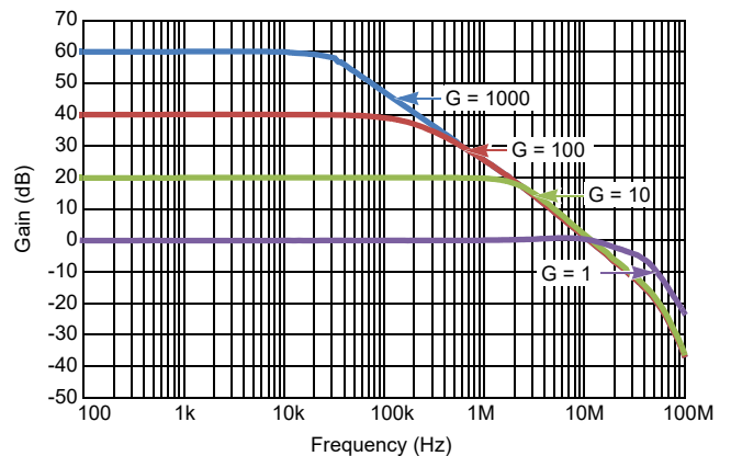
Figure 39. Frequency Response vs Closed-Loop Gain
