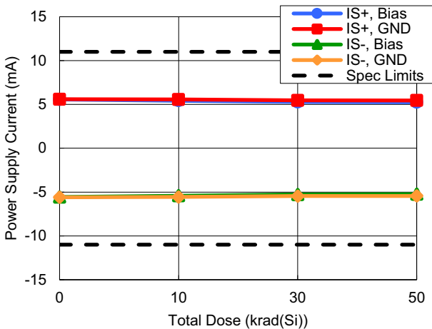
Figure 57. Operating Supply Current vs TID V_S = \pm 18V
