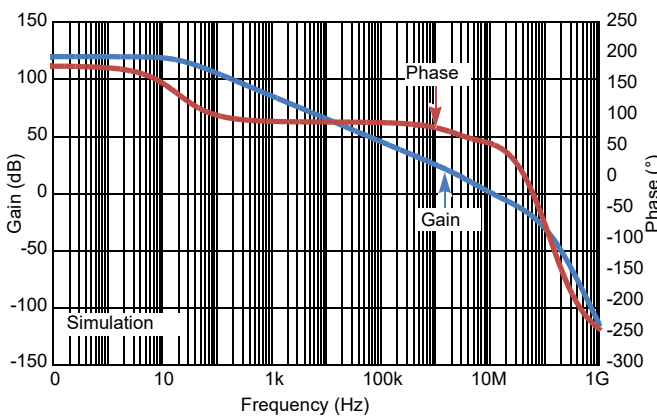
Figure 32. Open-Loop Frequency Response ( C_L = 22pF )
