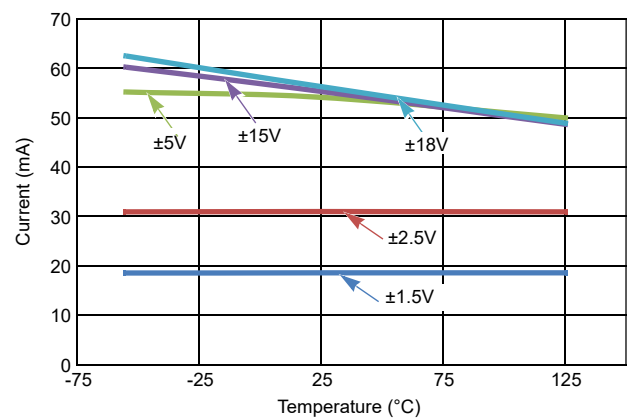
Figure 21. Short-Circuit Current vs Temperature
