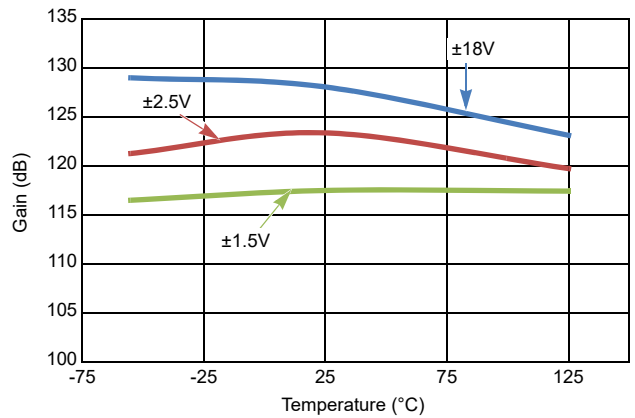
Figure 19. PSRR- vs Temperature vs Supply Voltage
