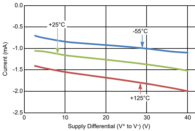
Figure 16. Negative Supply Current vs Supply Voltage
