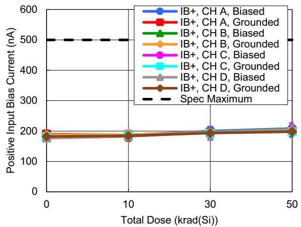
Figure 58. Positive Input Bias Current vs TID ( V_S = \pm 18V )
