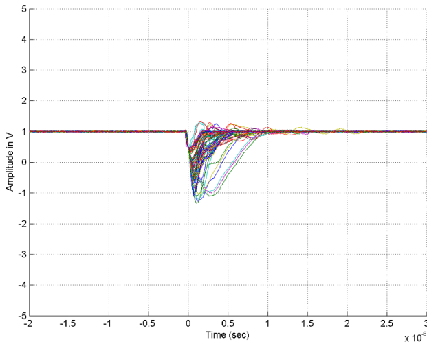
Figure 62. SET Response with V_S = \pm 1.35V
