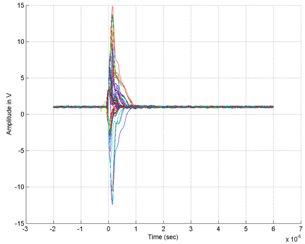
Figure 63. SET Response with V_S = \pm 15.0V
