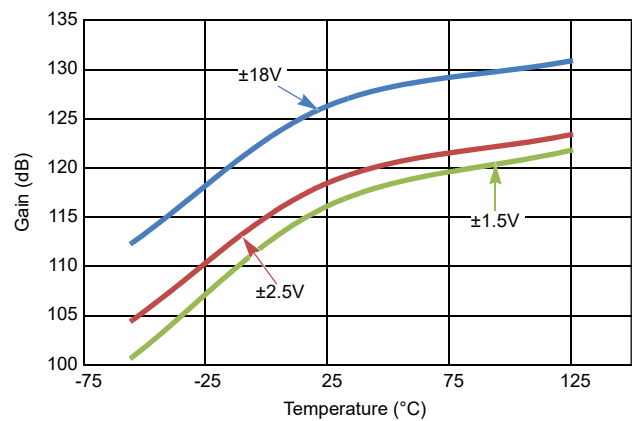
Figure 15. A_{VOL} vs Temperature vs Supply Voltage
