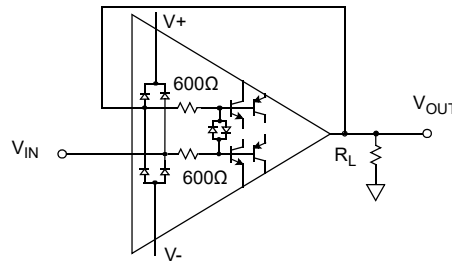
Figure 53. Input ESD Diode Current Limiting, Unity Gain
