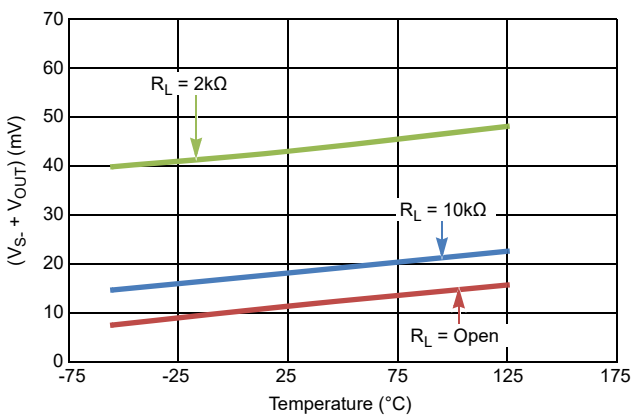
Figure 26. ( V_S = \pm 2.5V ) V_{OL} vs Temperature
