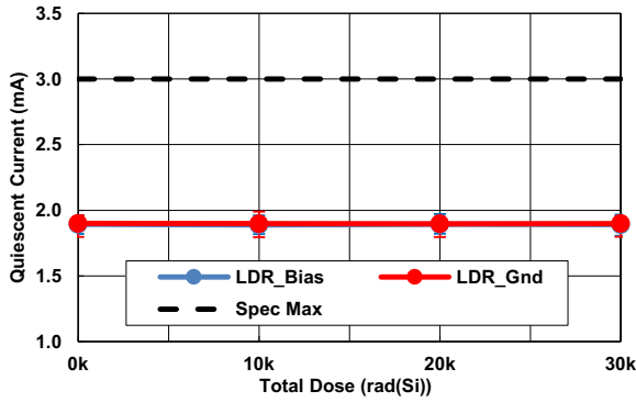
Figure 25. 5V Quiescent Supply Current vs TID
