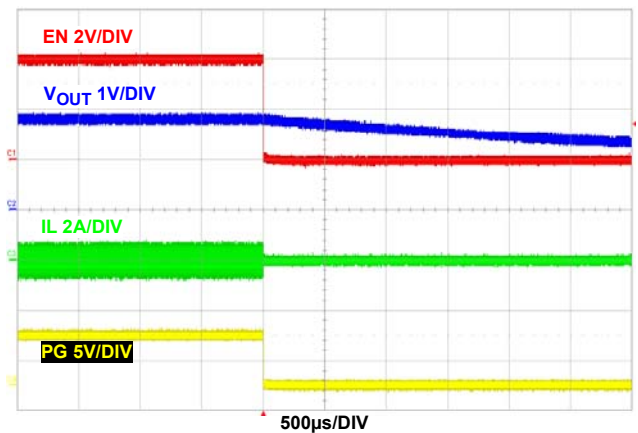
FIGURE 25. SOFT-DISCHARGE SHUTDOWN
