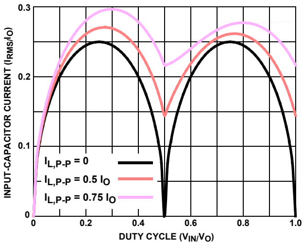
FIGURE 25. NORMALIZED INPUT-CAPACITOR RMS CURRENT FOR 2-PHASE CONVERTER
