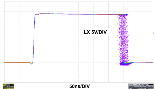
FIGURE 28. JITTER AT 800mA LOAD, PWM
