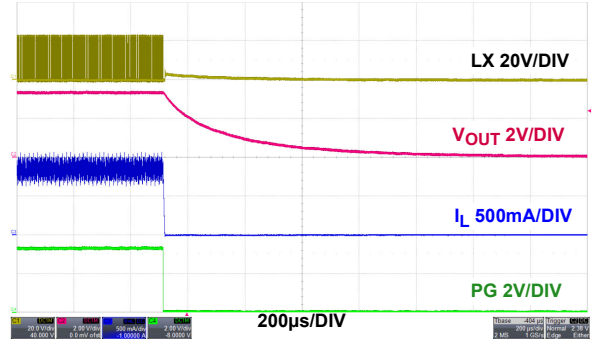
FIGURE 26. SHUTDOWN AT 800mA, PFM
