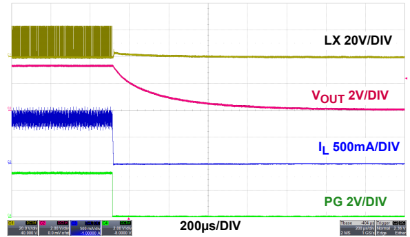
FIGURE 24. SHUTDOWN AT 800mA, PWM
