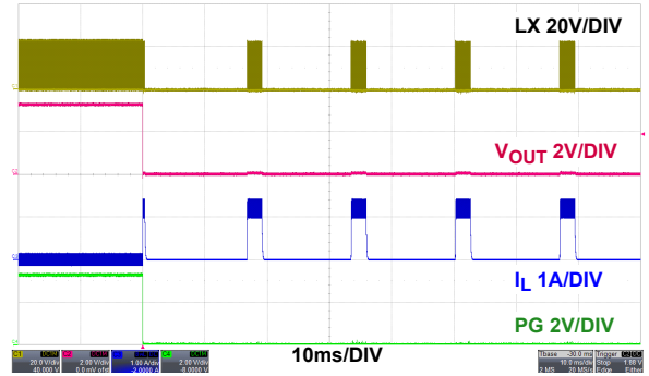
FIGURE 38. OVERCURRENT PROTECTION HICCUP, PWM
