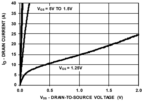
FIGURE 3. OUTPUT CHARACTERISTICS
