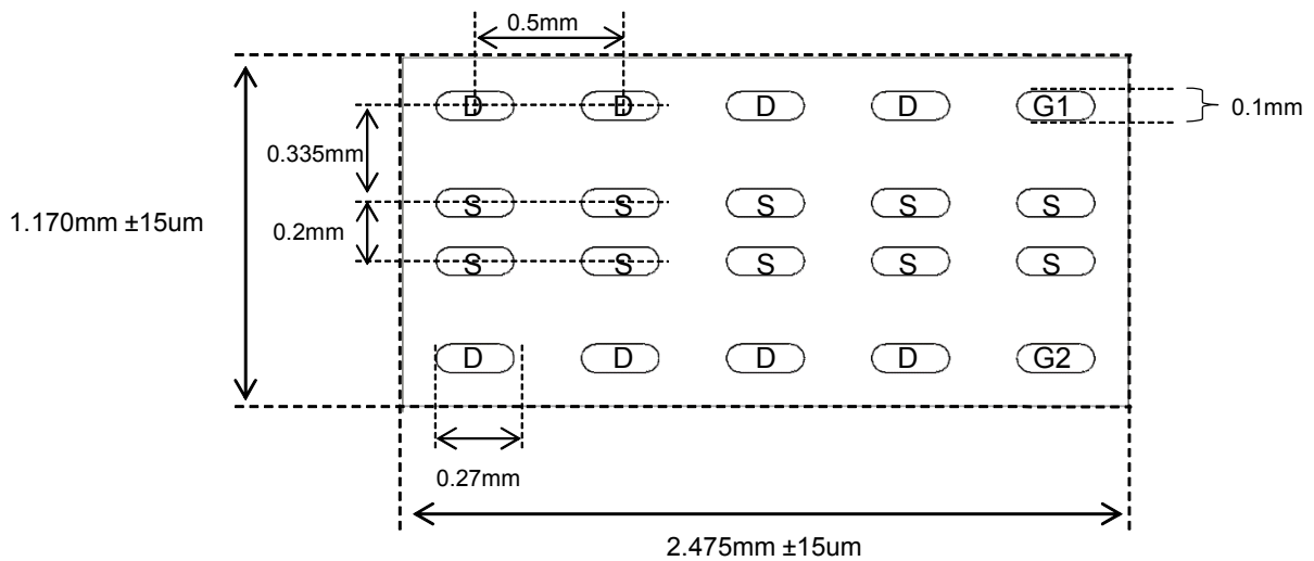
Pad-up View
