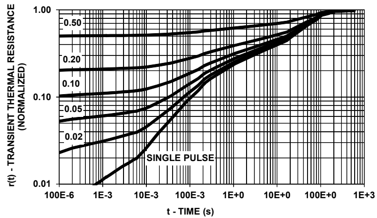
FIGURE 14. TRANSIENT THERMAL RESPONSE, JUNCTION-TO-AMBIENT (IN PARALLEL)
