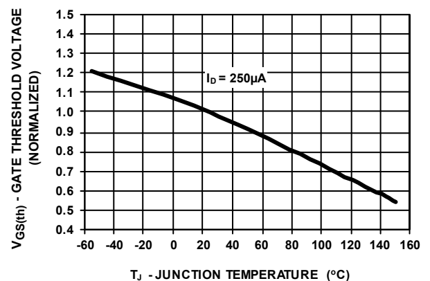
FIGURE 8. GATE THRESHOLD VOLTAGE vs JUNCTION TEMPERATURE
