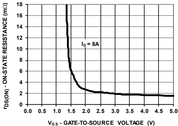
FIGURE 7. DRAIN-TO-SOURCE ON-STATE RESISTANCE vs GATE-TO-SOURCE VOLTAGE
