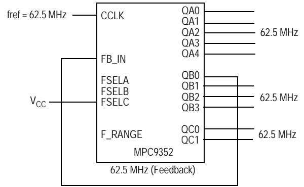
MPC9352 zero-delay (feedback of QB0 = 62.5 MHz). All control pins are left open except FSEL = 1. All outputs are locked in frequency and phase to the input clock.
