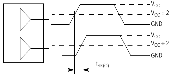
Figure 17. Output-to-Output Skew t_{sk(O)}
