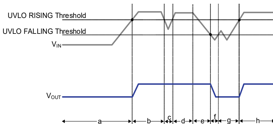
Figure 43. UVLO Operation
