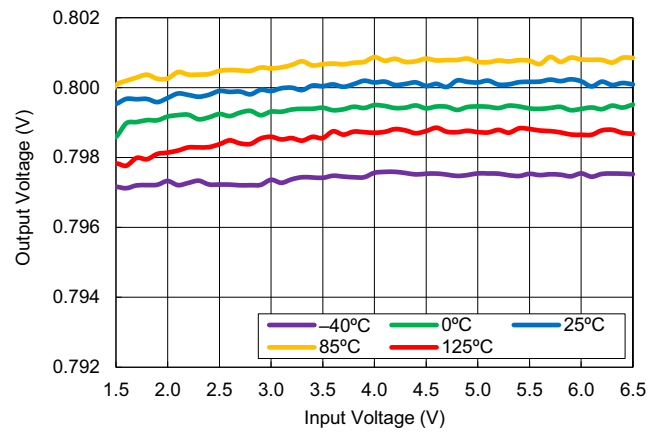
Figure 35. Line Regulation vs Input Voltage ( V_{OUT} = 0.8\text{V} , I_{OUT} = 5\text{mA} )
