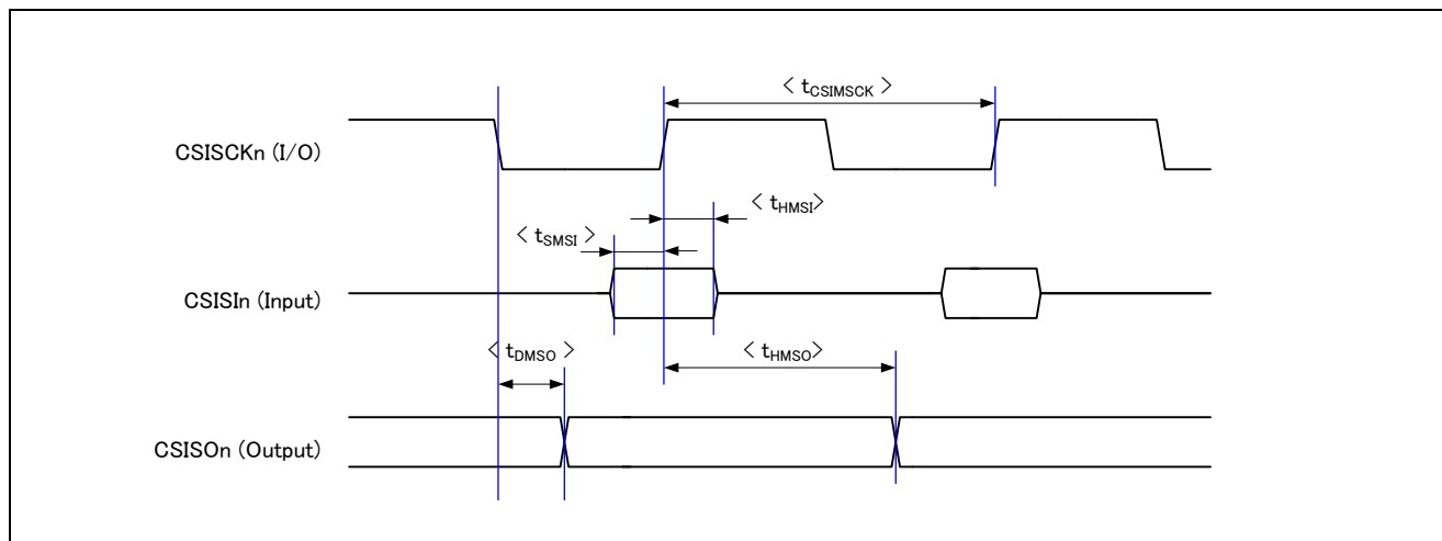
Figure 4.20 CSI Access Timing Diagram (Master Mode)
