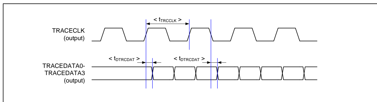
Figure 4.31 Trace Interface
