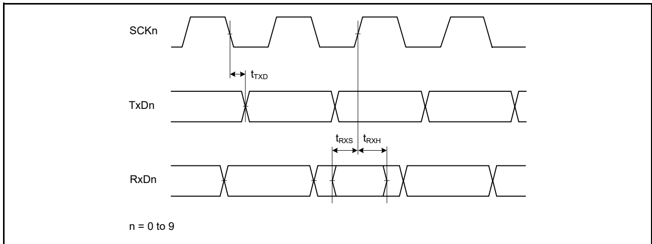
Figure 2.41 SCI input/output timing in clock synchronous mode
