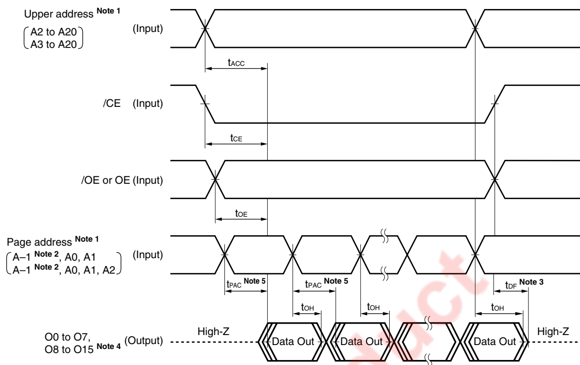
Read Cycle Timing Chart 2 (Page Access Mode)
