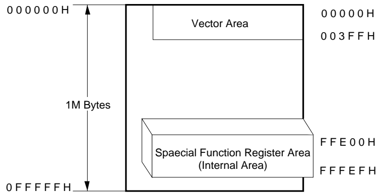
Figure 3-3. Basic Memory Space
