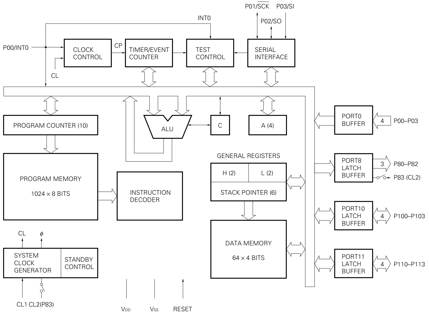
BLOCK DIAGRAM OF \mu\text{PD7554A}
