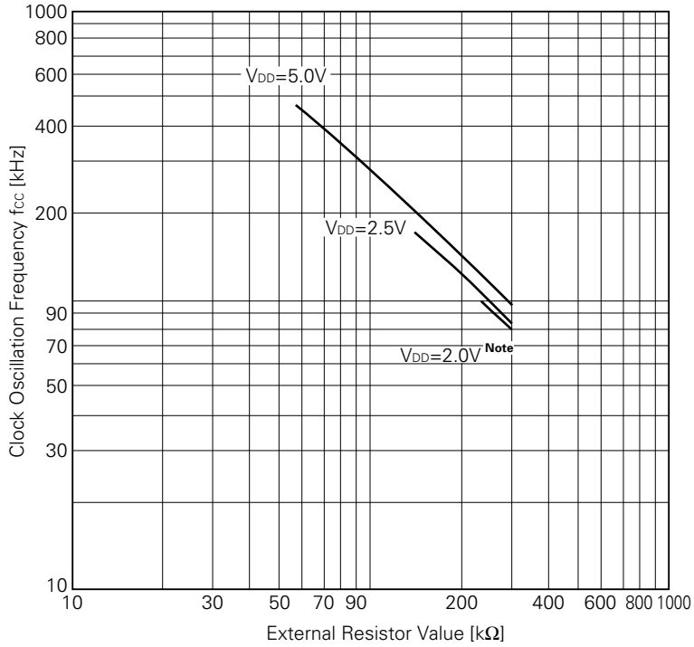
f cc vs. R Characteristics Example (Reference Value) (T a =25°C)
