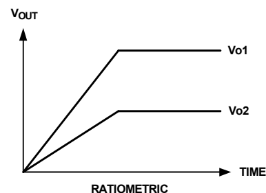
FIGURE 9. TRACKING MODES
