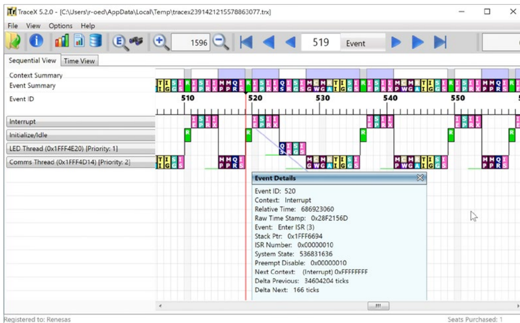
Figure 11-5: The sequence of events as visualized by TraceX®
