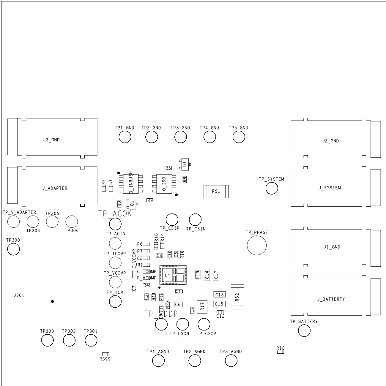
FIGURE 20. BOTTOM SILK SCREEN (VIEWED FROM THE BOTTOM)
