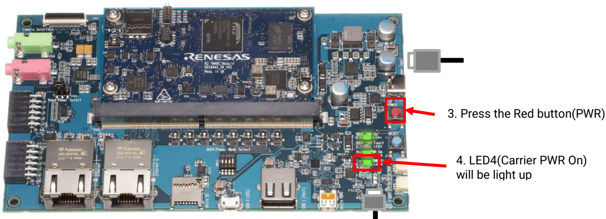
Figure 5. Power ON
