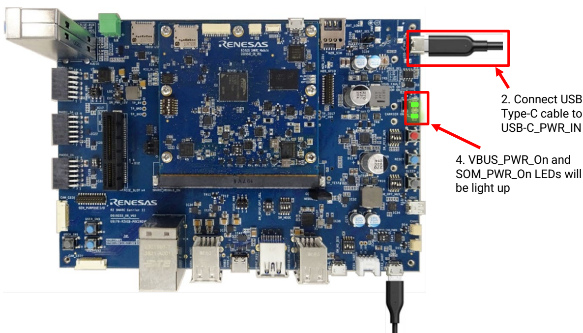
Figure 11. Connecting Power Supply
