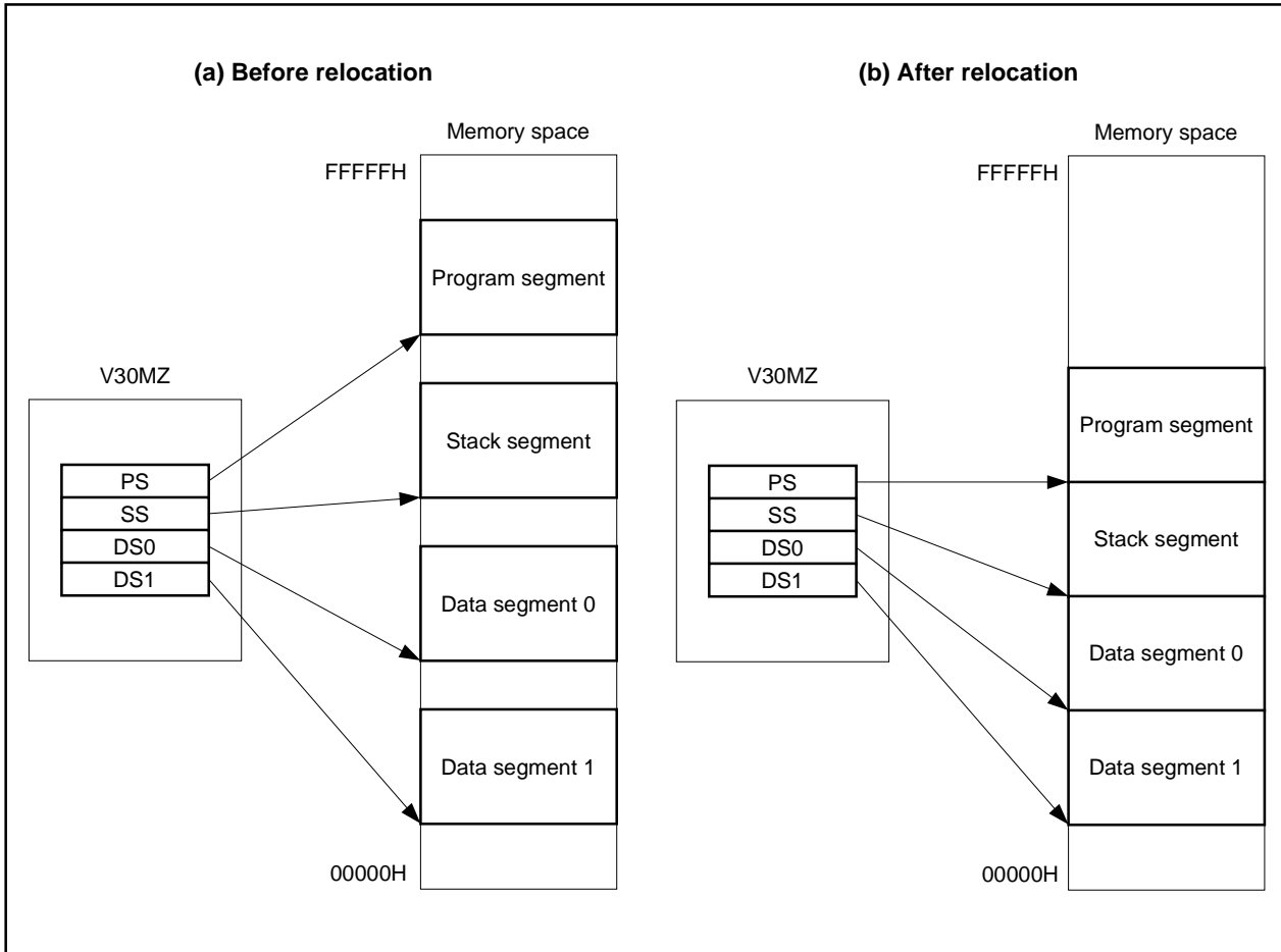
Figure 3-8. Dynamic Relocation
