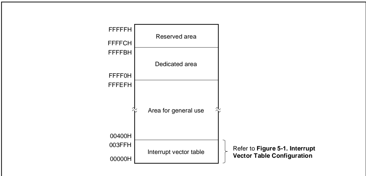
Figure 3-2. Memory Map
