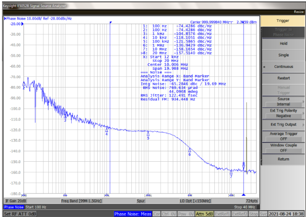
Figure 8. Phase Noise Plot of 1000MHz Output from 8V97003 #1 ROUT_A/nROUT_A
