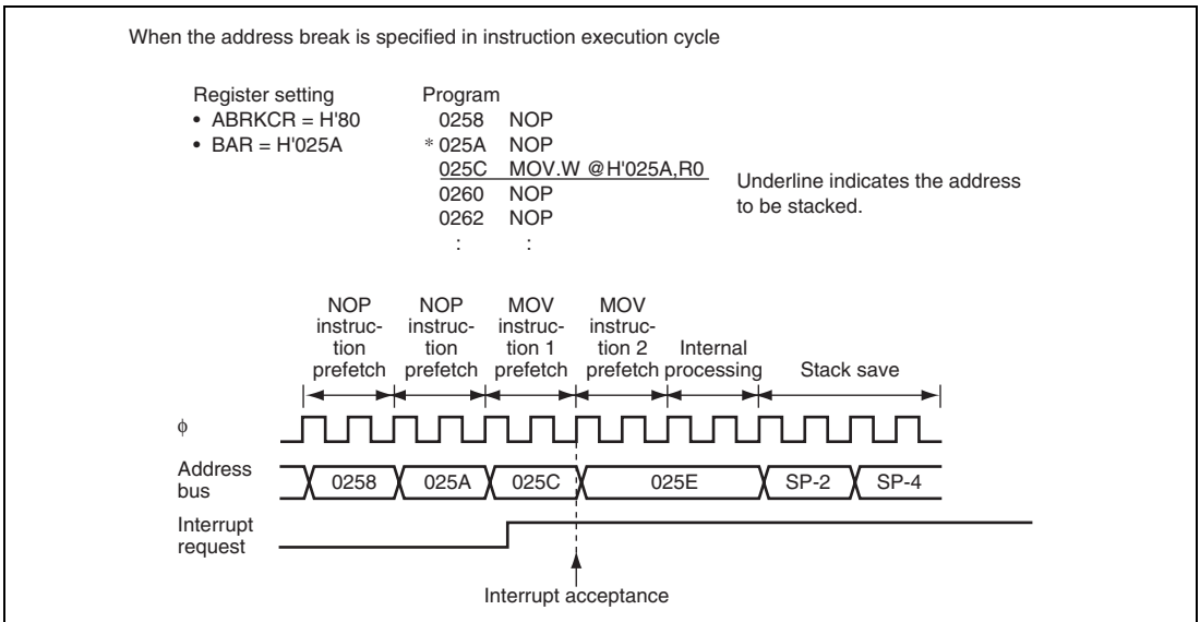
Figure 4.2 Address Break Interrupt Operation Example (1)
