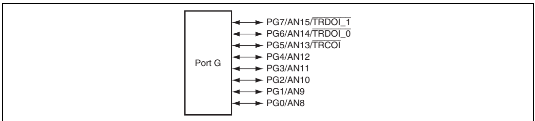
Figure 9.11 Port G Pin Configuration
