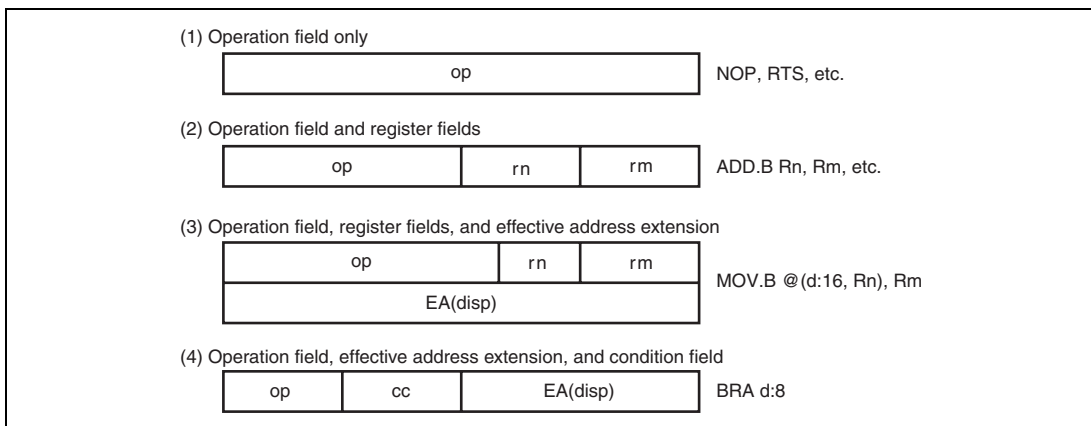
Figure 2.7 Instruction Formats
