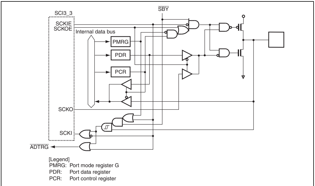
Figure B.32 Port H Block Diagram (PH0)
