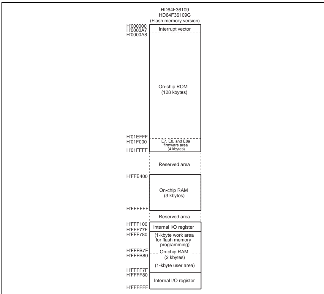
Figure 2.1 Memory Map
