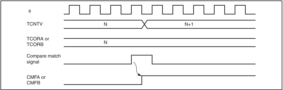
Figure 12.5 CMFA and CMFB Set Timing
