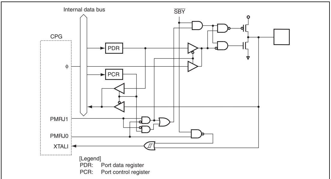
Figure B.33 Port J Block Diagram (PJ1)
