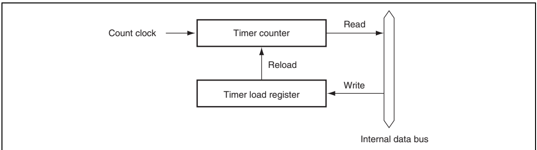
Figure 2.13 Example of Timer Configuration with Two Registers Allocated to Same Address
