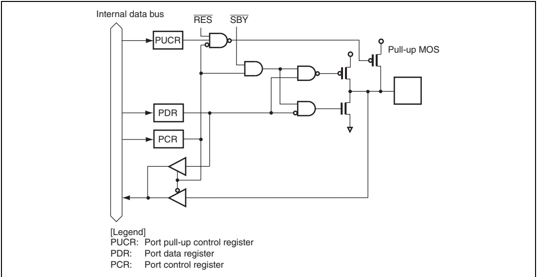
Figure B.4 Port 1 Block Diagram (P12)
