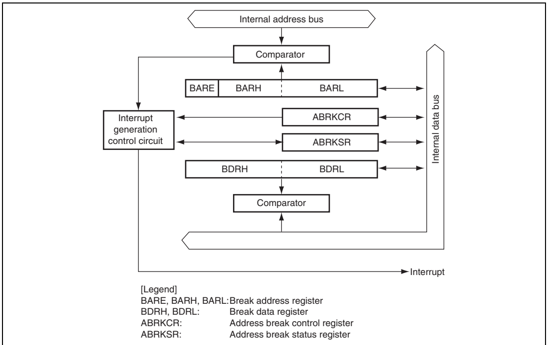
Figure 4.1 Block Diagram of Address Break
