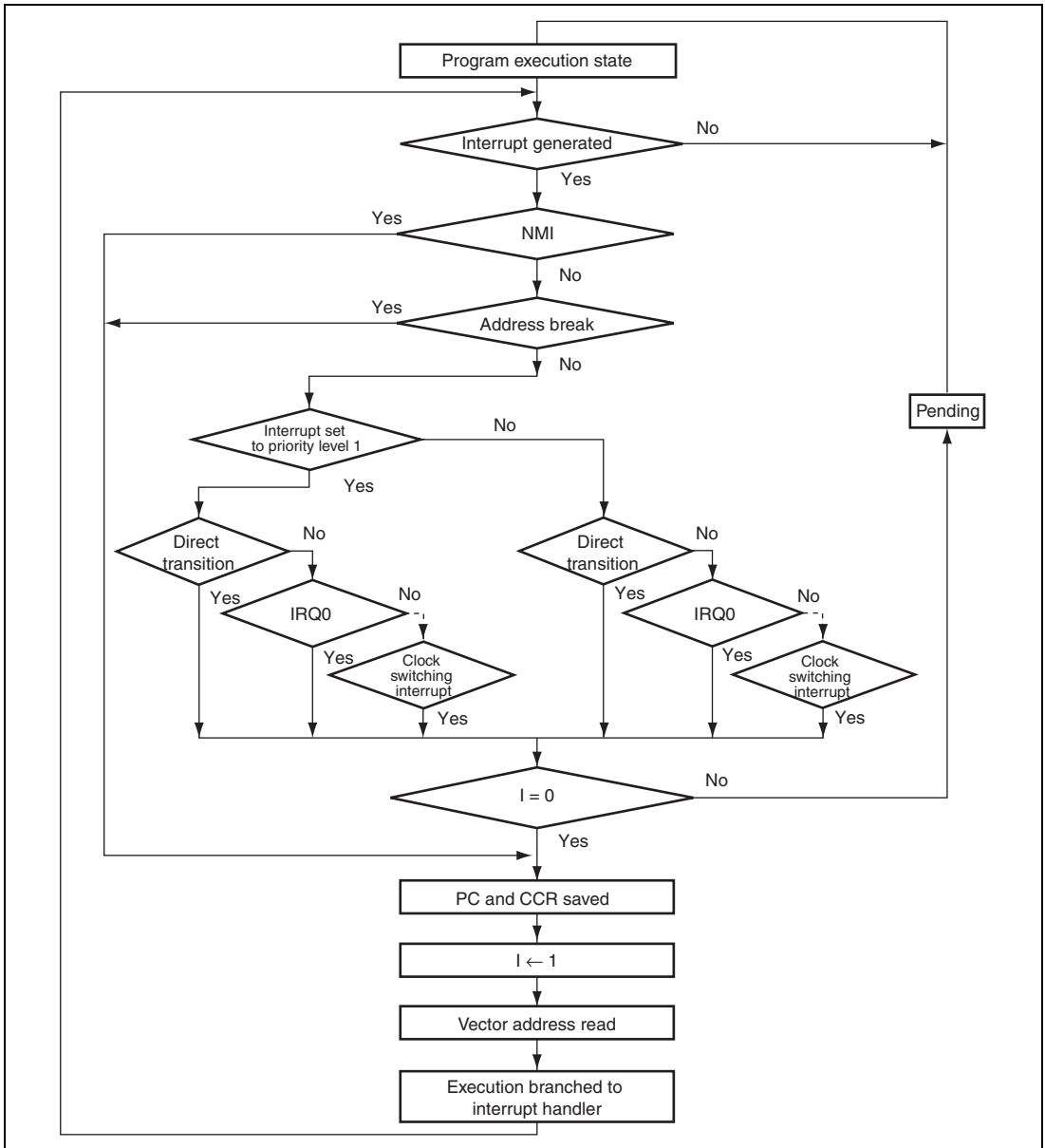
Figure 3.2 Interrupt Acceptance Flowchart
