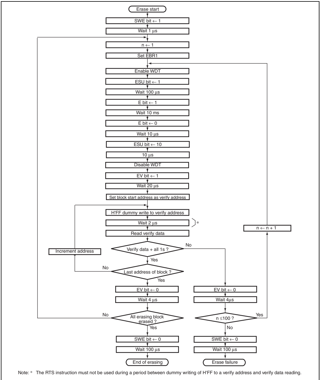
Figure 7.4 Erasure/Erase-Verify Flowchart
