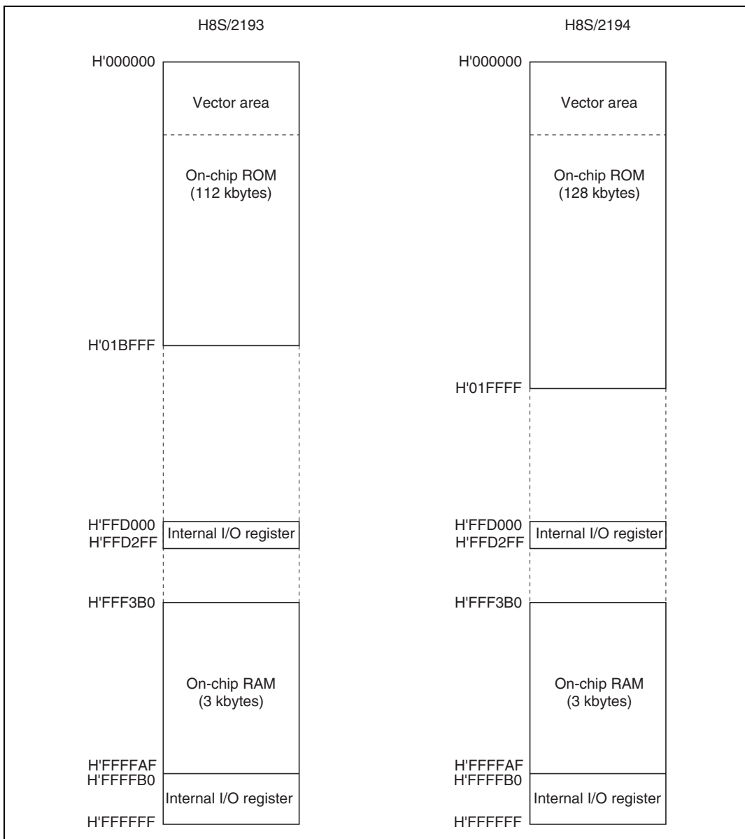
Figure 3.2 Address Map (2)
