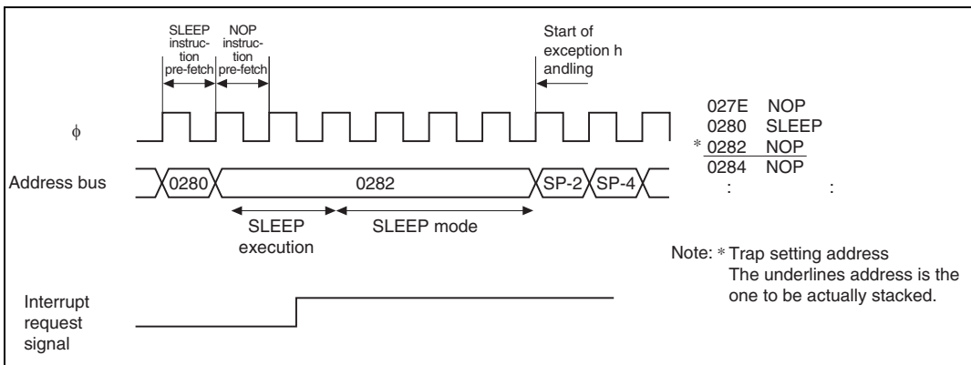
Figure 27.18 SLEEP Instruction (3)
