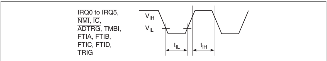
Figure 29.15 Input Timing
