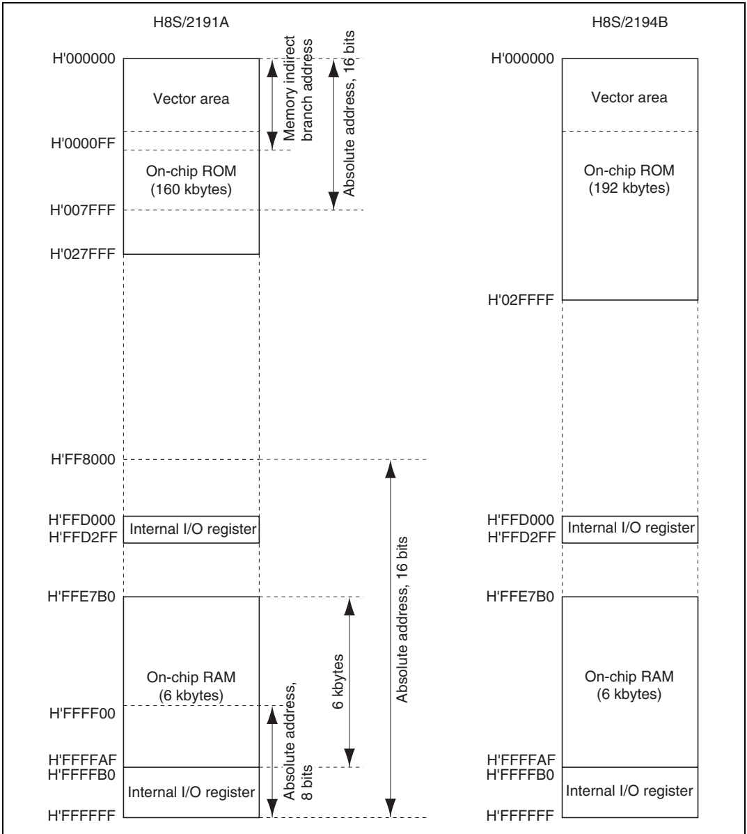
Figure 3.3 Address Map (3)
