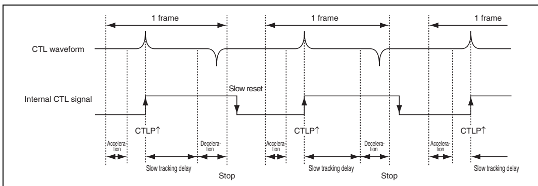
Figure 28.54 PB-CTL Waveform in Slow Mode Operation
