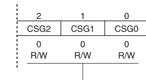
Capstan system gain control bit
