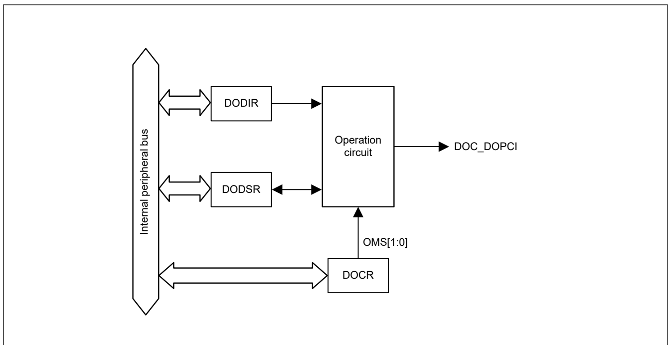
Figure 31.1 DOC block diagram
