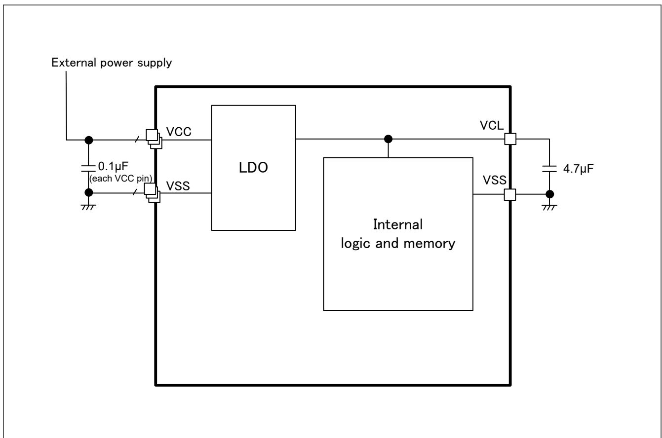
Figure 34.1 LDO settings
