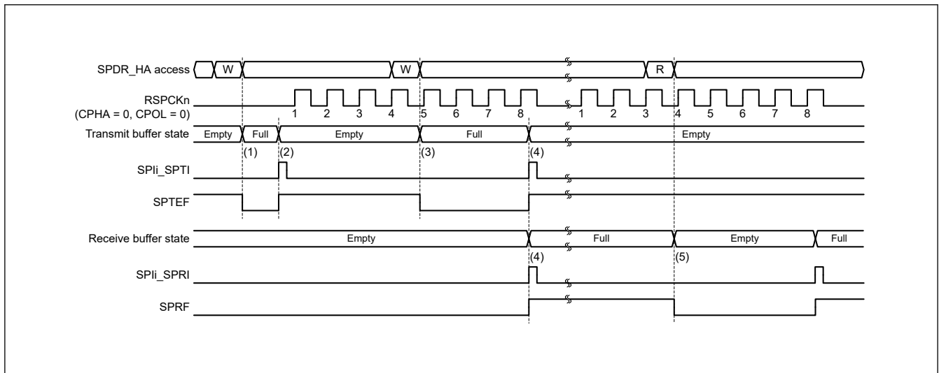
Figure 27.25 Operation example of the SPI_SPTI and SPI_SPRI interrupts when CPHA = 0 and CPOL = 0 in master mode
