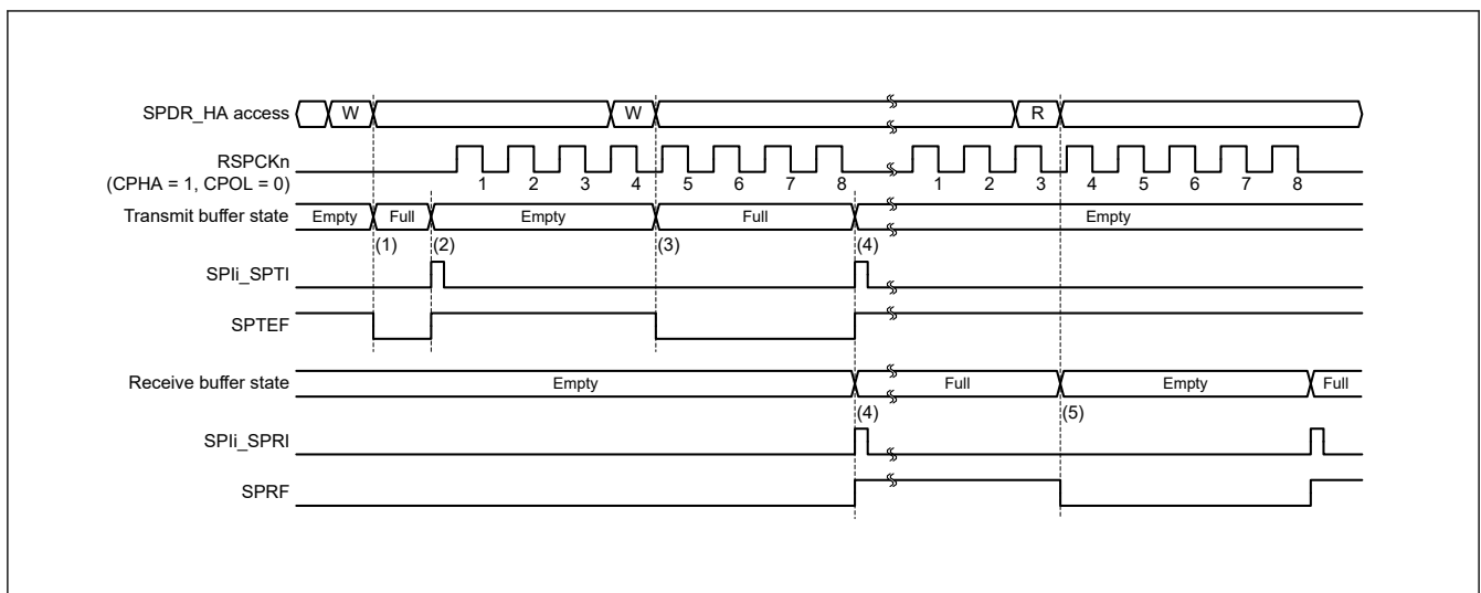
Figure 27.26 Operation example of the SPI_SPTI and SPI_SPRI interrupts when CPHA = 1 and CPOL = 0 in master mode
