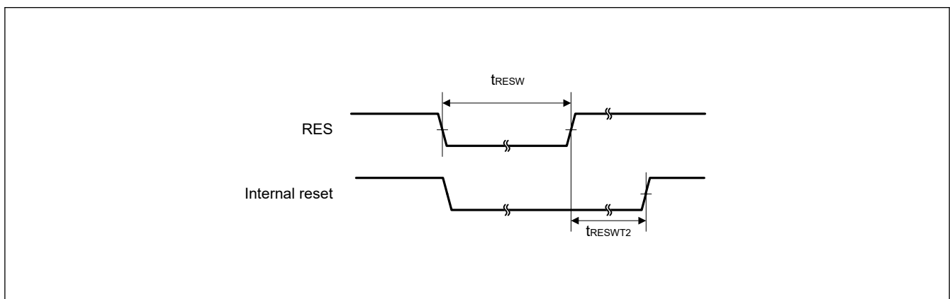
Figure 35.8 Reset input timing (1)
