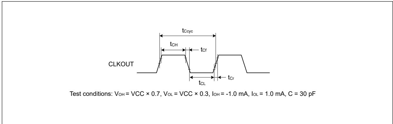
Figure 35.36 CLKOUT output timing
