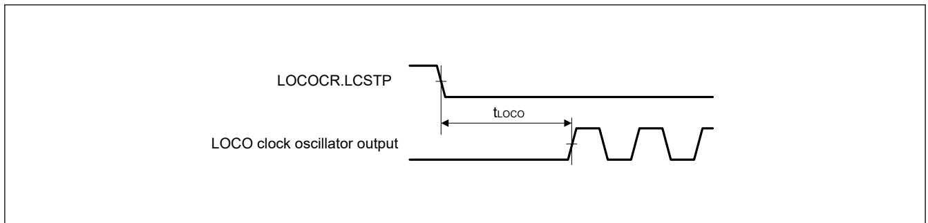
Figure 35.4 LOCO clock oscillation start timing
