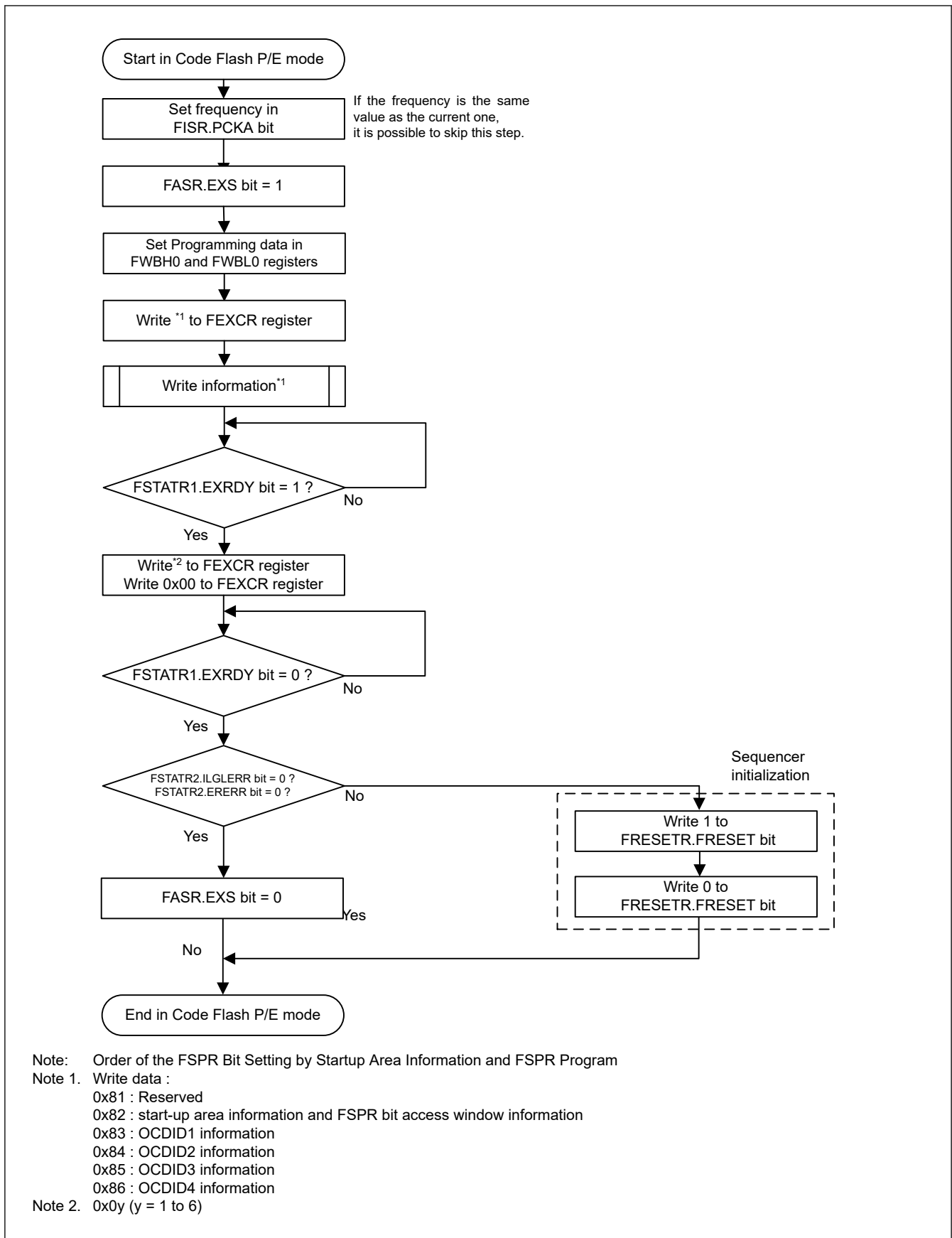
Figure 33.29 Simple flowchart for the procedure for Startup Area Information and FSPR Program/Access Window Information Program/OCDID information Program
