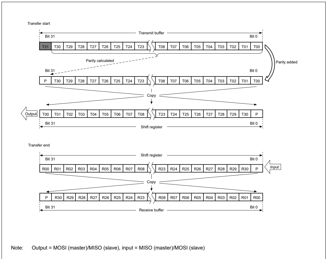
Figure 27.19 LSB-first transfer with 32-bit data and parity enabled
