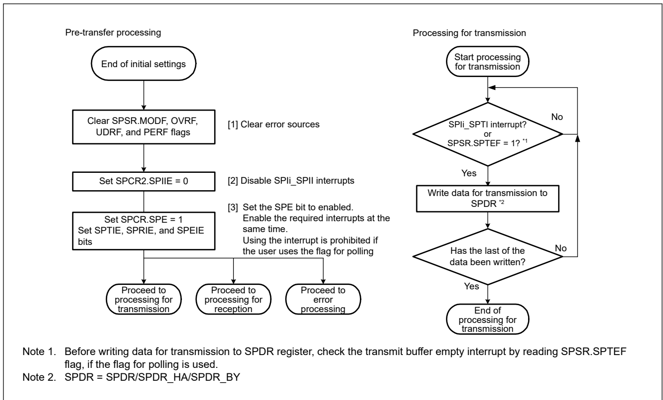
Figure 27.36 Transmission flow in slave mode
