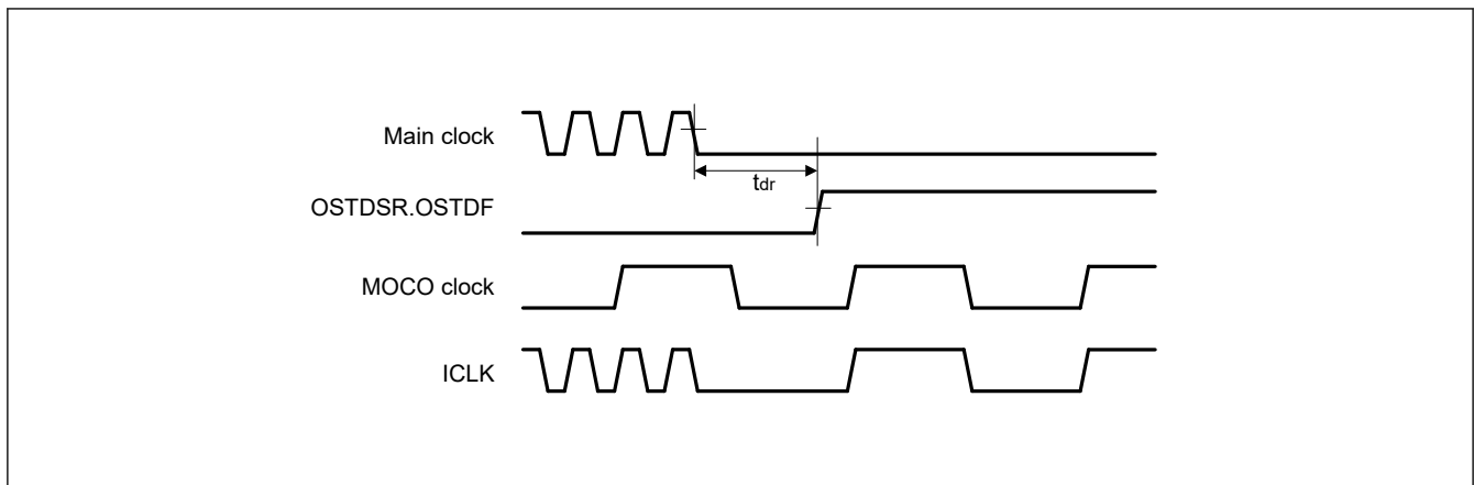
Figure 35.40 Oscillation stop detection timing
