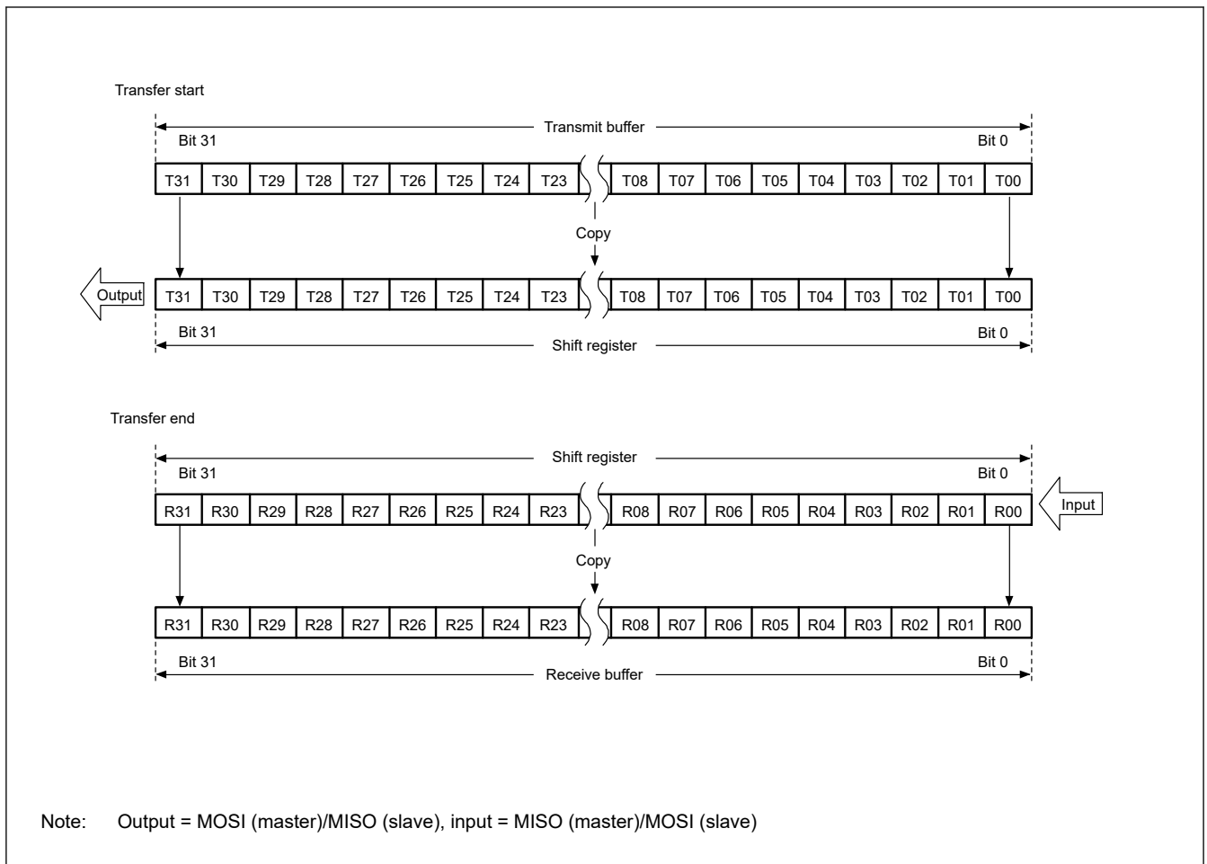
Figure 27.13 MSB-first transfer with 32-bit data and parity disabled
