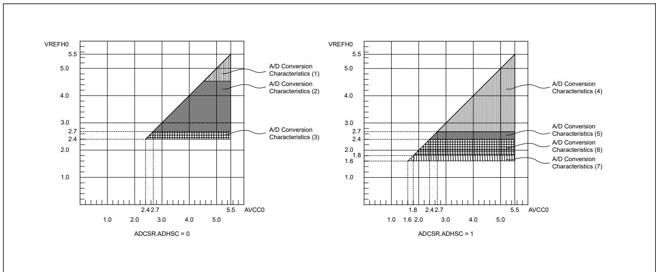
Figure 35.37 AVCC0 to VREFH0 voltage range
