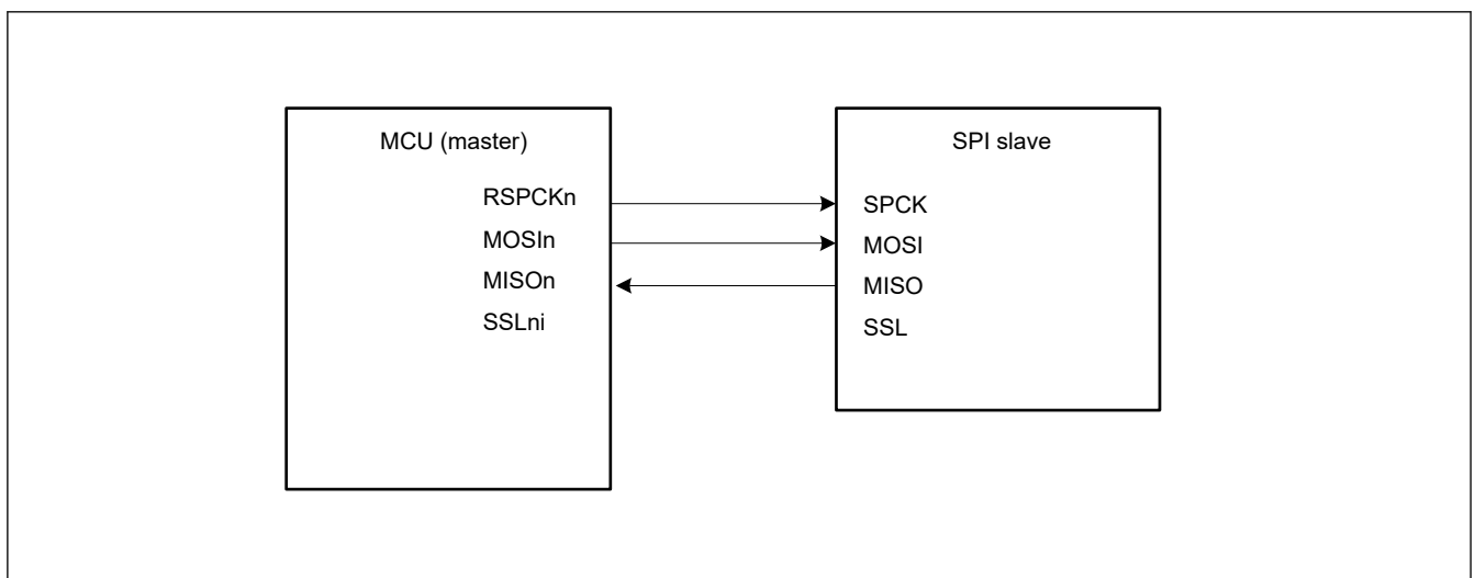
Figure 27.10 Clock synchronous master/slave configuration example with the MCU as a master
