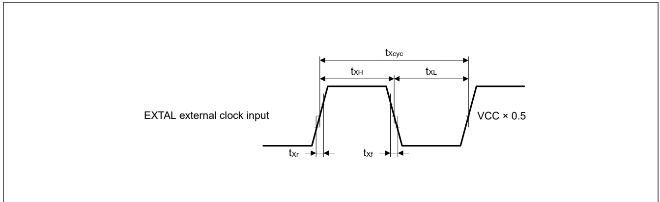
Figure 35.3 EXTAL external clock input timing
