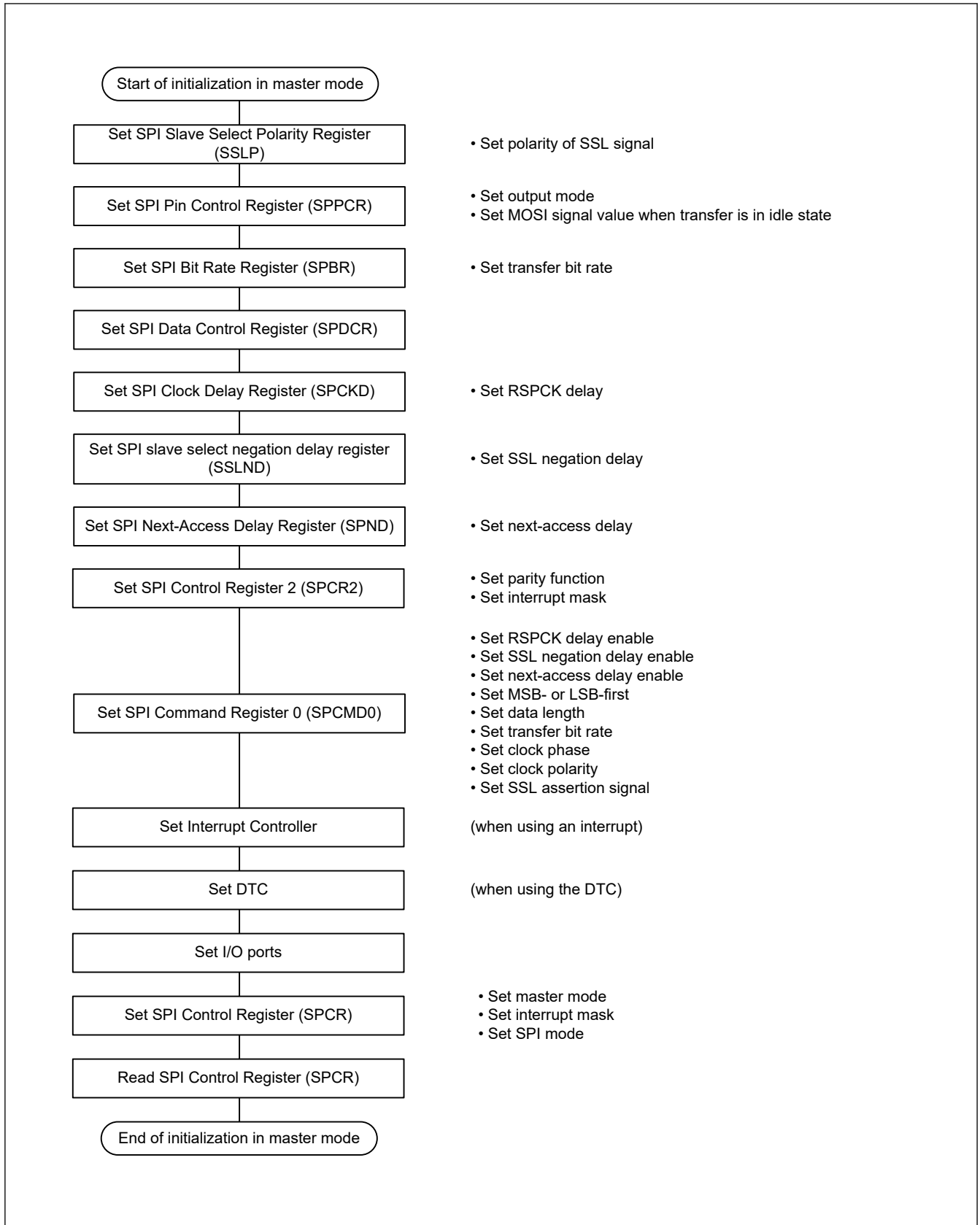
Figure 27.31 Example of initialization flow in master mode for SPI operation
