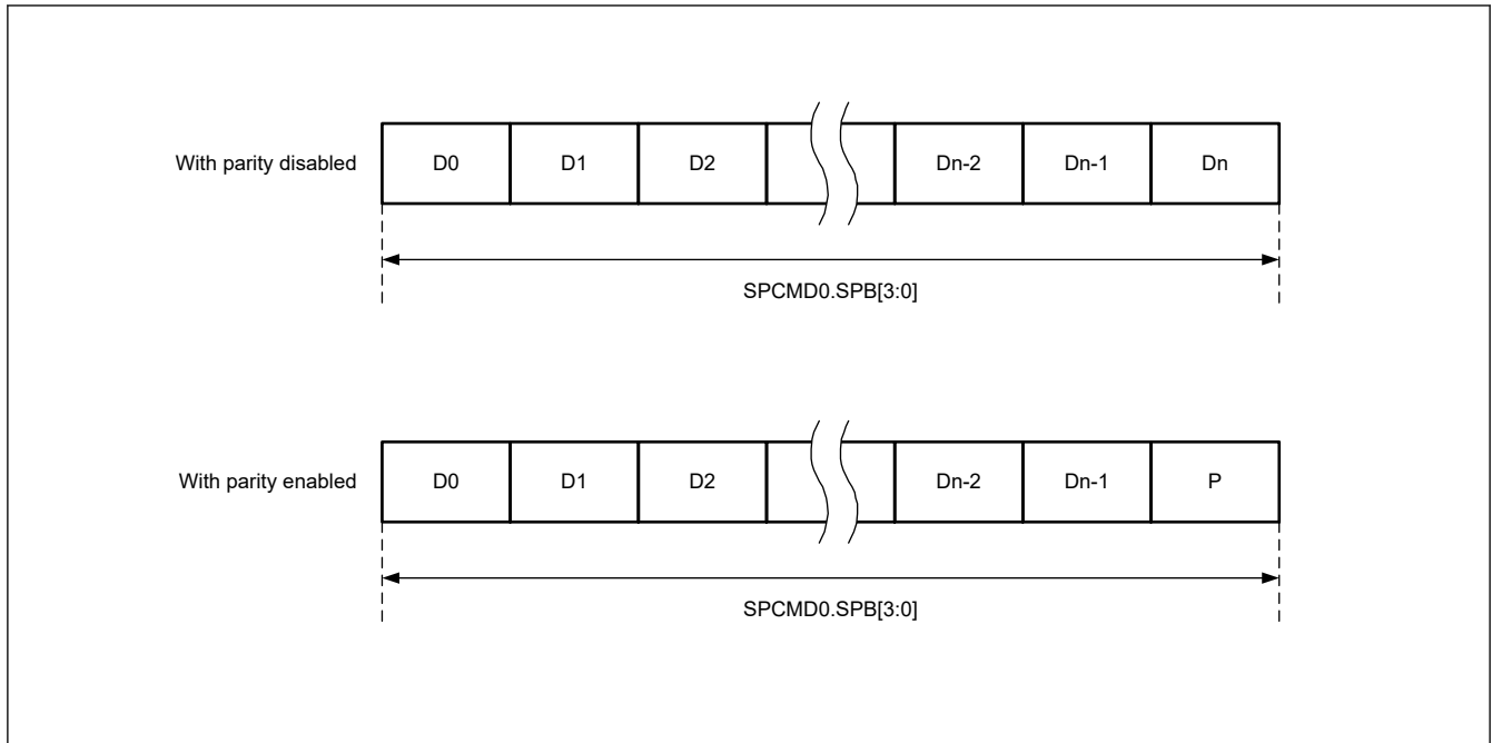
Figure 27.12 Data format with parity disabled and enabled
