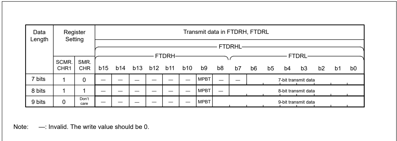
Figure 25.28 Data format written to FTDRH and FTDRL in multi-processor mode with FIFO selected
