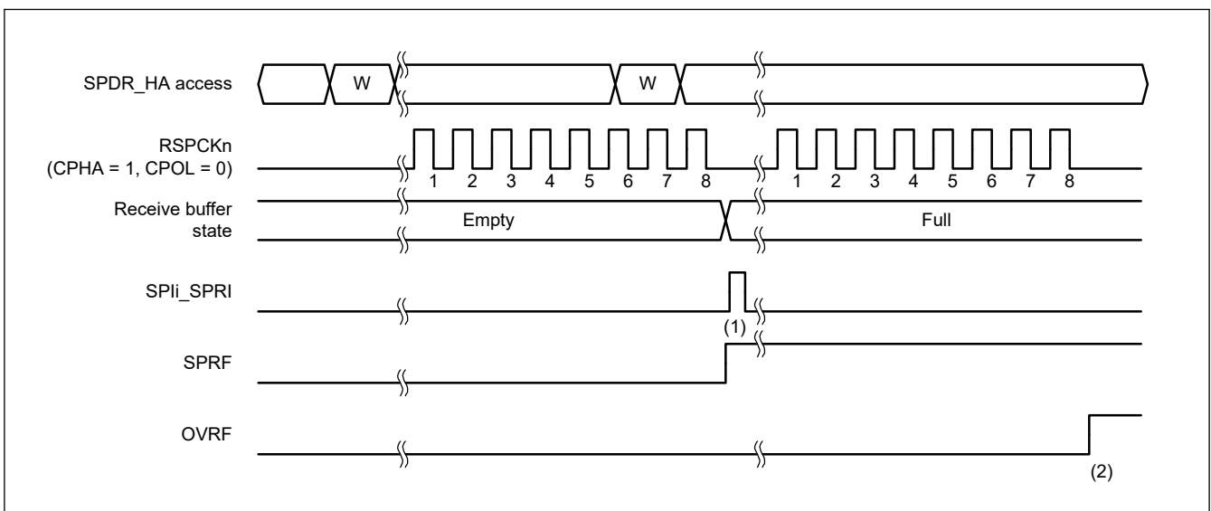
Figure 27.23 Operation example when SPCR.TXMD = 0
