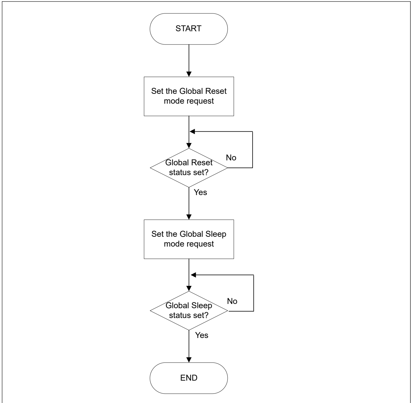
Figure 28.3 Procedure for entering Global Sleep mode
