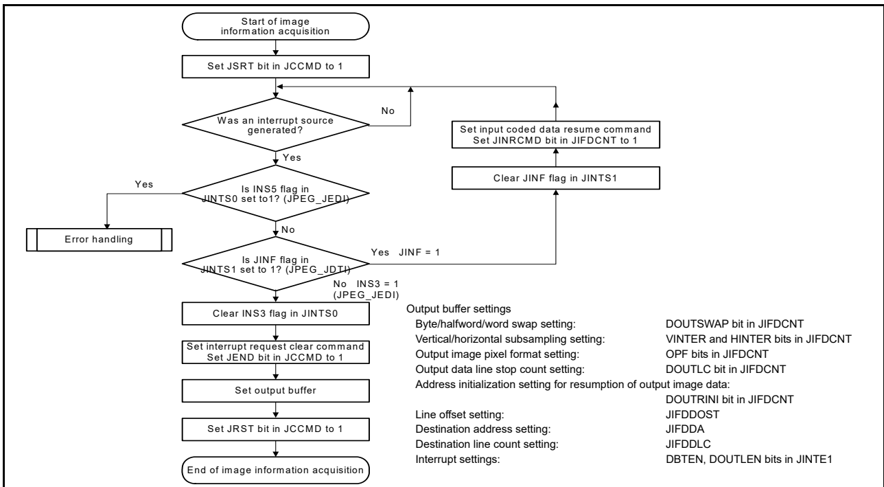
Figure 57.8 Flow of image information acquisition
