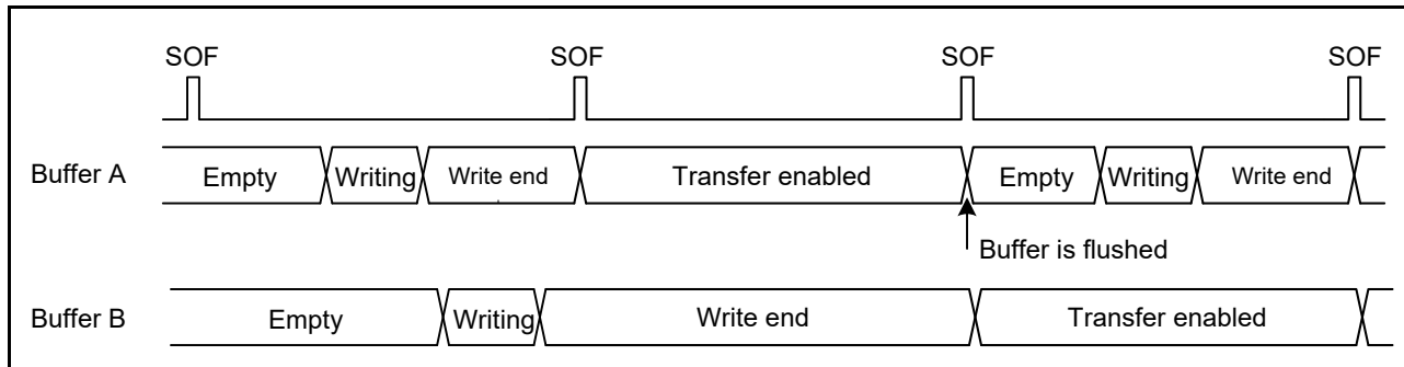
Figure 32.21 Example buffer flush operation
