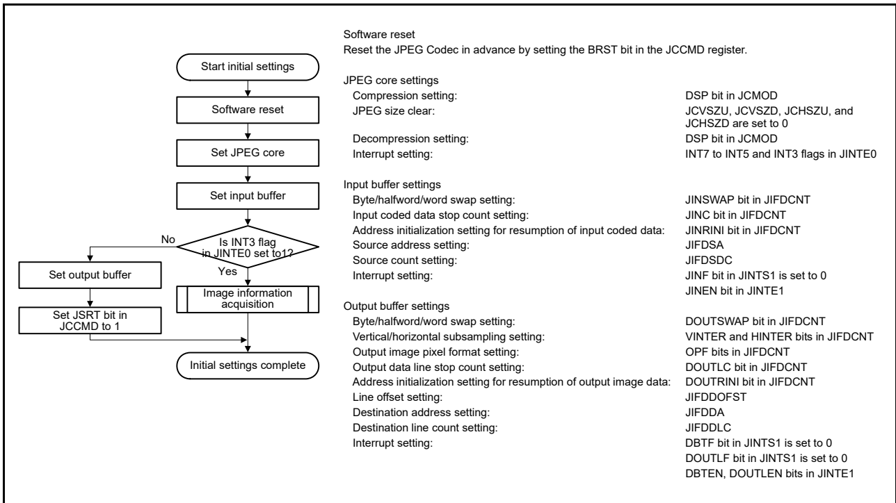
Figure 57.7 Flow of decompression initial settings
