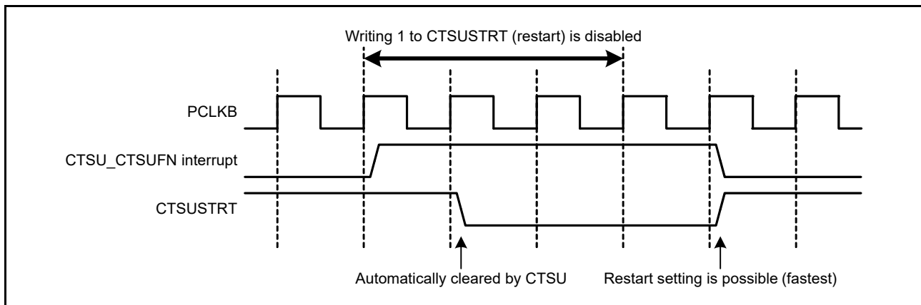
Figure 51.21 Notes on restarting measurement
