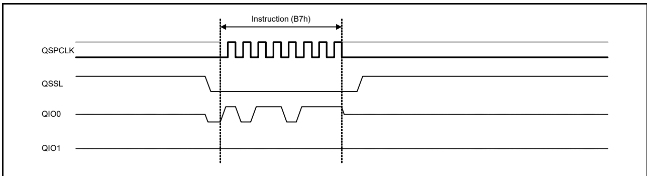
Figure 39.26 Enter 4-Byte Mode bus cycle
