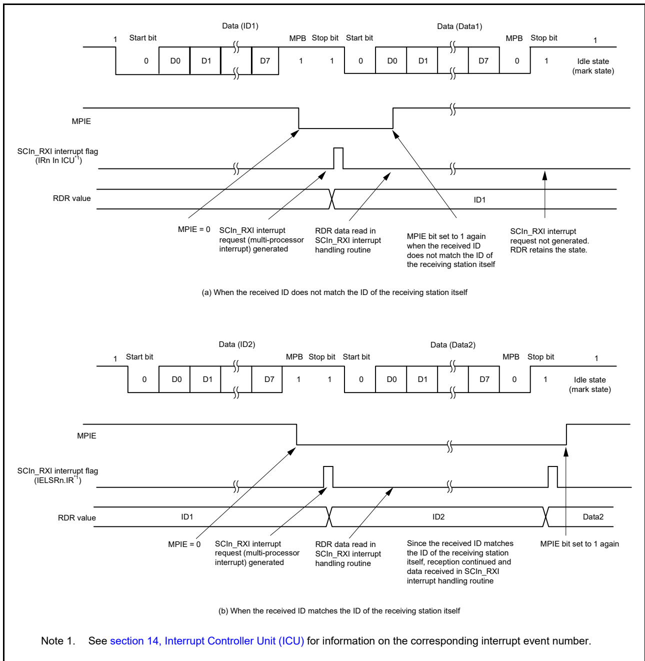
Figure 34.26 Example of SCI reception with 8-bit data, multi-processor bit, and 1 stop bit
