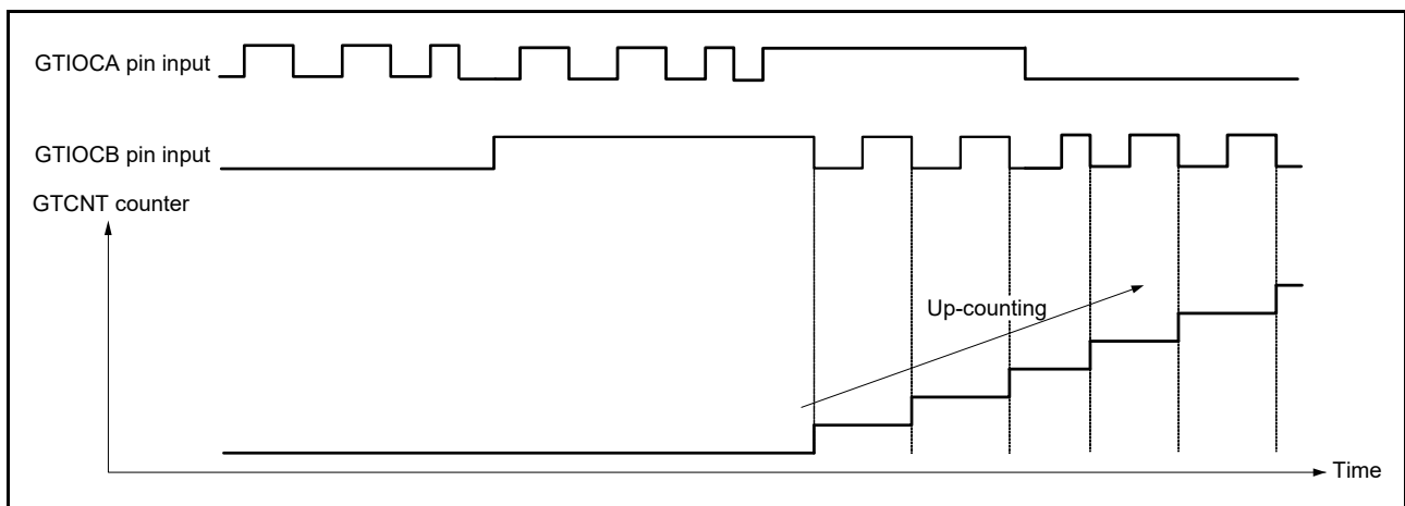
Figure 23.80 Example of phase counting mode 5 (B)
