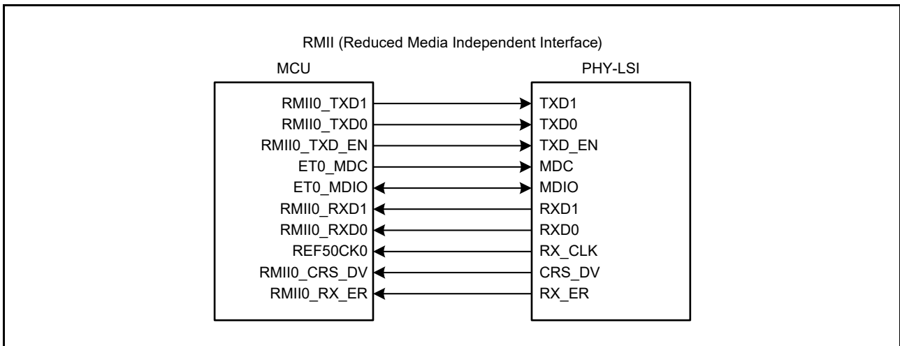
Figure 29.3 Example of connection with PHY-LSI for RMI
