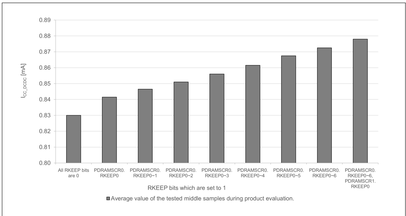
Figure 55.8 Software Standby current per SRAM state (reference data)
