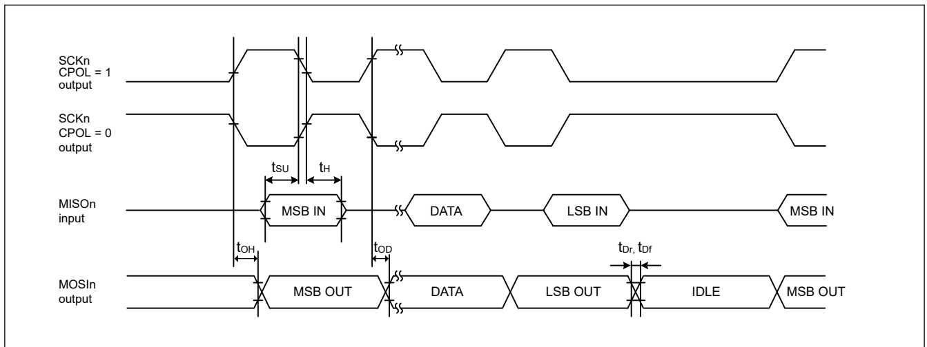
Figure 55.54 SCI simple SPI mode timing for master when CPHA = 1
