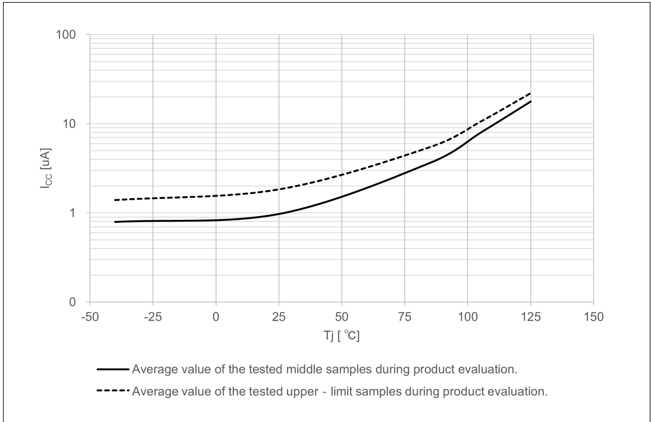
Figure 55.7 Temperature dependency in Deep Software Standby mode 3 (reference data)
