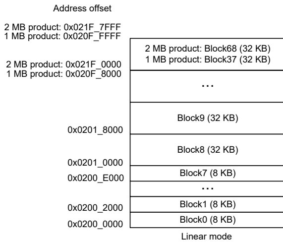
Figure 6.3 Code Flash block structure
