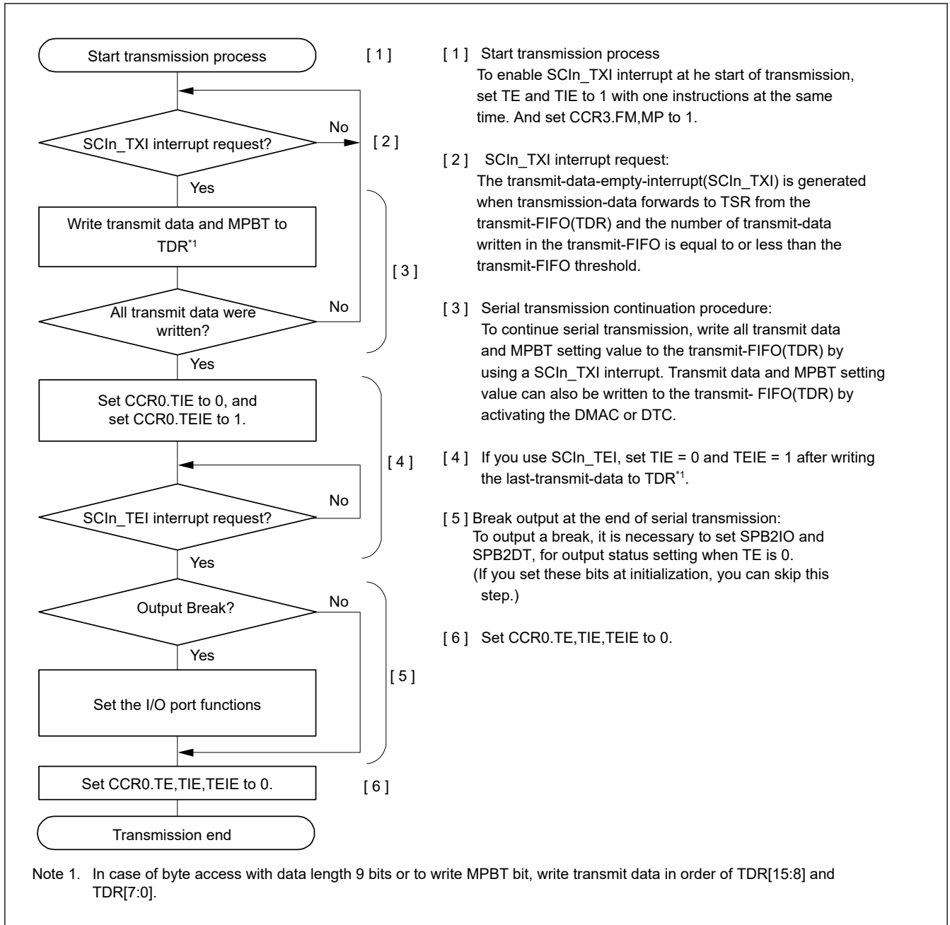
Figure 31.38 Example flow of serial transmission in multi-processor mode with FIFO selected
