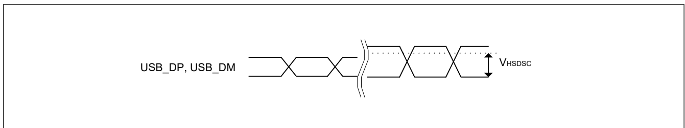
Figure 55.113 USB_DP and USB_DM disconnect detect sensitivity (high-speed)
