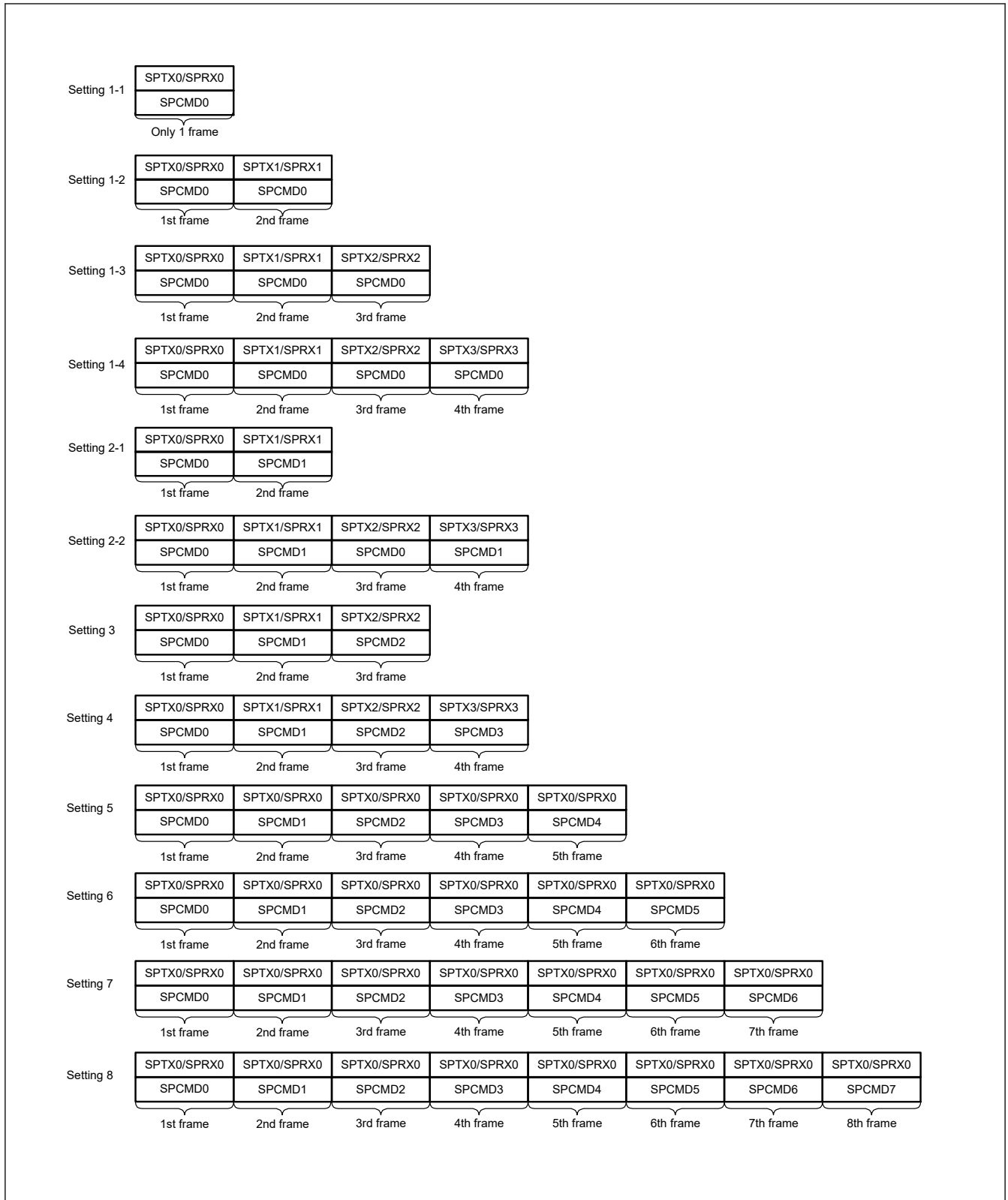
Figure 36.56 Correspondence between SPI Command Register and transmit and receive buffers in sequence operations
