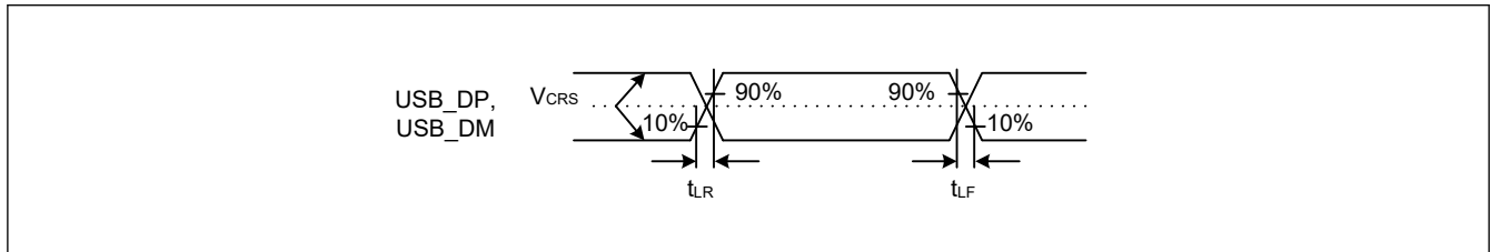
Figure 55.104 USB_DP and USB_DM output timing in low-speed mode
