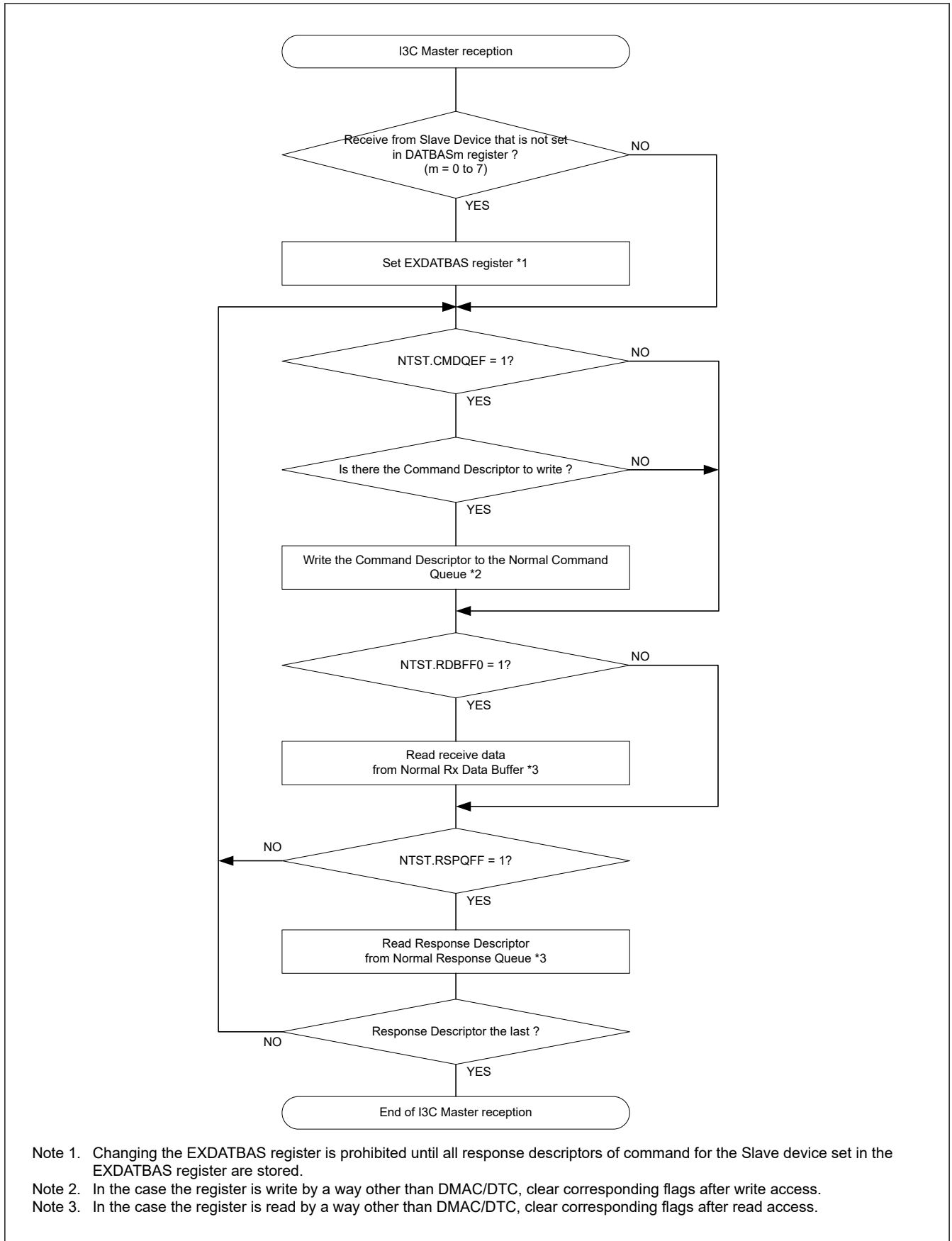
Figure 33.147 Example of I3C master reception flowchart (normal FIFO buffer transfer)
