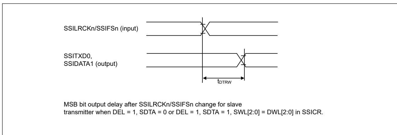
Figure 55.89 SSIE data output delay after SSILRCK0/SSIFSn change
