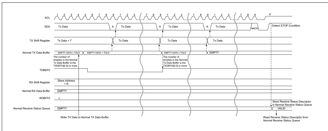
Figure 33.52 Legacy I 2 C message data read transfer timing (2/2)
