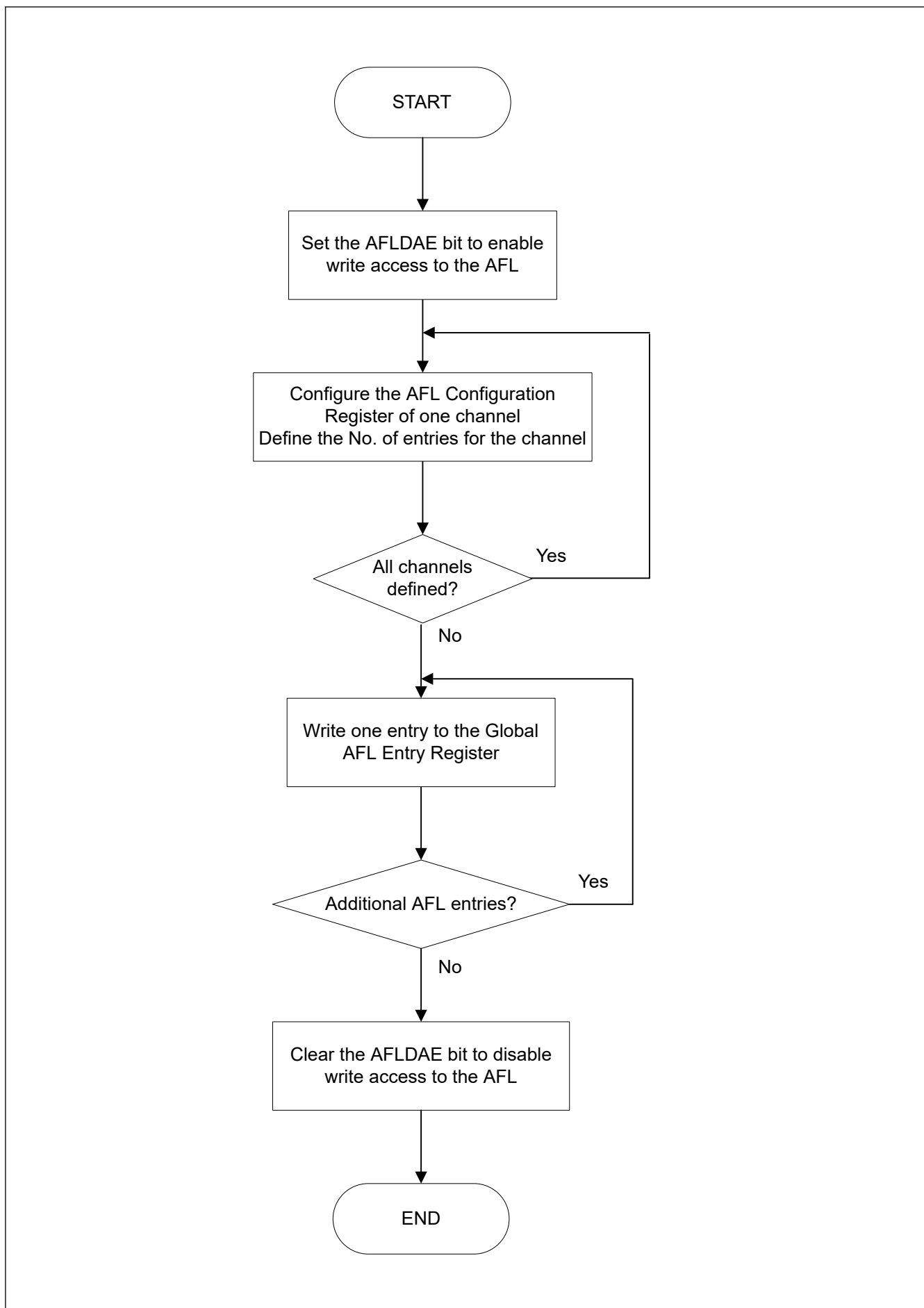
Figure 34.26 AFL configuration flow R01UH0994EJ0120 Rev.1.20 Nov 22, 2024
