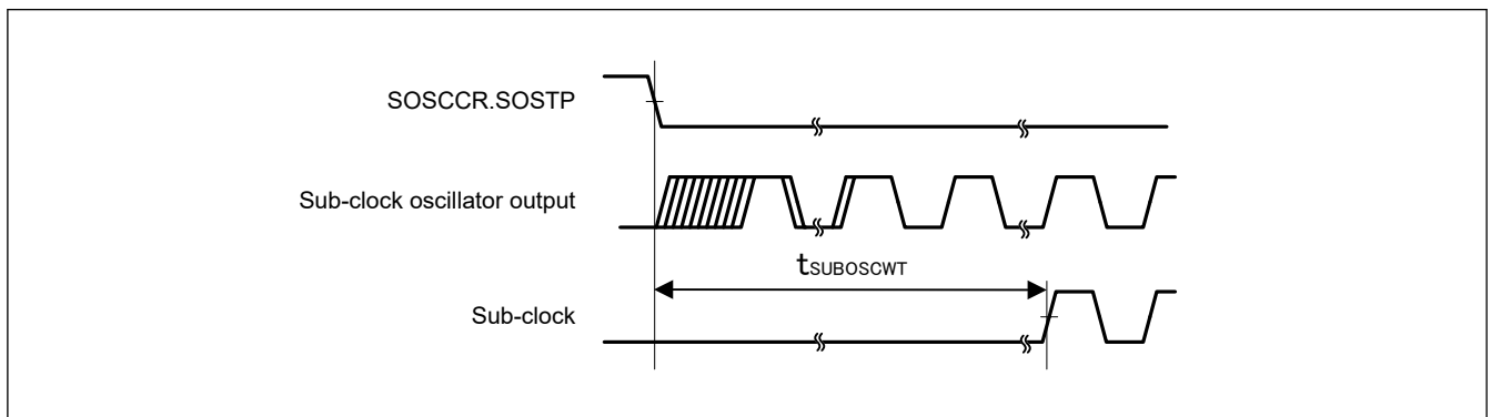
Figure 55.20 Sub-clock oscillation start timing
