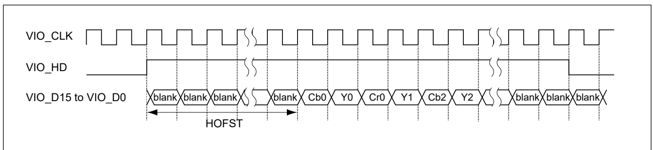
Figure 53.19 Horizontal offset
