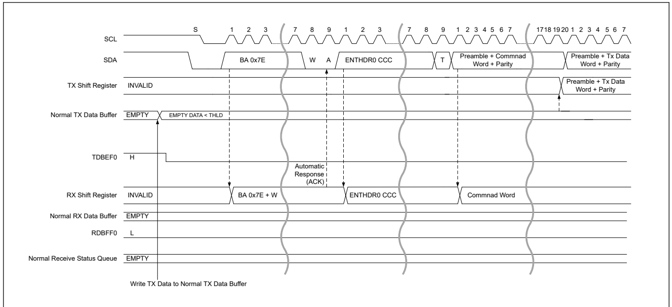
Figure 33.58 HDR data read transfer (HDR-DDR) timing (1/3)
