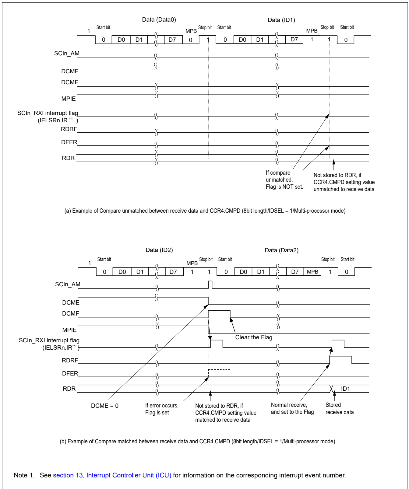
Figure 31.10 Example of address match (2) multi-processor mode
