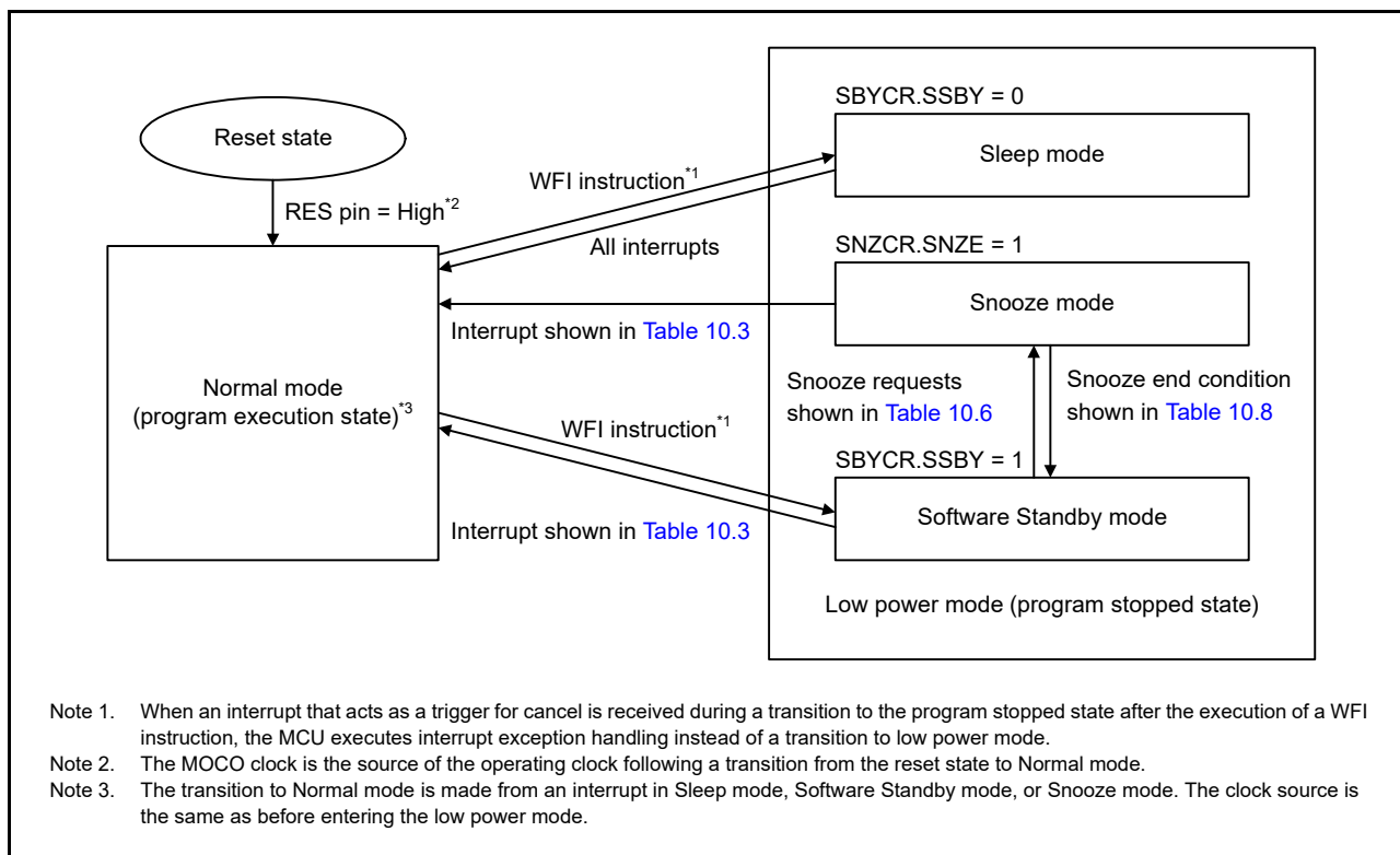
Figure 10.1 Mode transitions
