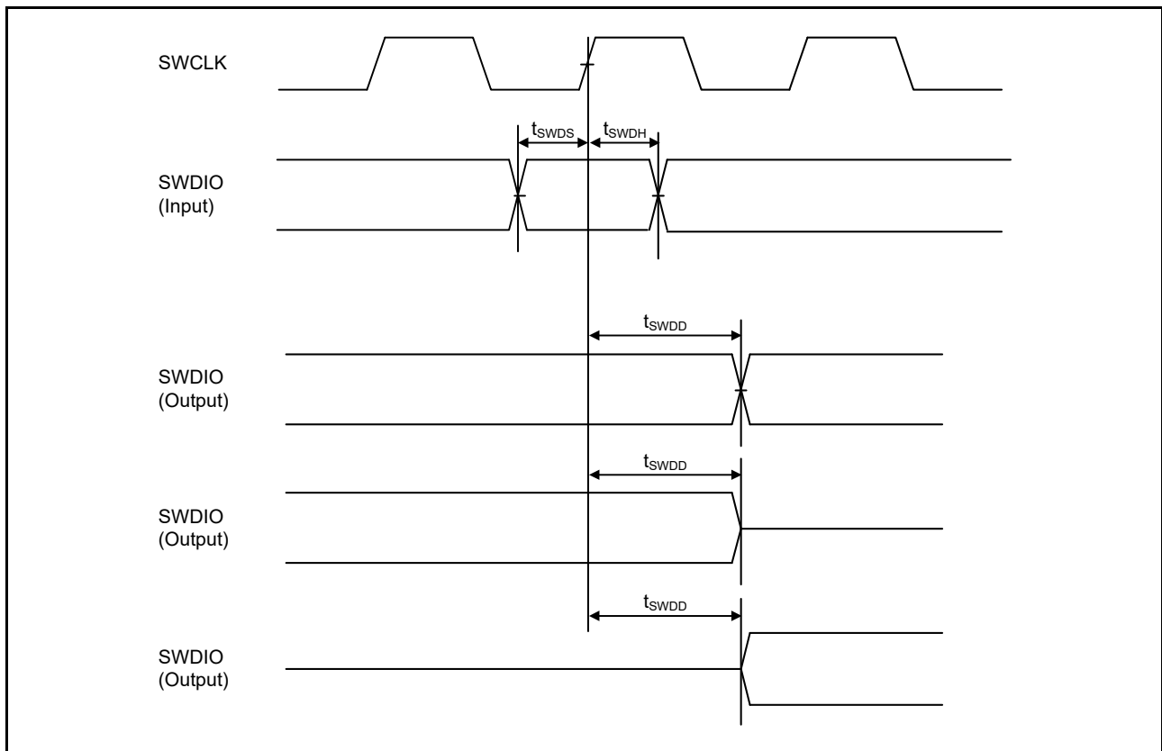
Figure 48.88 SWD input/output timing
