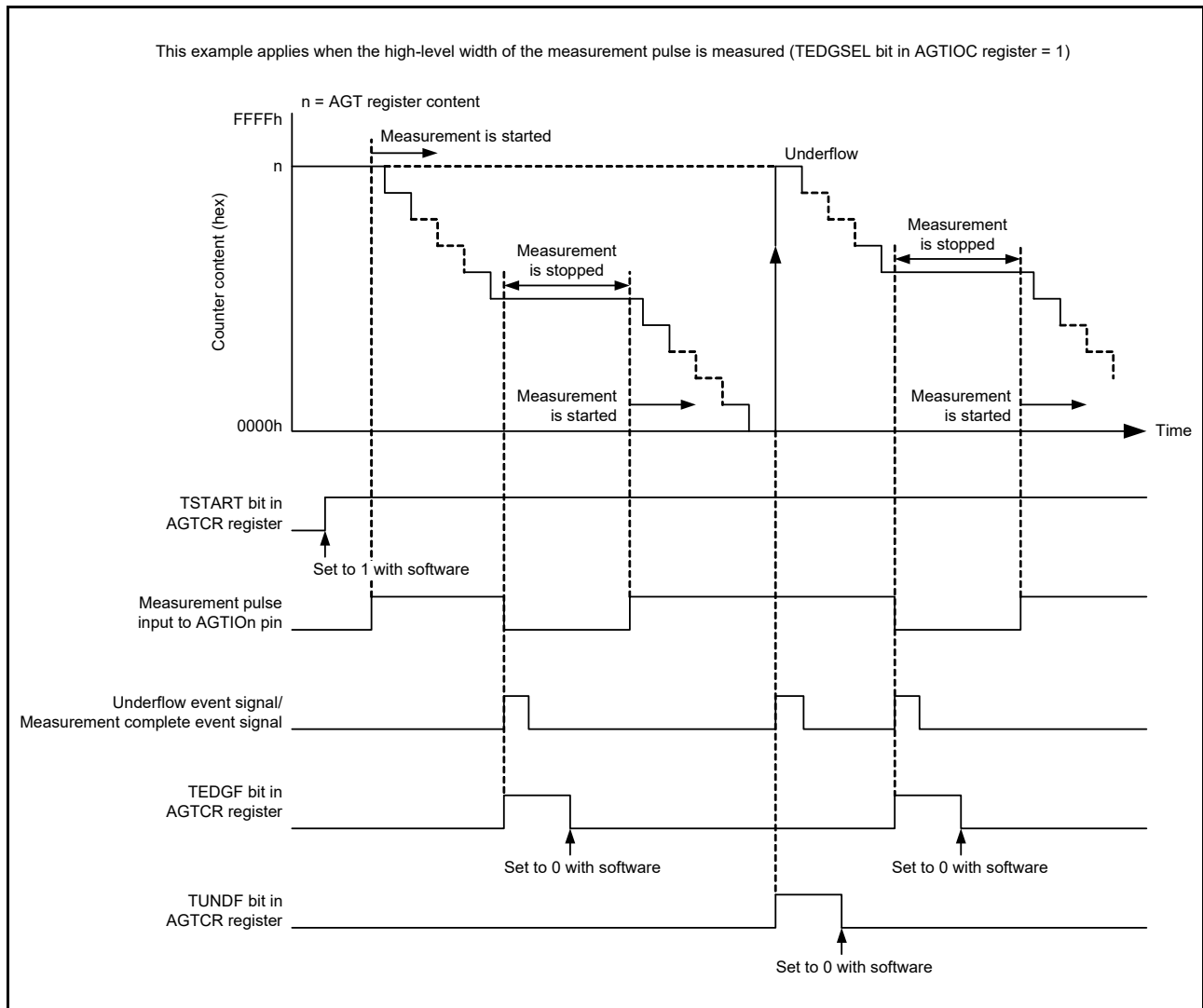
Figure 23.9 Operation example in pulse width measurement mode
