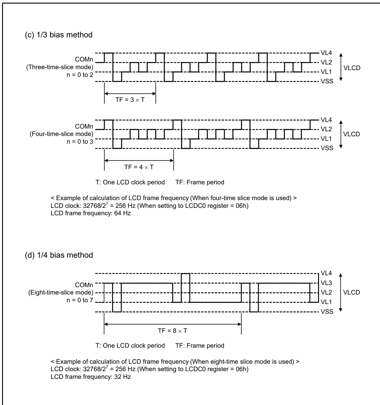
Figure 45.14 Common signal waveforms (2 of 2)
