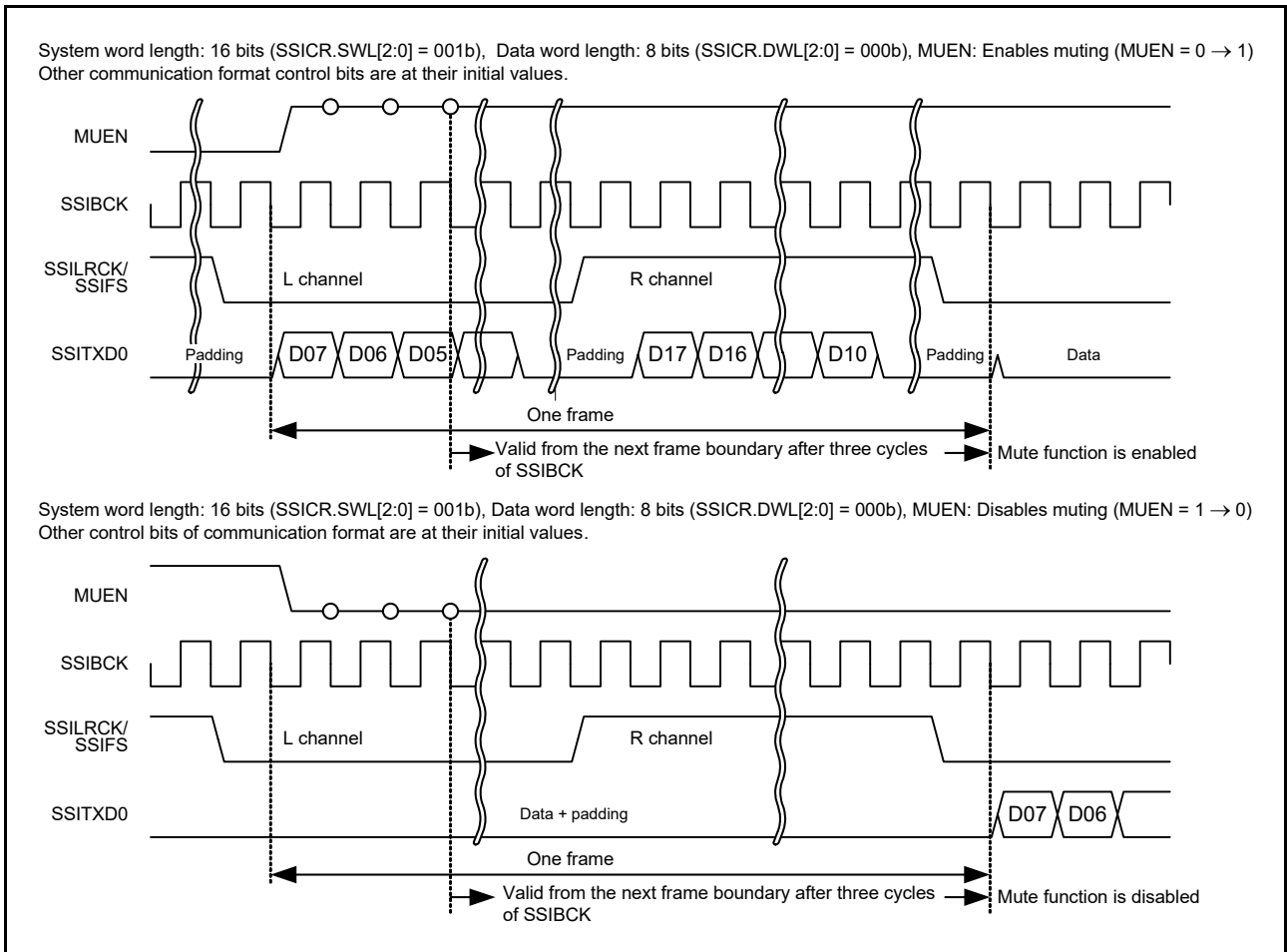
Figure 33.4 Transmit data with the mute function set
