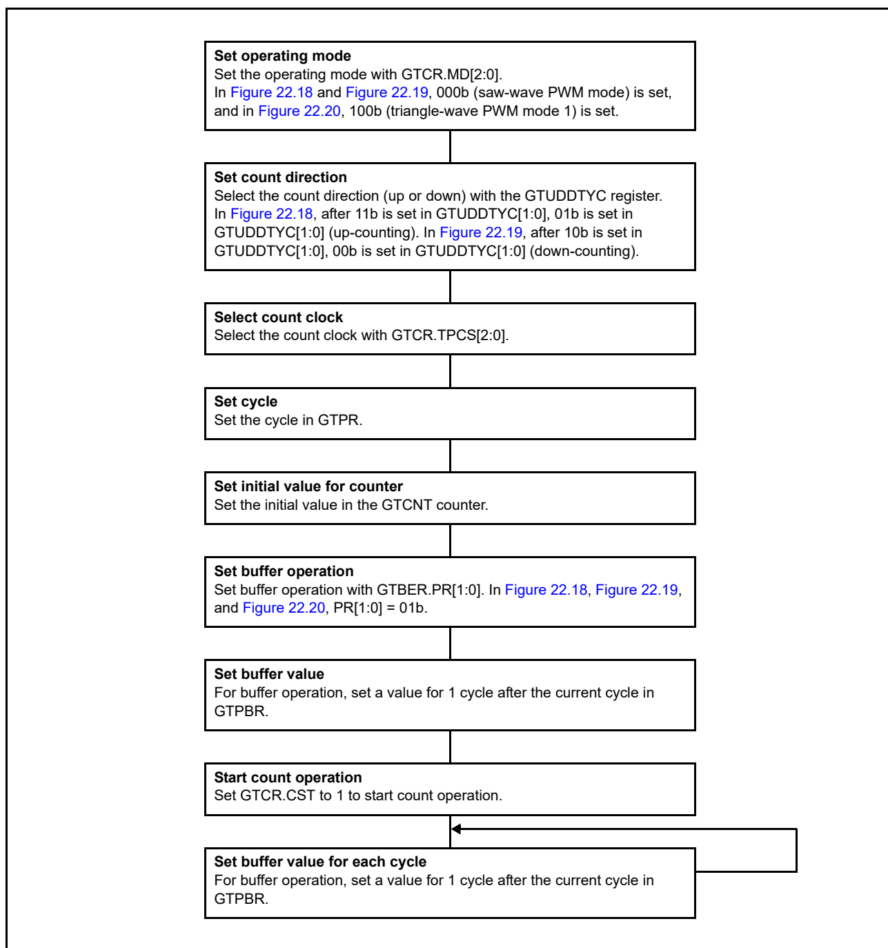
Figure 22.21 Example for setting GTPR buffer operation
