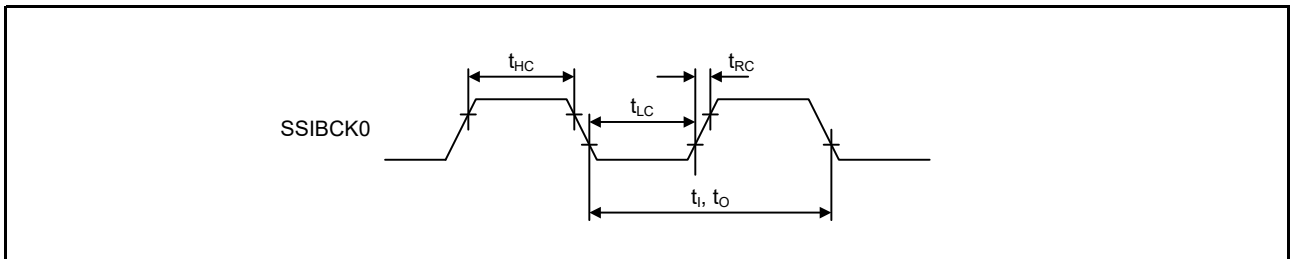
Figure 48.60 SSIE clock input/output timing
