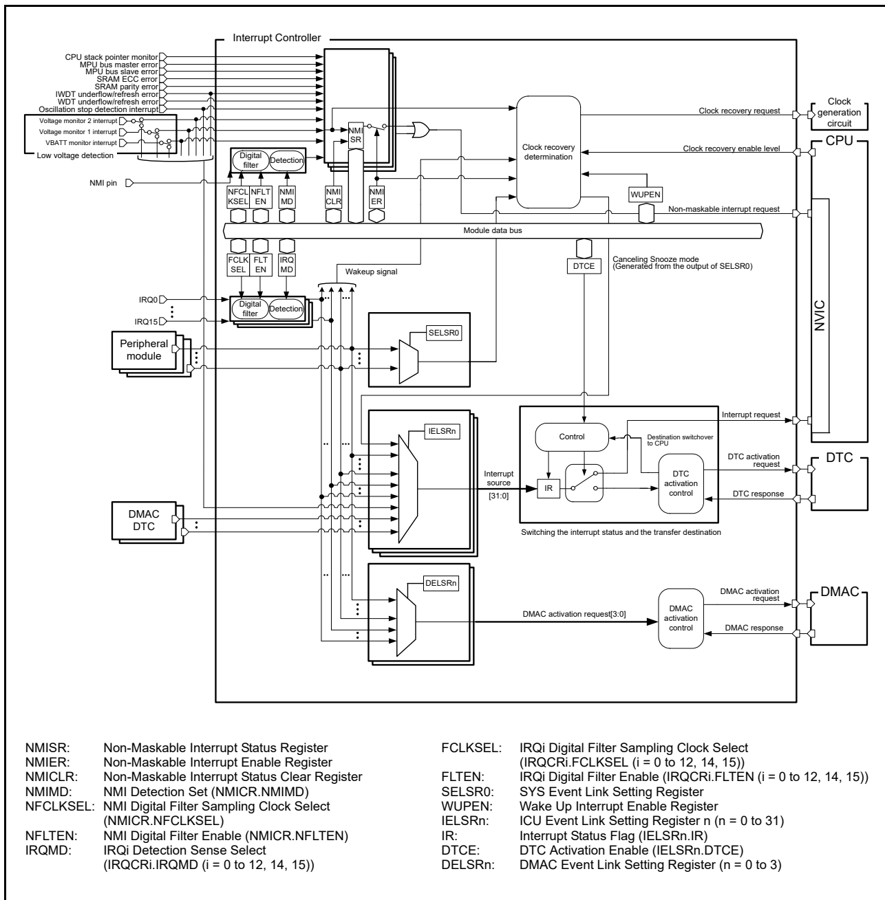
Figure 13.1 ICU block diagram
