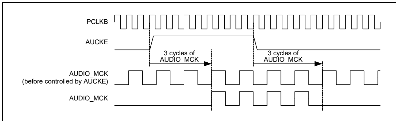
Figure 33.23 Stop/resume of AUDIO_MCK
