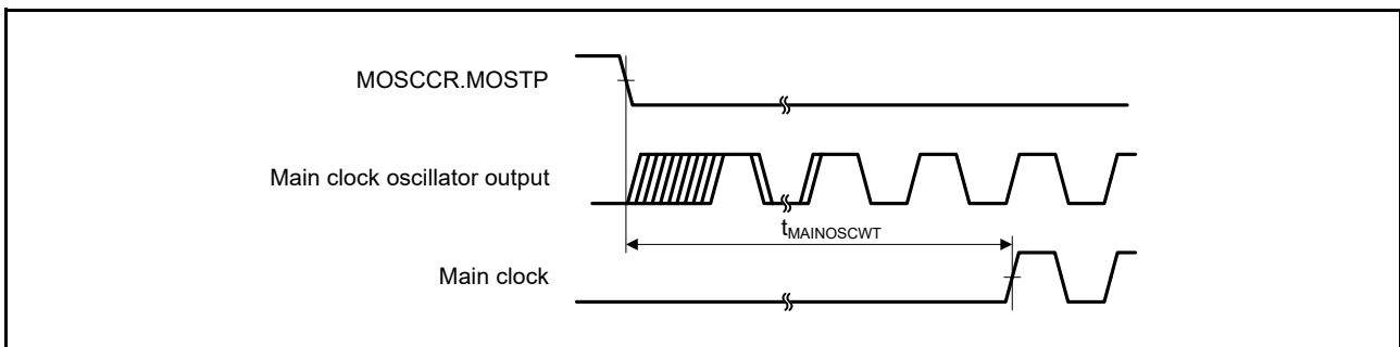
Figure 48.28 Main clock oscillation start timing
