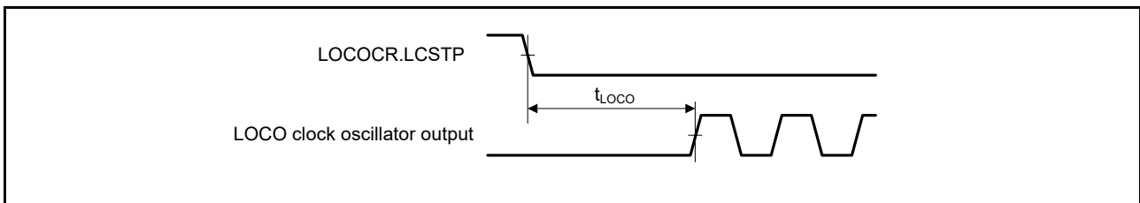
Figure 48.26 LOCO clock oscillation start timing
