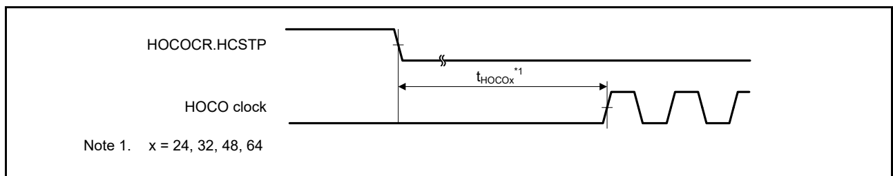
Figure 41.27 HOCO clock oscillator start timing (started by setting the HOCOCCR.HCSTP bit)
