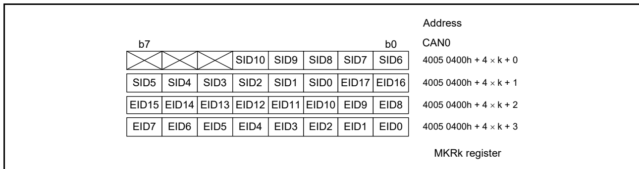
Figure 27.14 Structure of the MKRk registers (k = 0 to 7)
