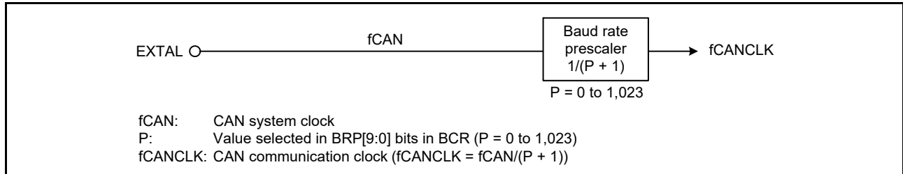
Figure 27.11 Block diagram of CAN clock generator
