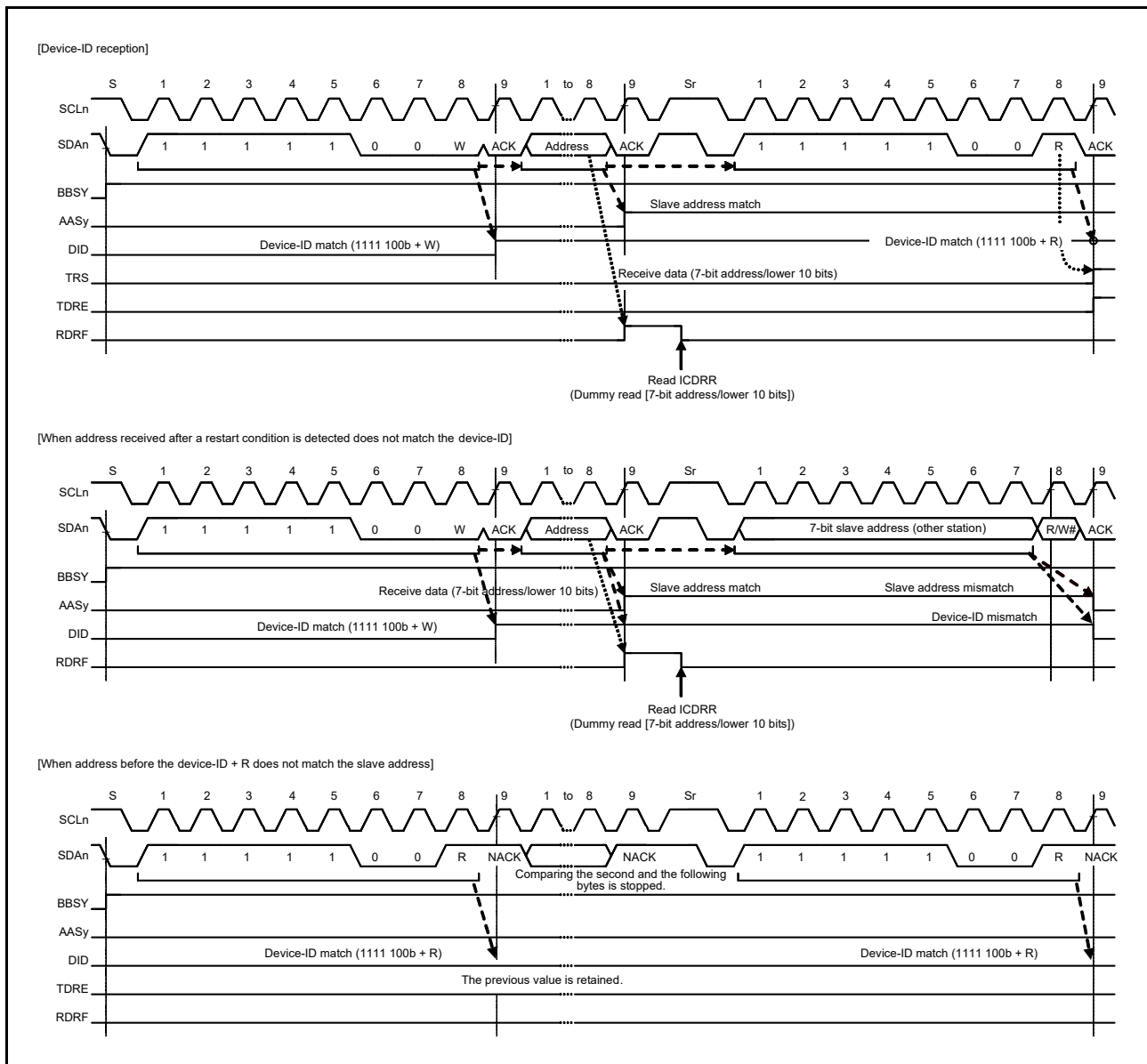
Figure 26.28 AASy/DID flag set and clear timing during reception of device ID
