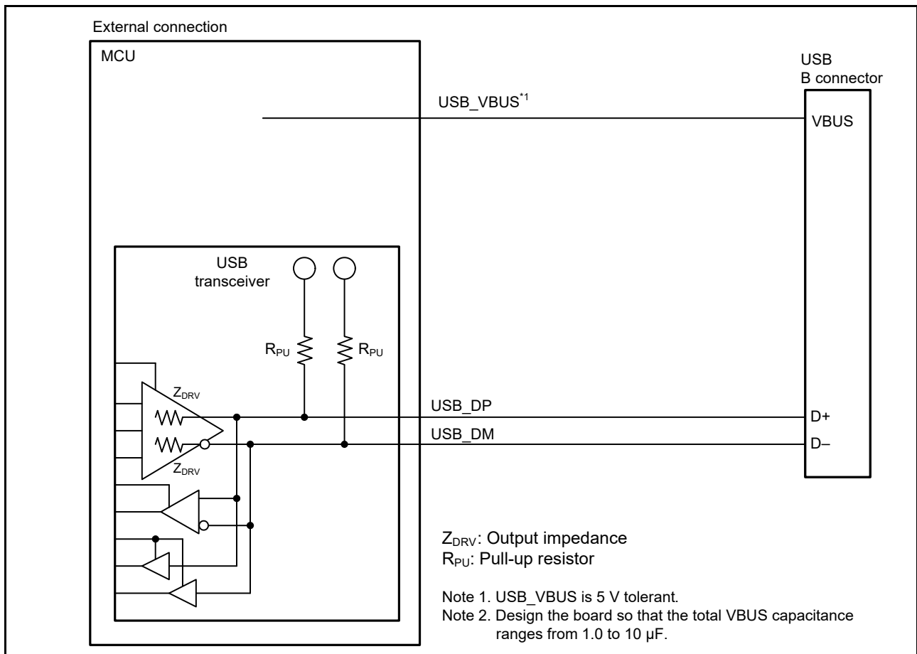
Figure 24.7 Example device connection in bus-powered state 2
