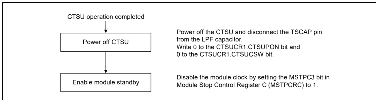
Figure 34.10 CTSUS stopping flow
