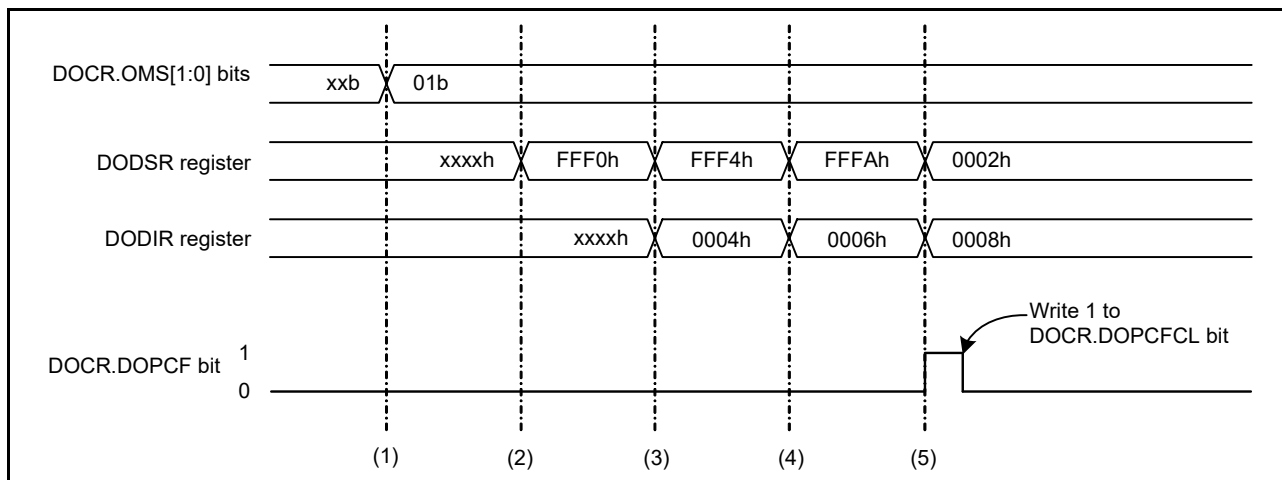
Figure 35.3 Example operation in data addition mode
