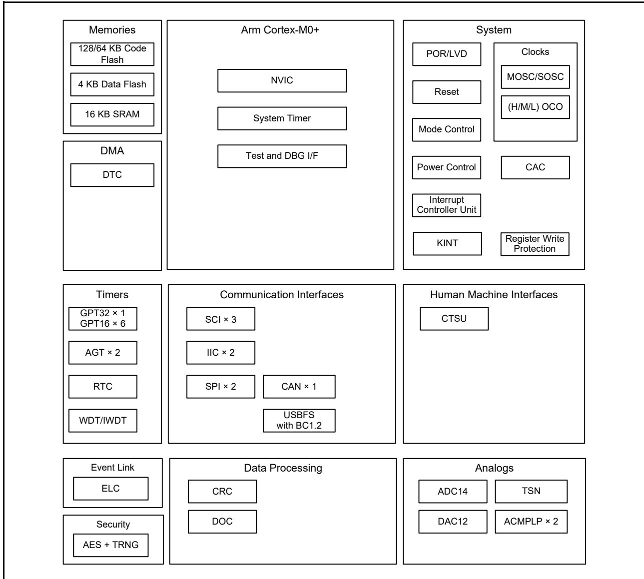
Figure 1.1 Block diagram
