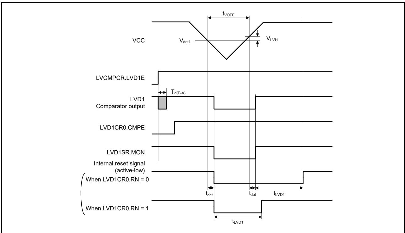
Figure 41.69 Voltage detection circuit timing (V det1 )
