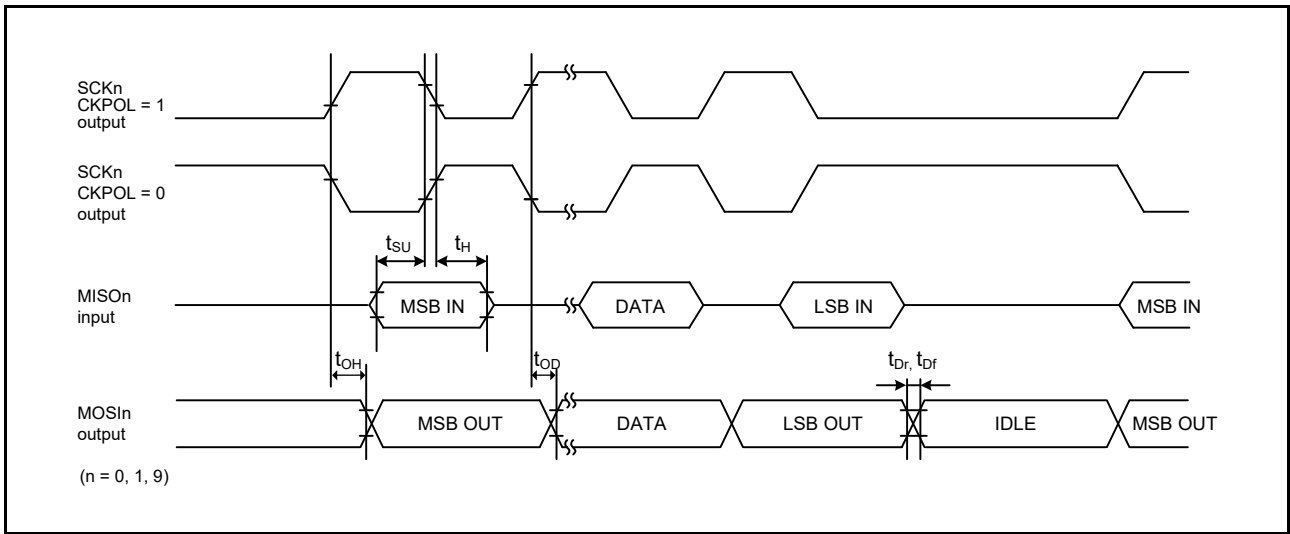
Figure 41.45 SCI simple SPI mode timing (master, CKPH = 0)
