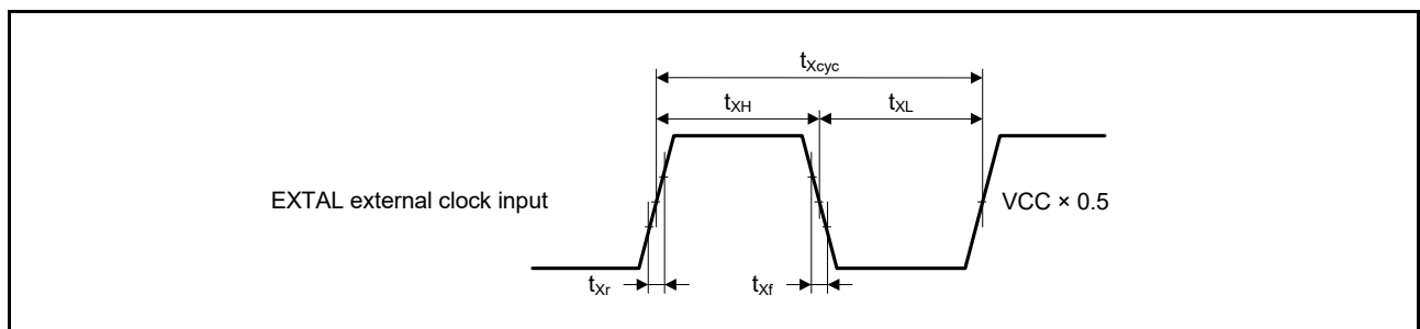
Figure 41.25 EXTAL external clock input timing
