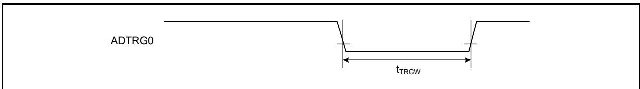
Figure 41.39 ADC14 trigger input timing
