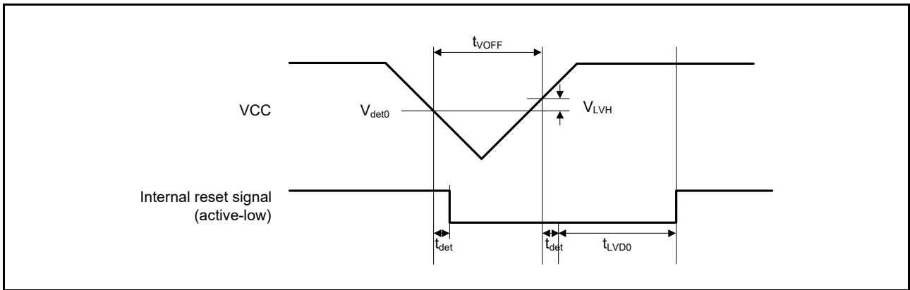
Figure 41.68 Voltage detection circuit timing (V det0 )
