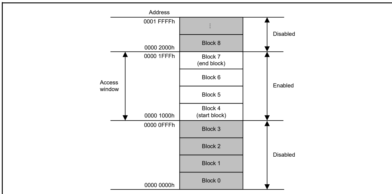
Figure 37.7 Flash area protection overview
