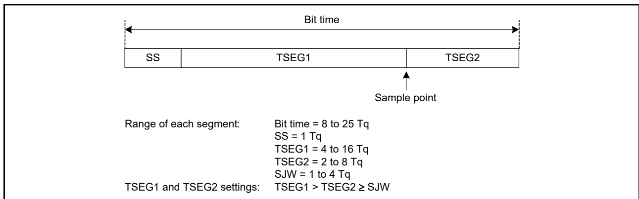
Figure 27.12 Bit timing
