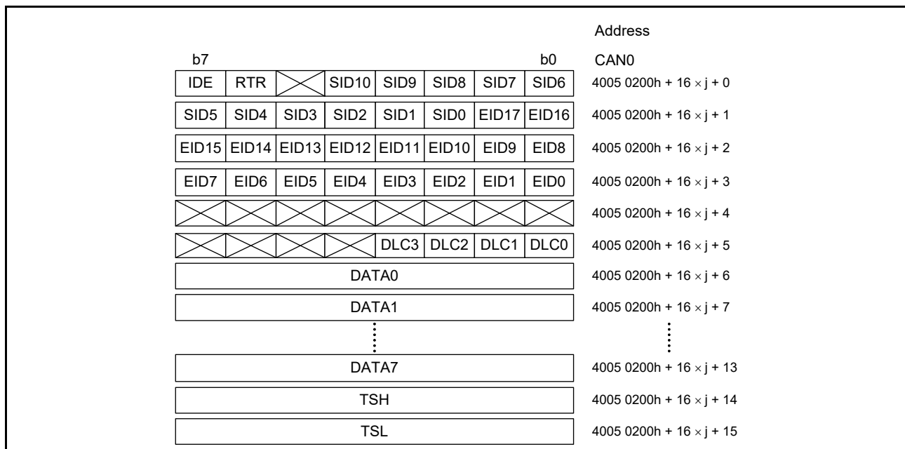
Figure 27.13 Structure of the mailbox registers (j = 0 to 31)
