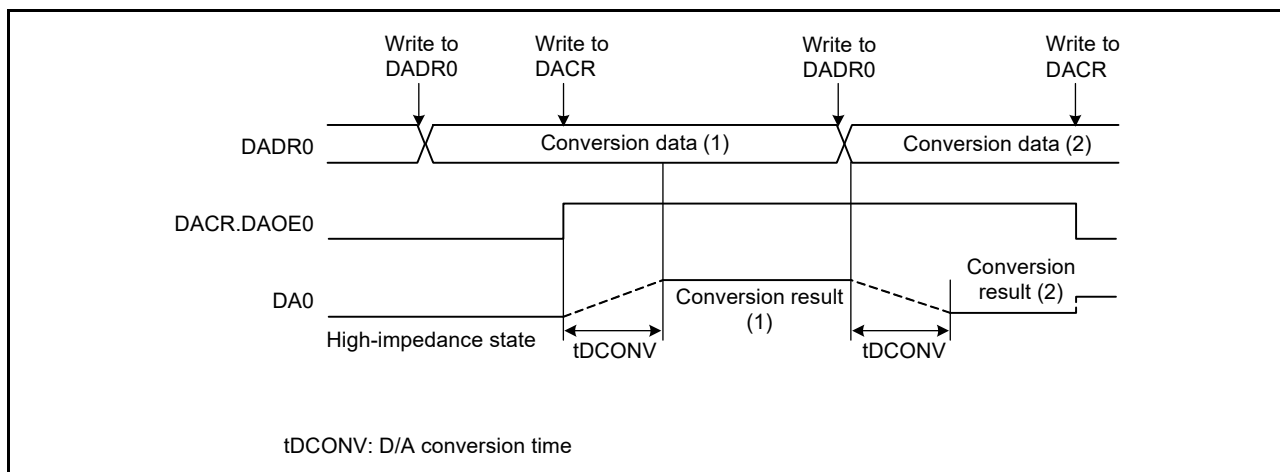
Figure 31.2 Example DAC12 operation
