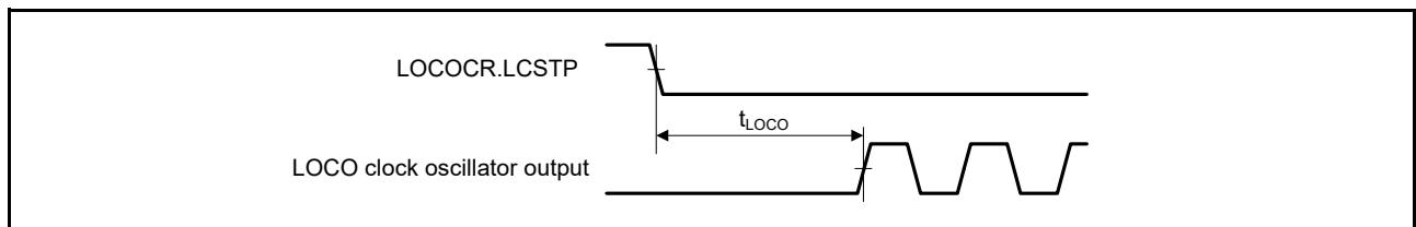
Figure 41.26 LOCO clock oscillator start timing
