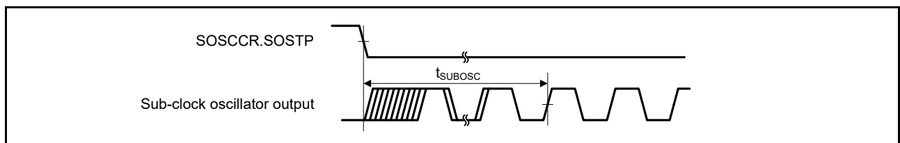
Figure 41.28 Sub-clock oscillator start timing
