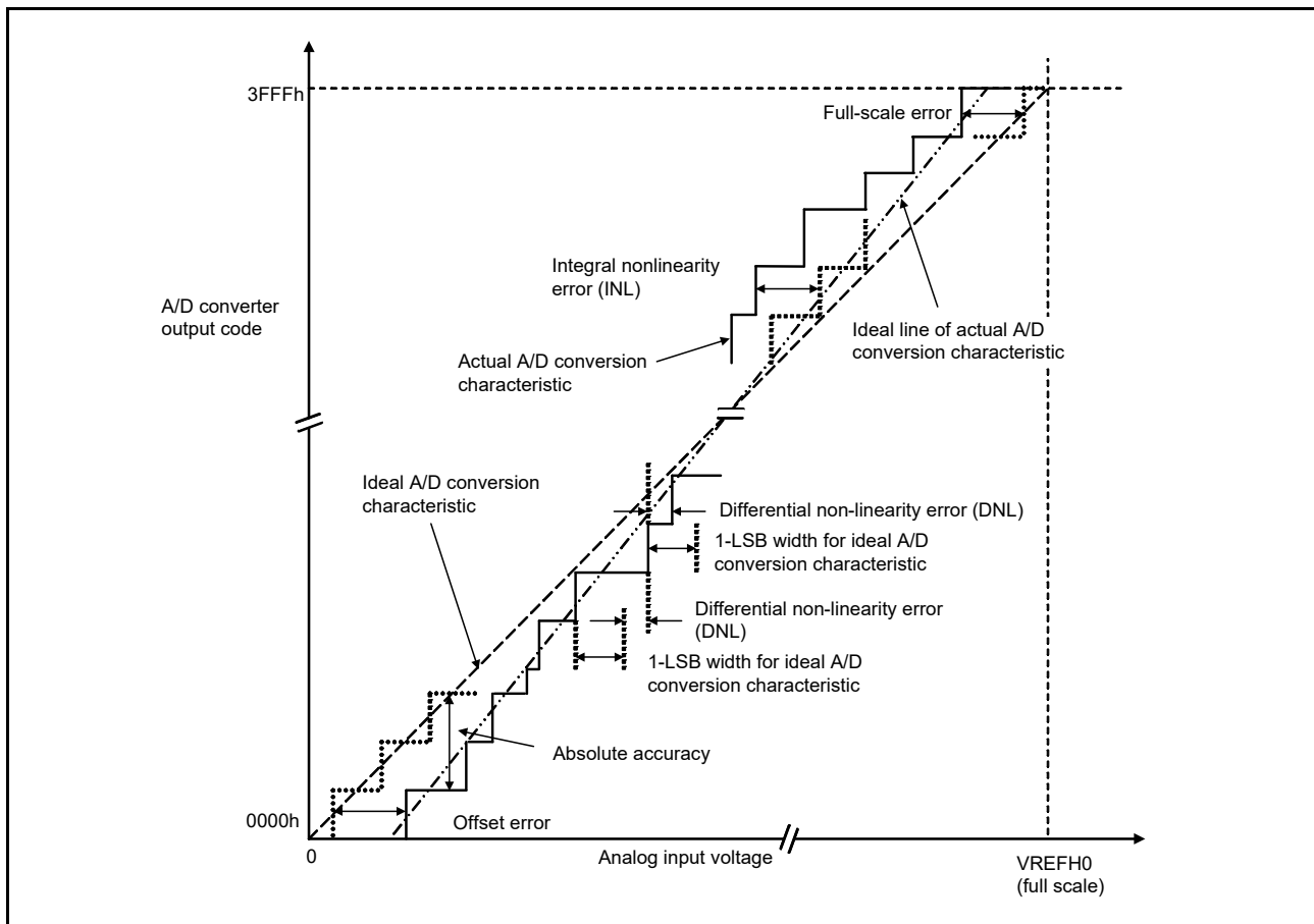
Figure 41.63 Illustration of 14-bit A/D converter characteristic terms
