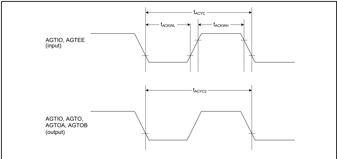
Figure 41.38 AGT I/O timing
