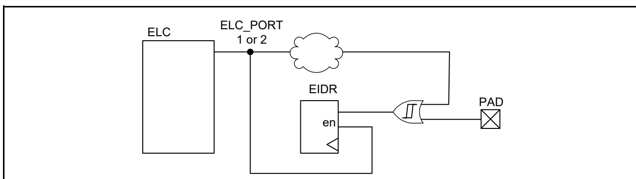
Figure 16.2 Event ports input data
