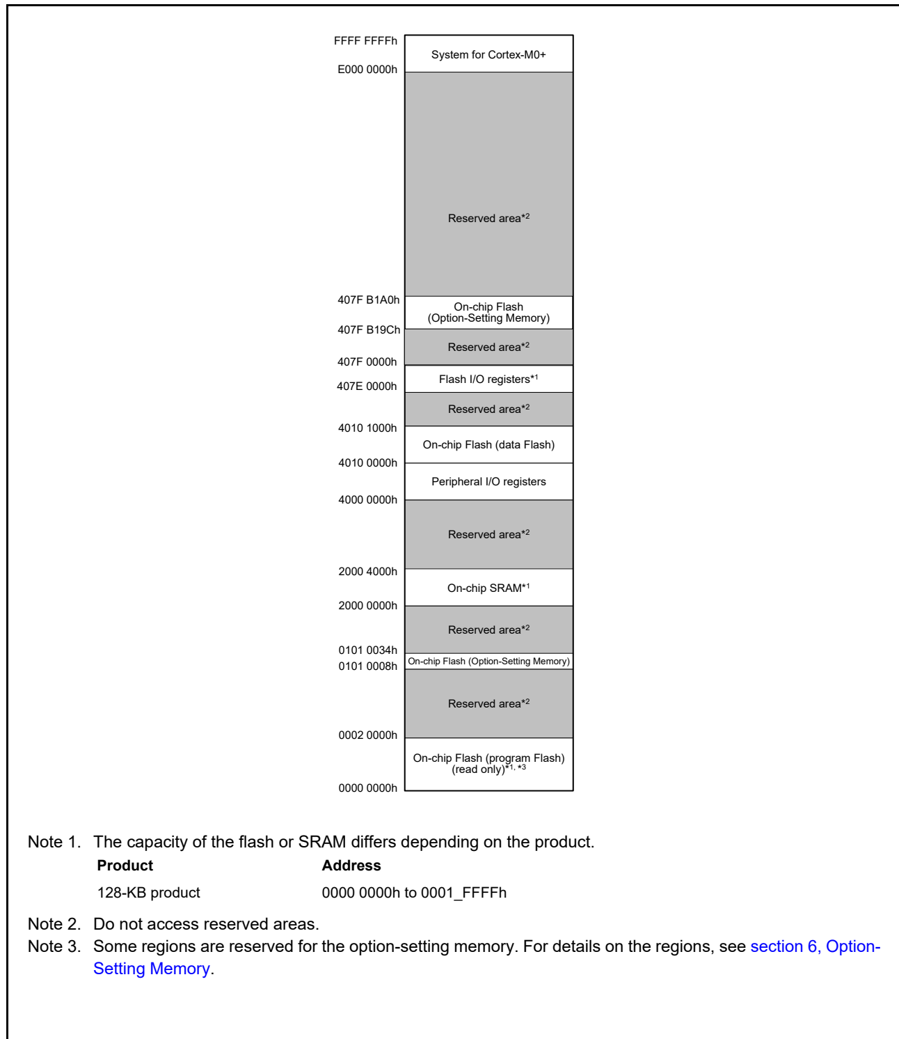
Figure 4.1 Memory map
