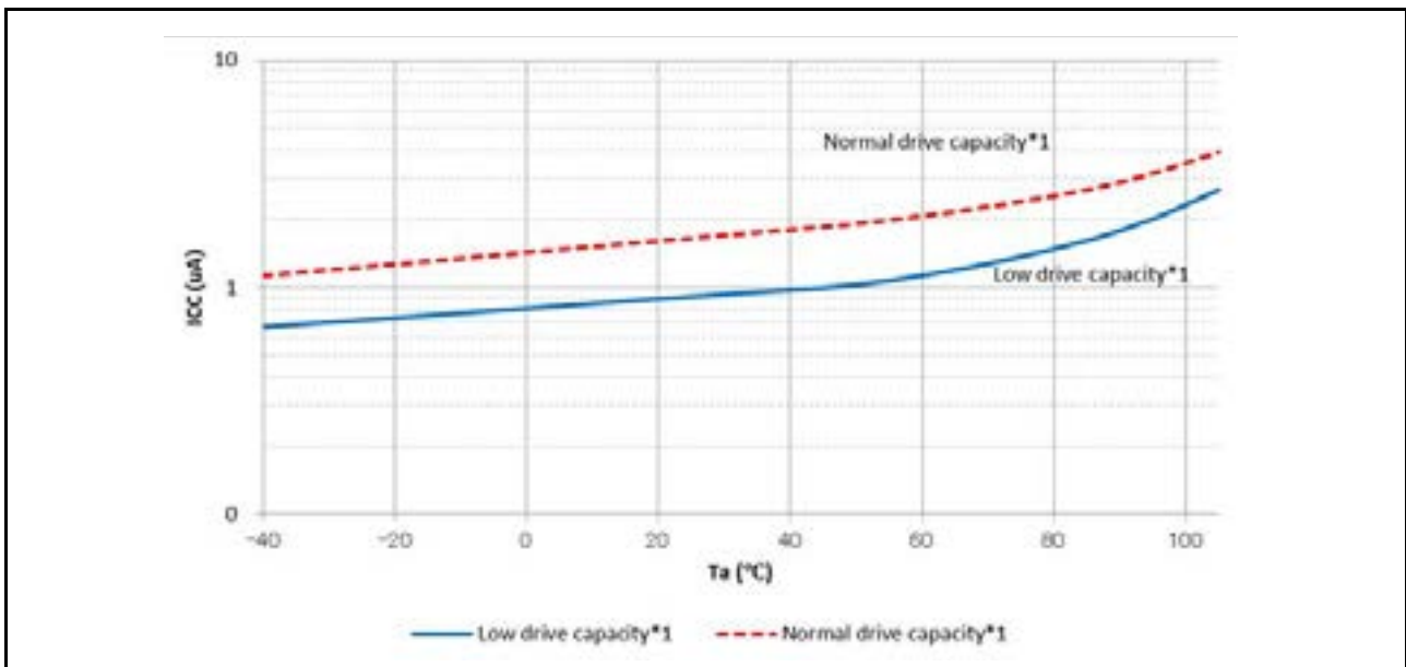
Figure 41.23 Temperature dependency of RTC operation (reference data)
