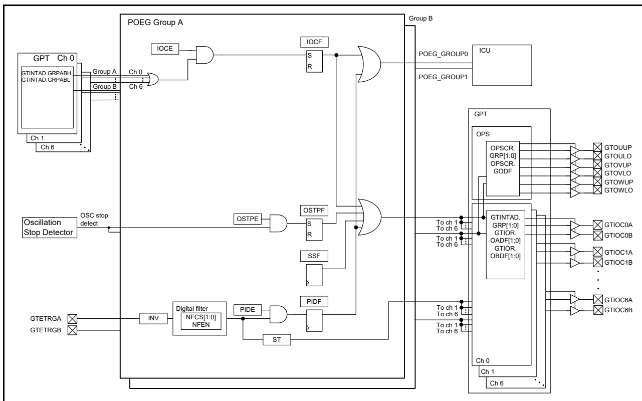
Figure 18.1 POEG block diagram
