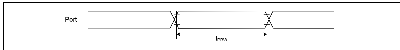
Figure 41.35 I/O ports input timing
