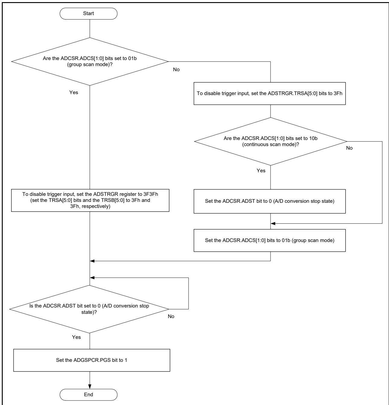
Figure 30.15 Setting flow of ADGSPCR.PGS bit
