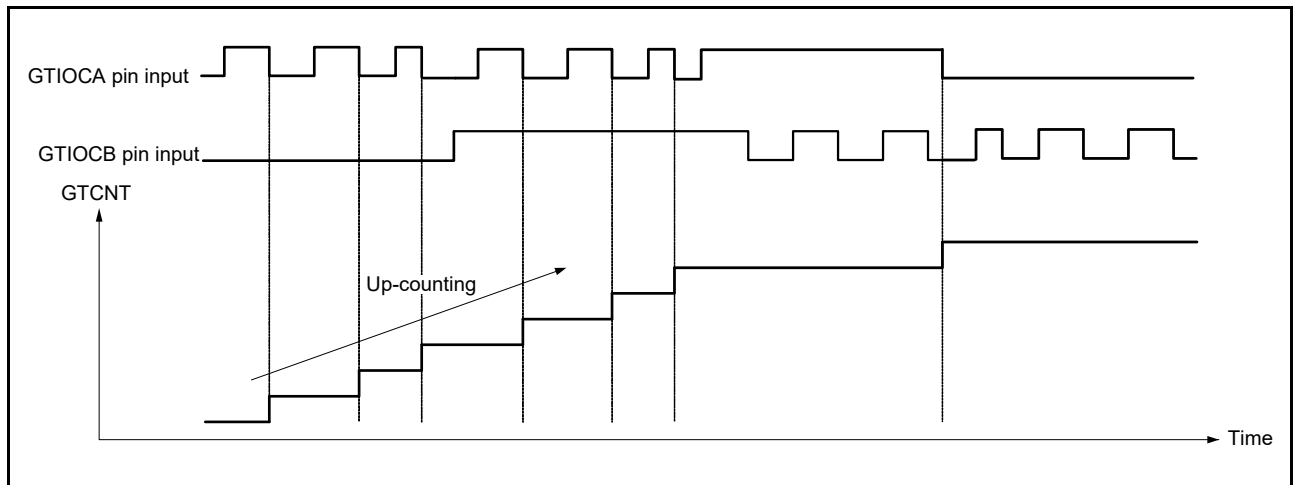
Figure 19.75 Example of phase counting mode 5 (A)
