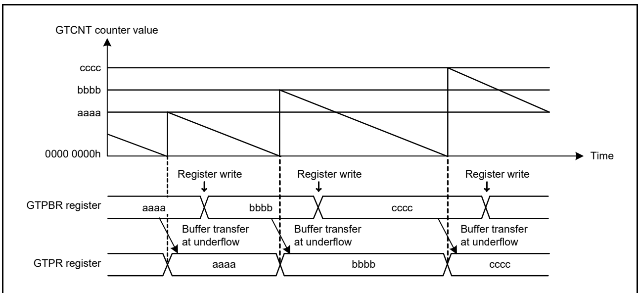
Figure 19.19 Example of GTPR buffer operation (saw waves in down-counting)
