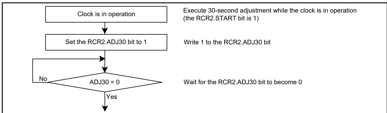
Figure 21.5 30-second adjustment
