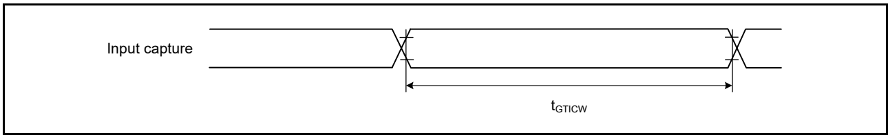
Figure 41.37 GPT input capture timing
