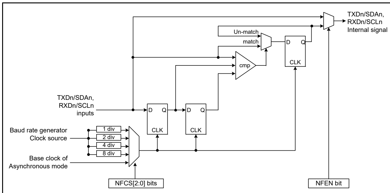
Figure 25.72 Digital noise filter circuit block diagram
