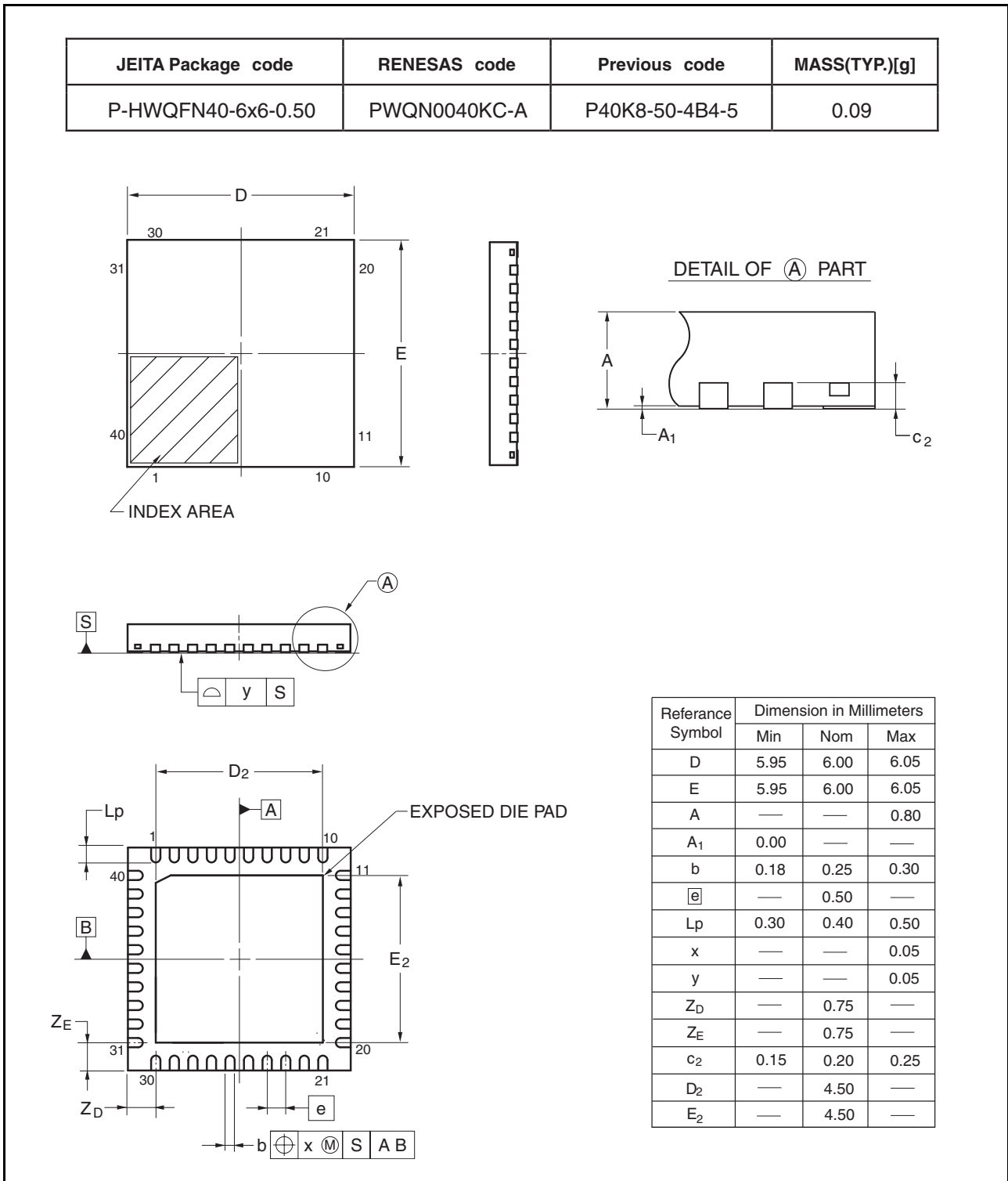
Figure 2.8 QFN 40-pin (1)
