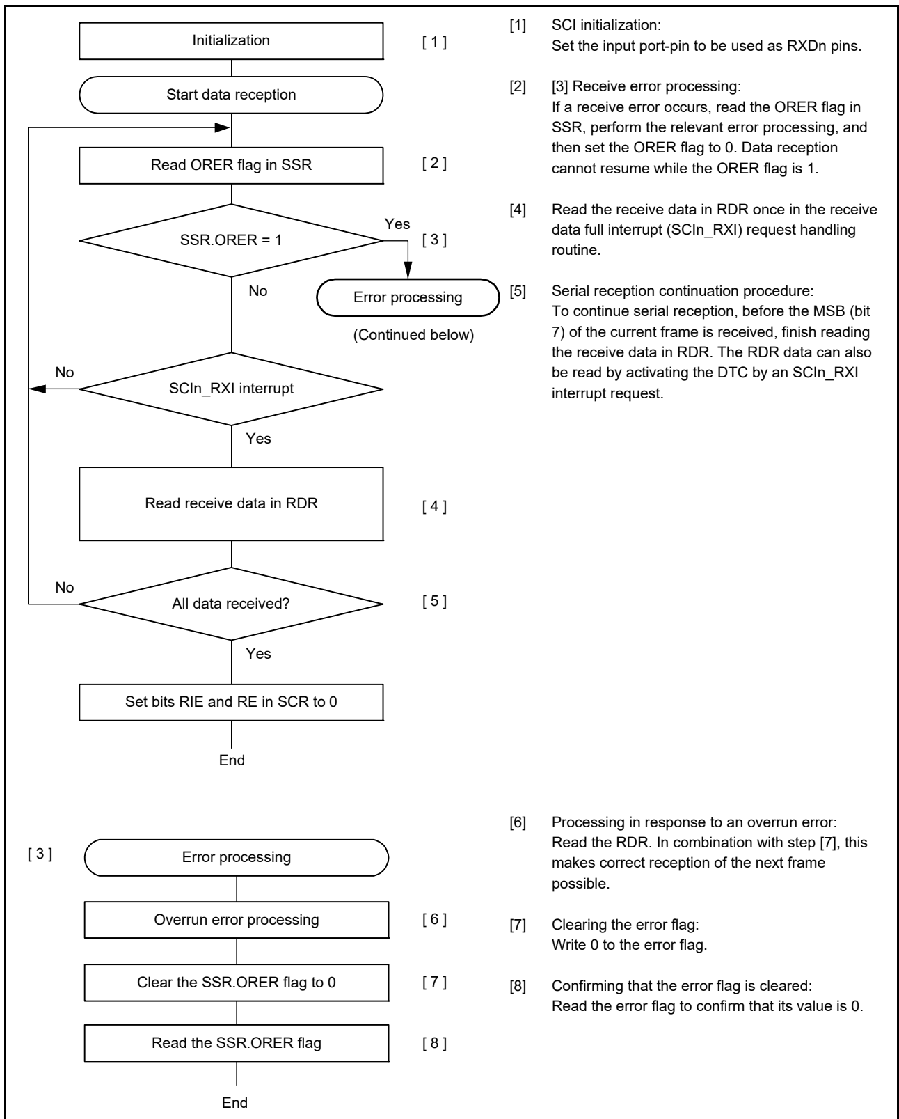
Figure 25.41 Example flow of serial reception in clock synchronous mode with non-FIFO selected
