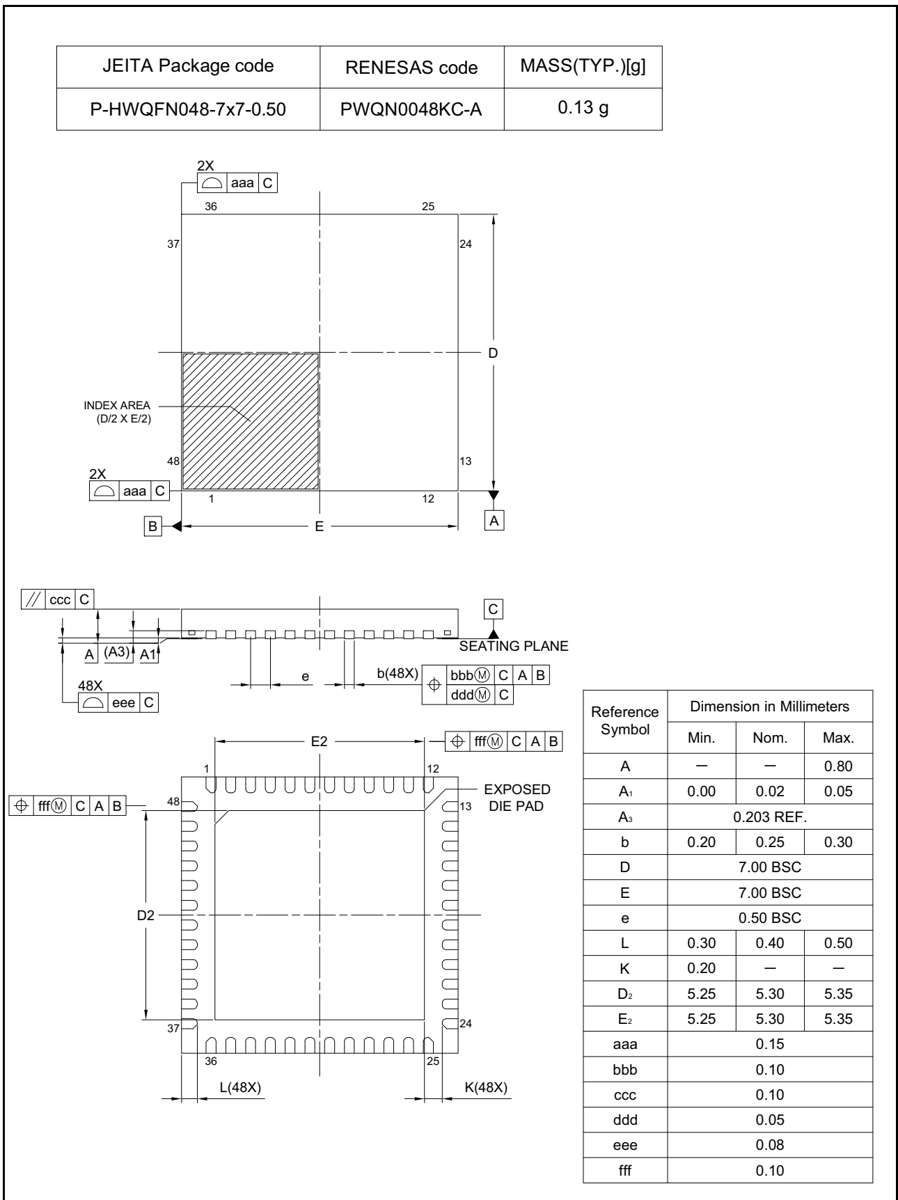
Figure 2.7 QFN 48-pin (2)
