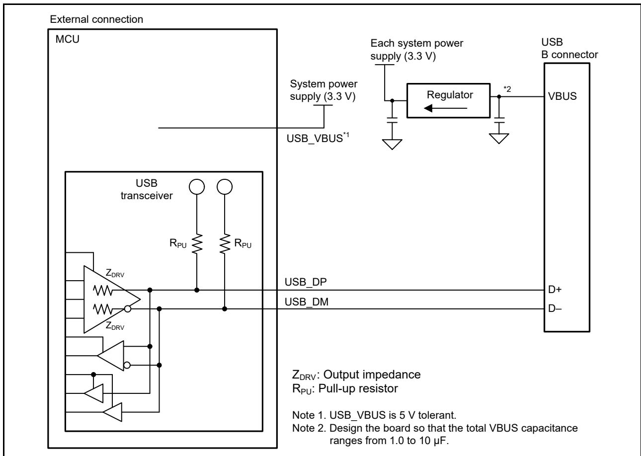
Figure 24.6 Example device connection in bus-powered state 1
