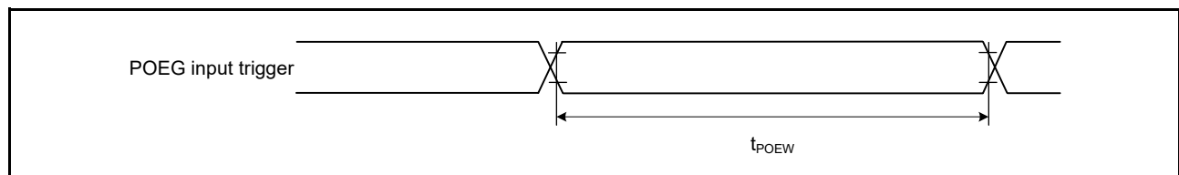
Figure 41.36 POEG input trigger timing
