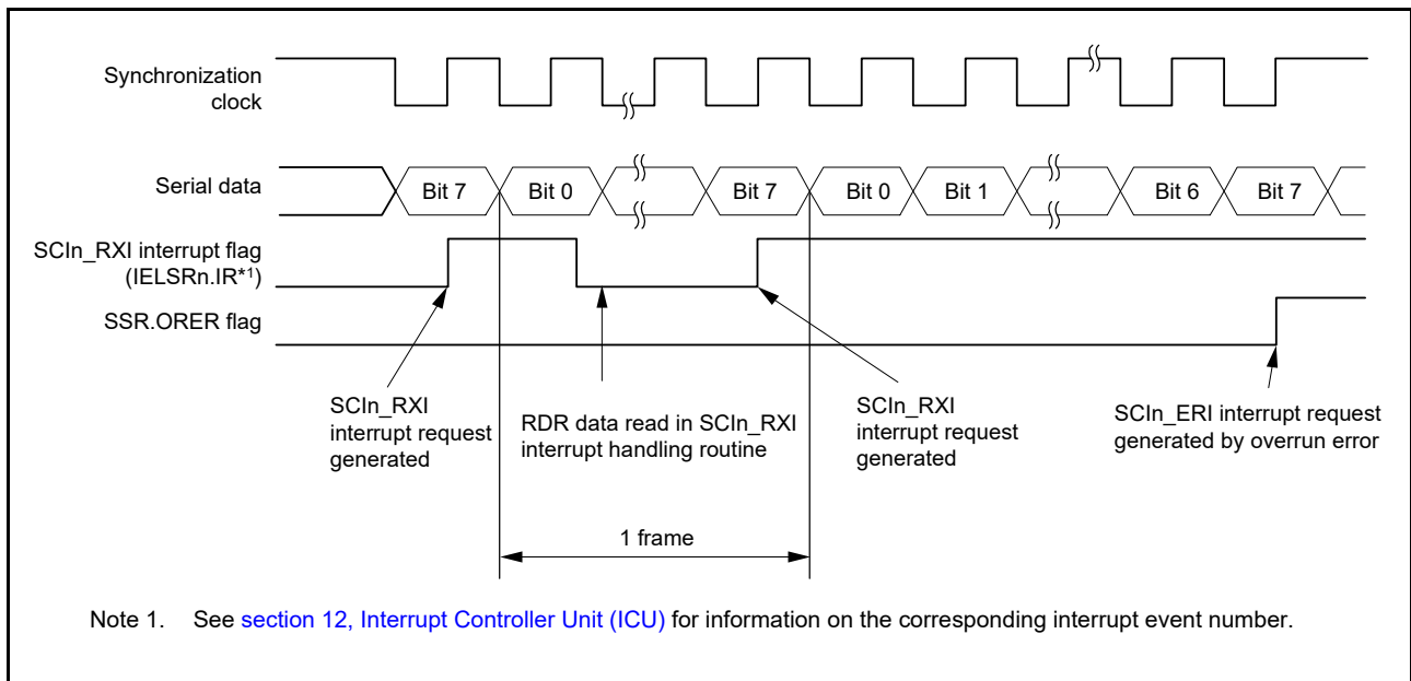
Figure 25.39 Example operation for serial reception in clock synchronous mode (1) when RTS function is not used
