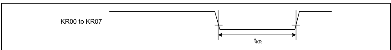
Figure 41.40 Key interrupt input timing
