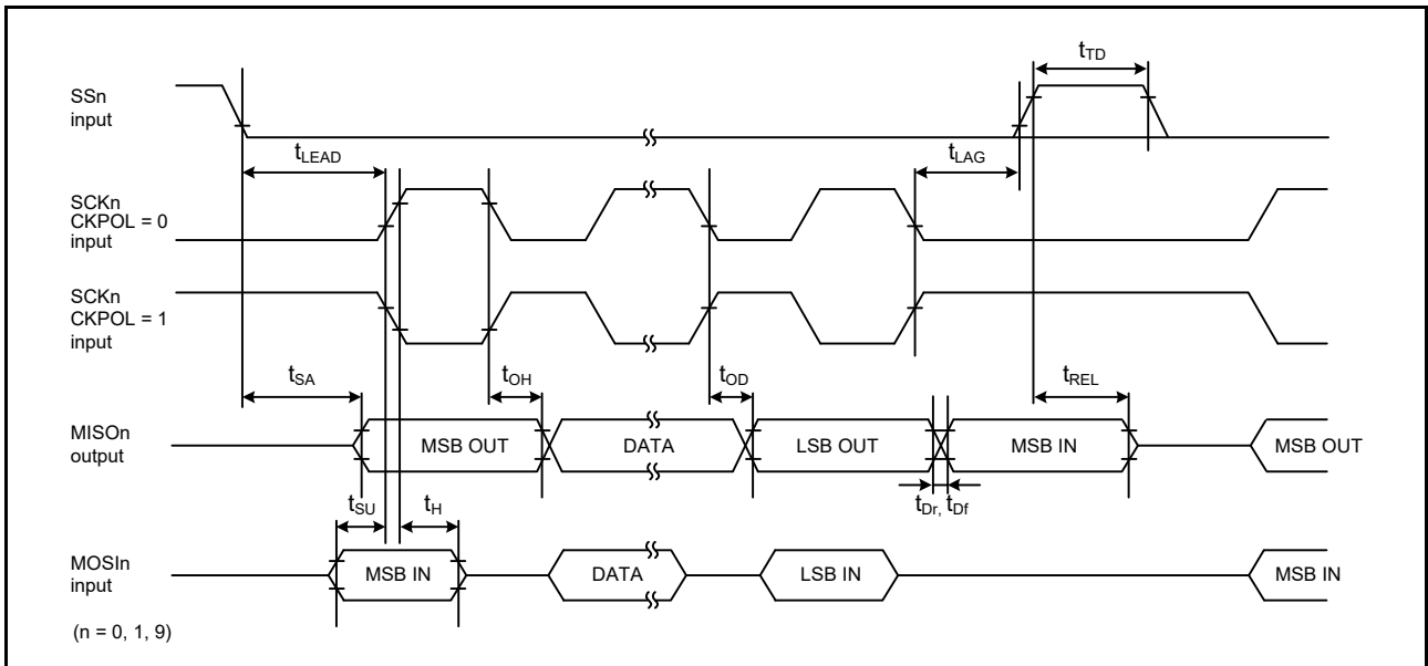
Figure 41.46 SCI simple SPI mode timing (slave, CKPH = 1)
