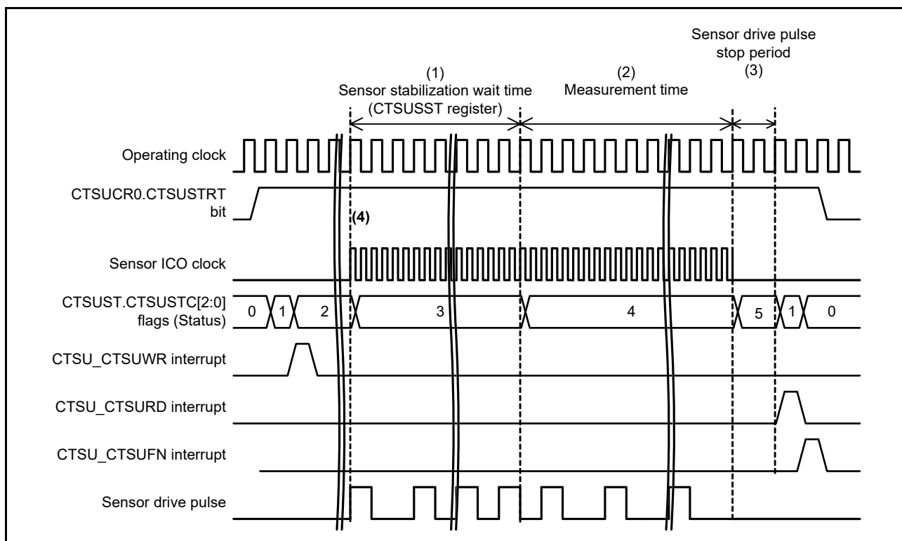
Figure 34.18 Sensor stabilization wait and measurement timing
