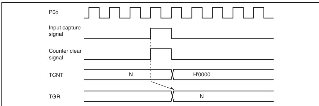
Figure 12.85 Counter Clear Timing (Input Capture)
