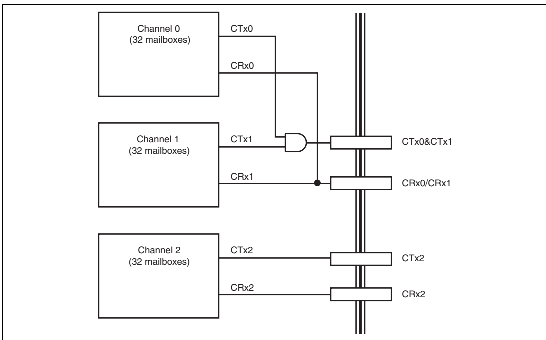
Figure 23.31 Connection Example when Using Channels 0 and 1 as One Channel (64 Mailboxes × 1 Channel) and Channel 2 as One Channel (32 Mailboxes × 1 Channel)
