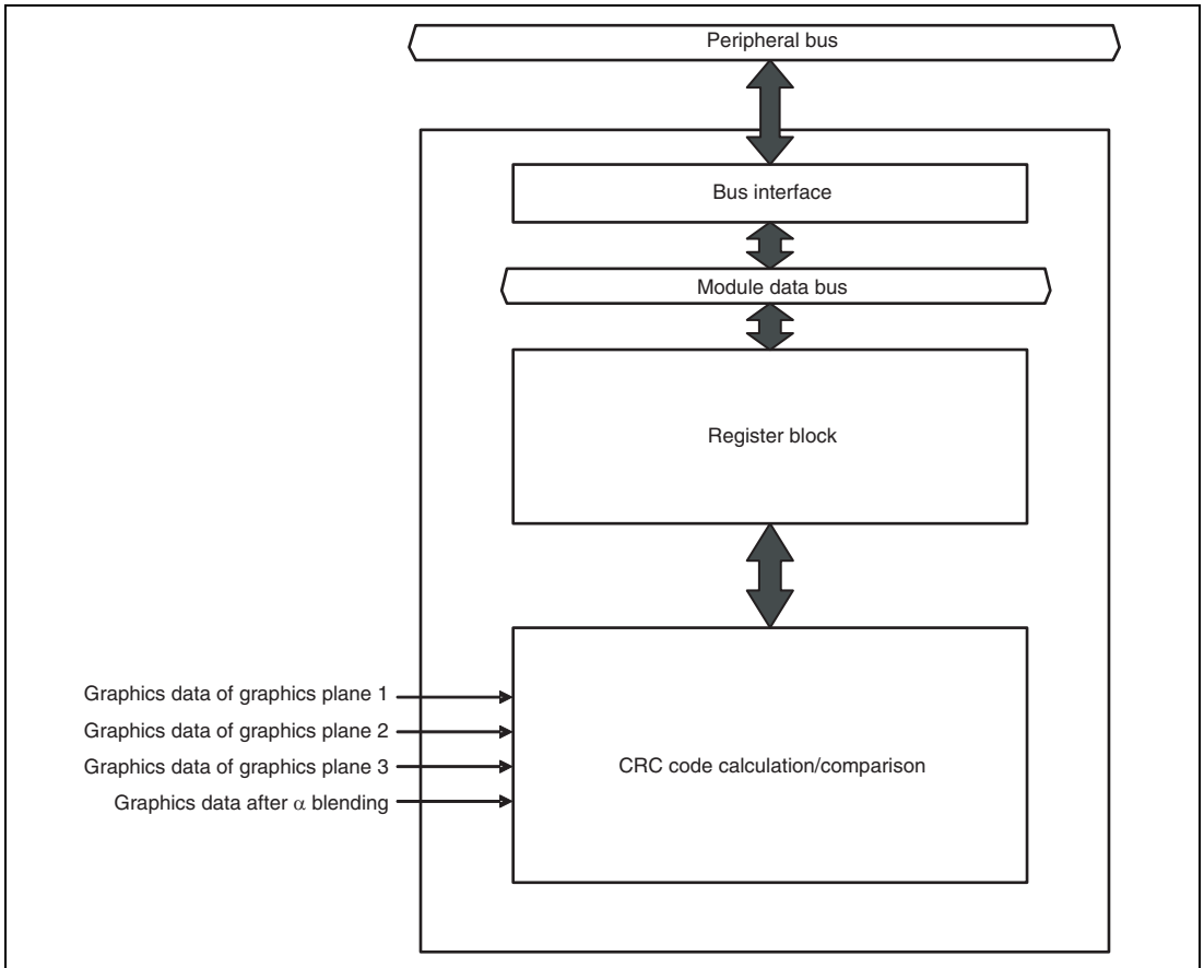
Figure 39.1 Block Diagram
