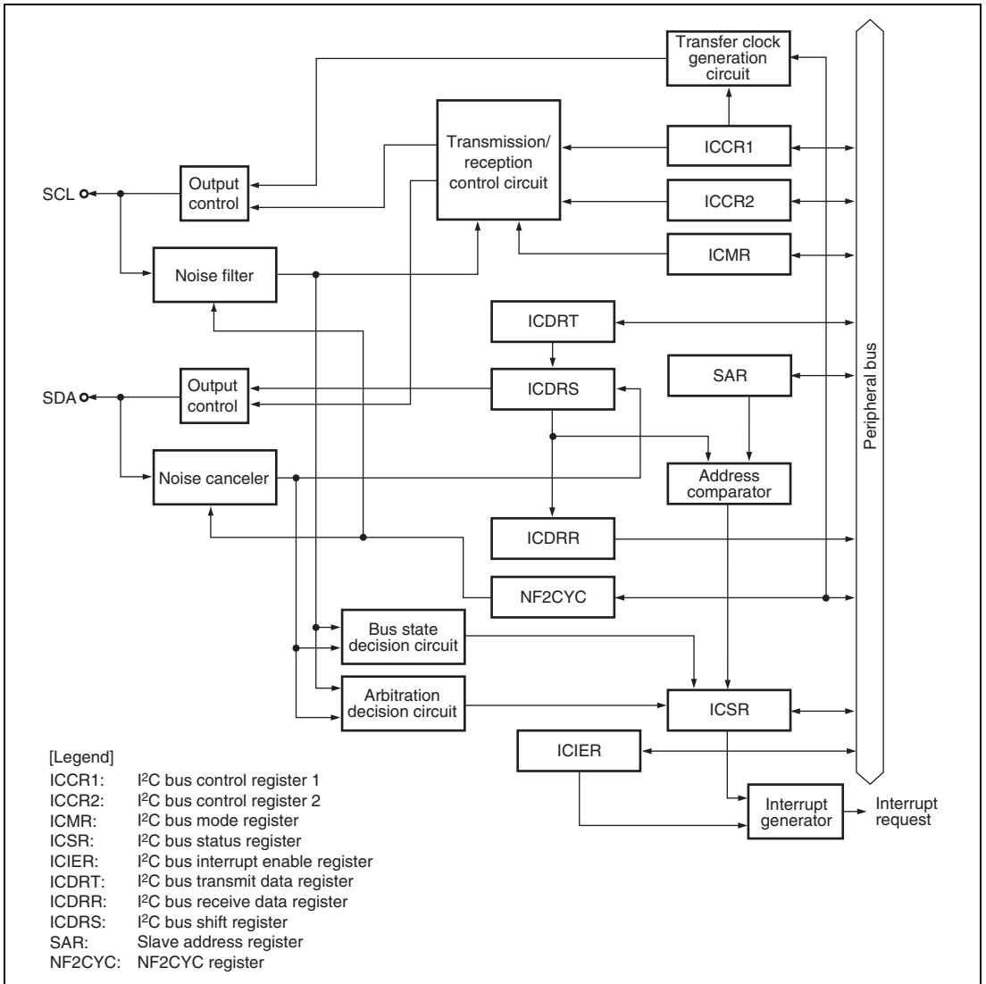
Figure 20.1 Block Diagram
