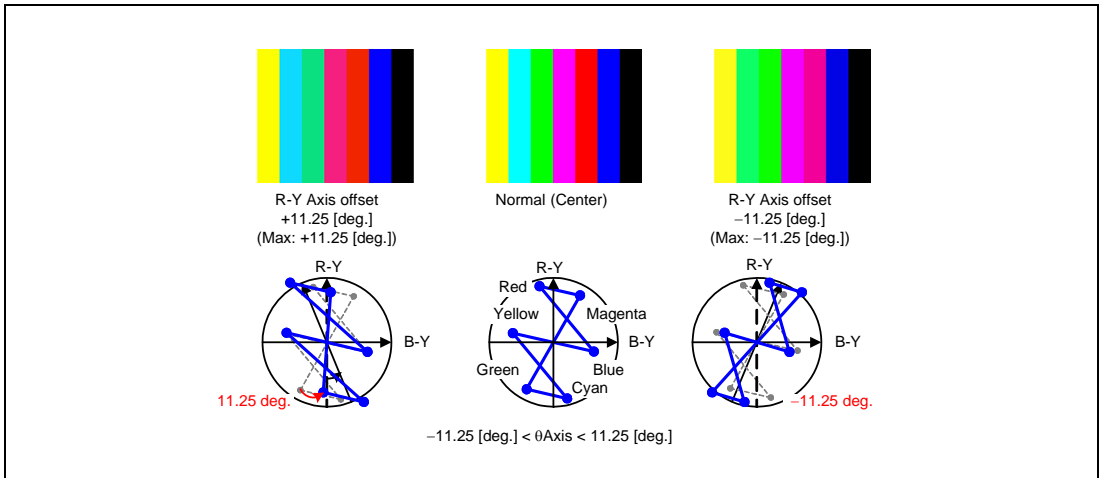
Figure 30.20 Example of R-Y Axis Correction
