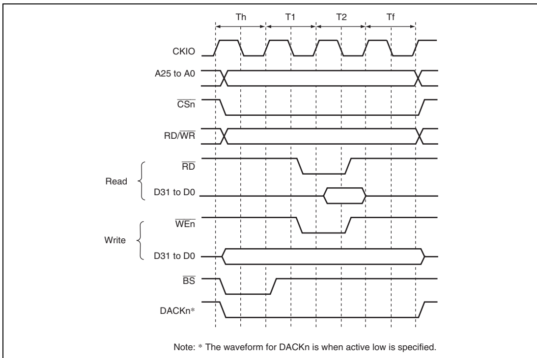
Figure 10.10 \overline{CSn} Assert Period Expansion
