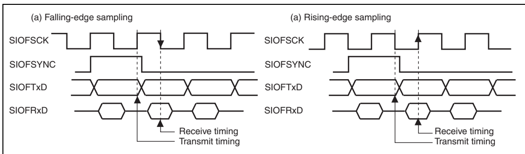
Figure 22.4 Transmit/Receive Timing
