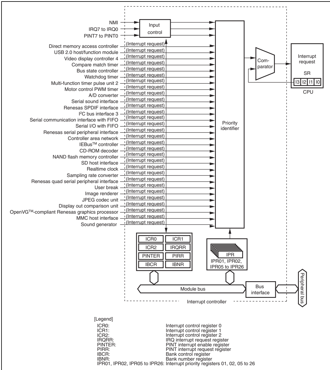
Figure 7.1 Block Diagram
