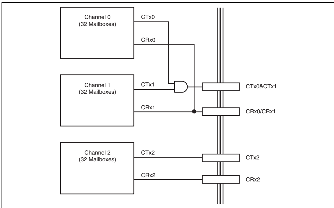
Figure 23.29 Connection Example when Using Channels 0 and 1 as One Channel (64 Mailboxes × 1 Channel) and Channel 2 as One Channel (32 Mailboxes × 1 Channel)
