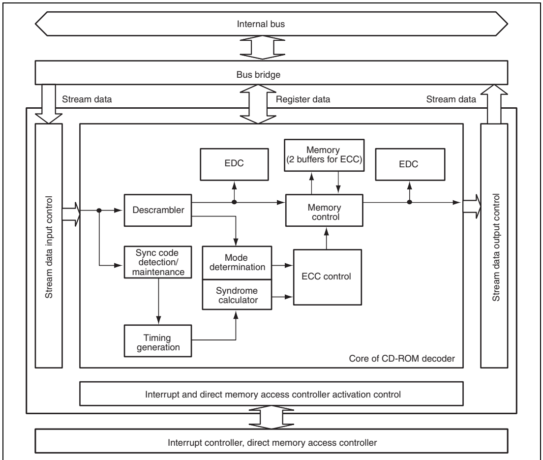
Figure 26.2 Block Diagram
