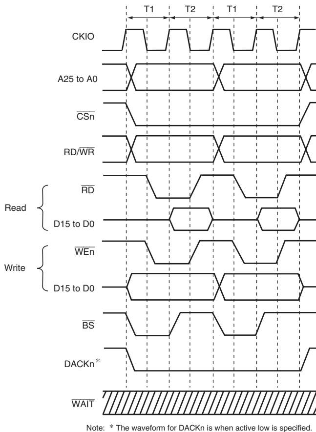
Figure 10.4 Continuous Access to Normal Space (2) Bus Width = 16 Bits, Longword Access, \overline{CSnWCR.WM} Bit = 1 (Access Wait = 0, Cycle Wait = 0)
