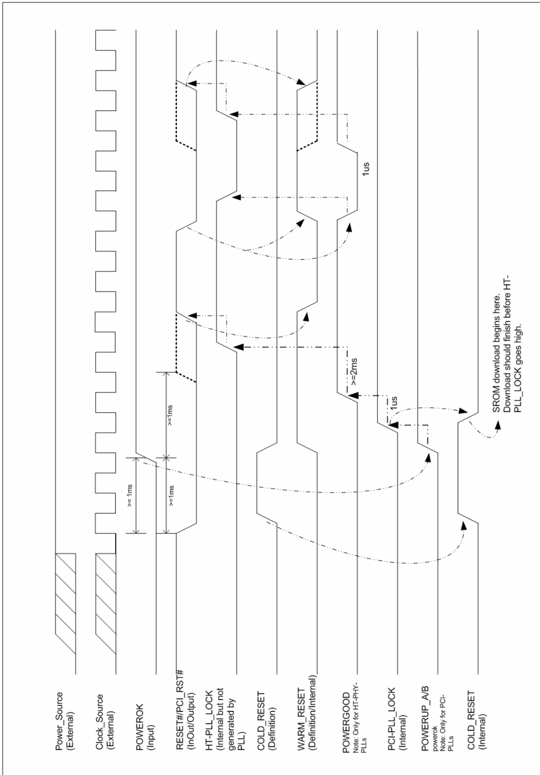
Figure 18: Tsi308 Reset Timing
